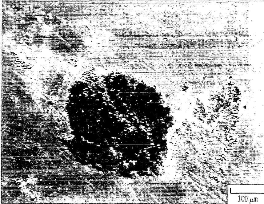
Figure 13. - Photomicrograph of 304 stainless steel rider after running against titanium carbide coated 440C disks. Load, 0.98 newton (100 g).
