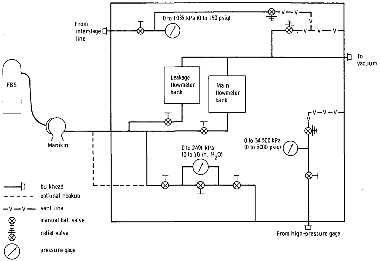
Figure D-3.- Type I FBS test stand.
