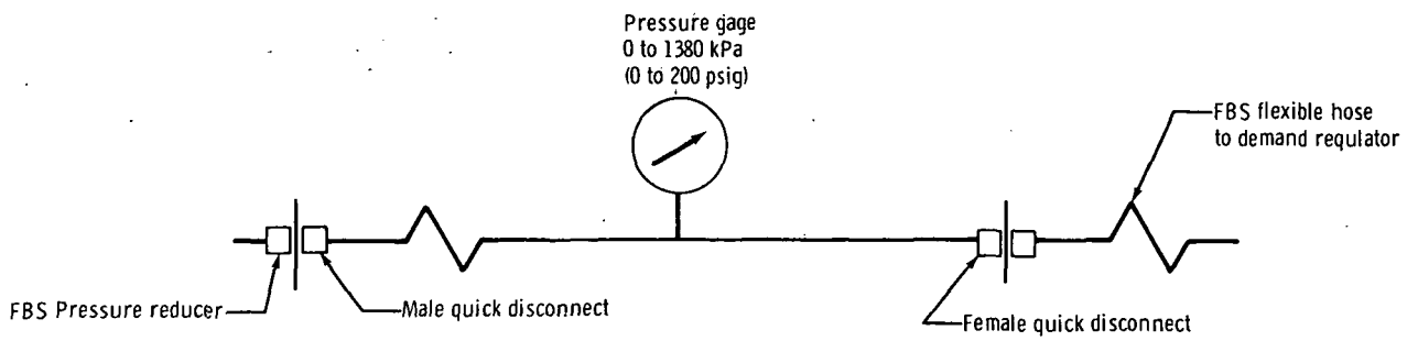
INTERSTAGE PRESSURE VERIFICATION SECTION
