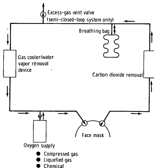
Figure 3.- Closed- and semi-closed-loop system schematic.
