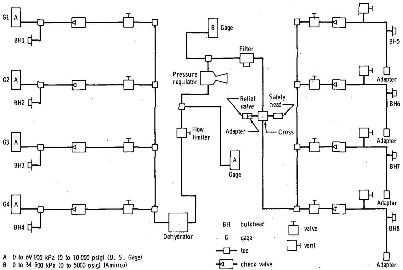
Figure D-1.- Cascade charging station schematic.
