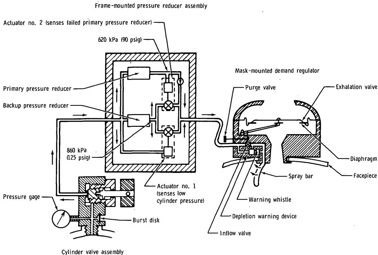
Figure 7.- NASA FBS schematic.
