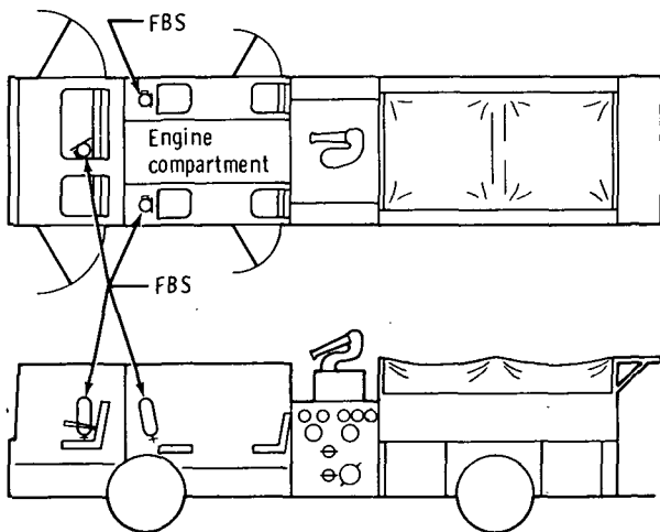
Figure C-3.- New York firetruck layout, Squad Company 4.
