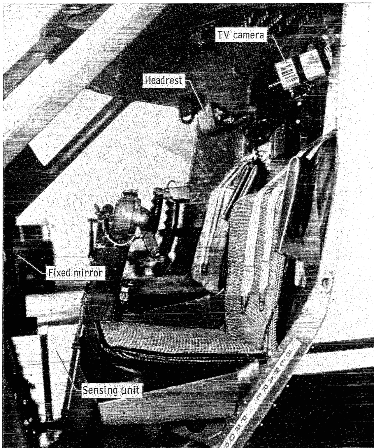
Figure 10.- Cockpit equipment added for oculometer flight tests.
