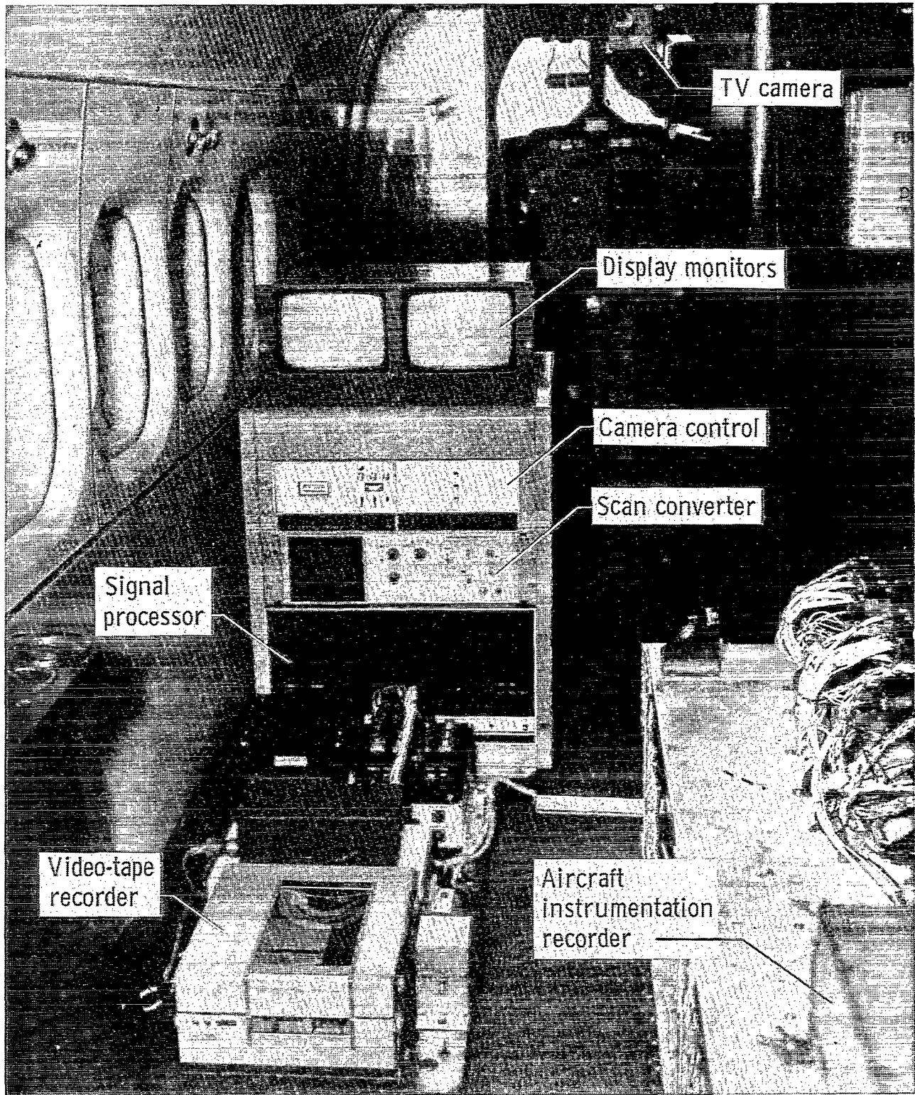
Figure 12.- Oculometer components located in passenger compartment.
