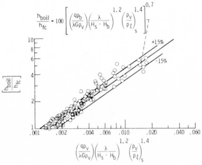
Figure 5. - Liquid neon convective boiling data correlation. Pressure = 1.12 to 1.66 MP a (11.2 to 16.6 bars); flow rate = 4.0 to 10.8 g/sec; heat flux = 1.8 to 20.5 W/cm 2 ; subcooling = 1.5 to 11.6 K.
