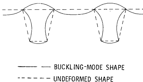
Figure 2.- Continuous buckle pattern.
