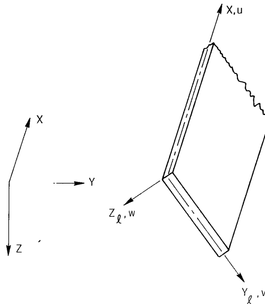
Figure 17.- Local coordinate system for panel element and overall coordinate system for stiffened panel.
