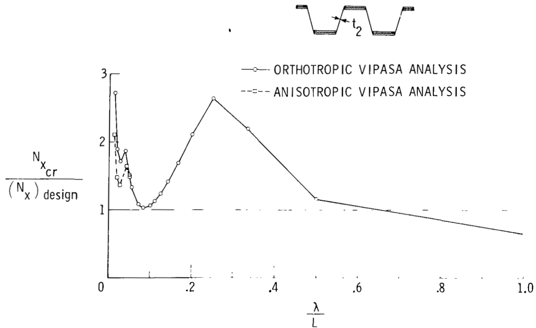
Figure 24.- Ratio of buckling load to design load as a function of buckling half-wavelength for a corrugated panel designed using the procedure of reference 11 for a loading of N_x/L = 1380 \text{ kPa} ( 200 \text{ lbf/in}^2 ); t_2 = 0.56 \text{ mm} ( 0.022 \text{ in.} ).
