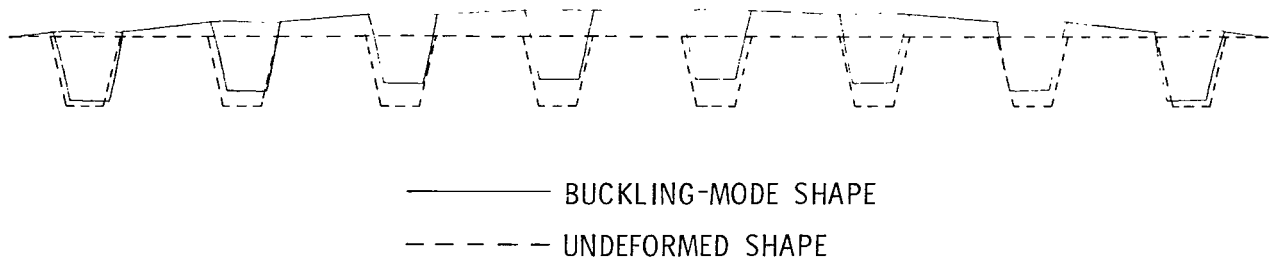
Figure 6.- Overall-buckling-mode shape for panel whose buckling response diagram is shown in figure 5. \lambda = L .
