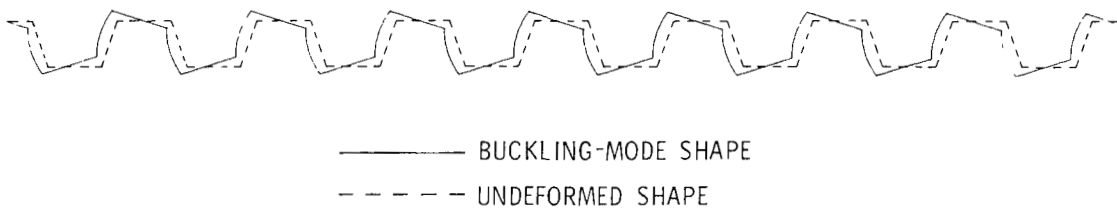
Figure 25.- Buckling-mode shape for panel whose buckling response diagram is shown in figure 24.
