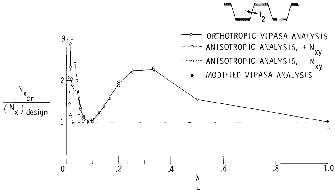
Figure 26.- Ratio of buckling load to design load as a function of buckling half-wavelength for a corrugated panel designed using the procedure of reference 11 for a loading of N_x/L = 689 \text{ kPa} ( 100 \text{ lbf/in}^2 ); N_{xy}/N_x = 0.1 ; t_2 = 0.56 \text{ mm} ( 0.022 \text{ in.} ).
