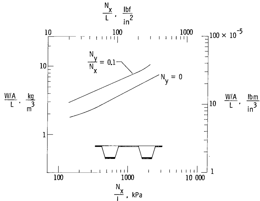
Figure 13.- Structural efficiency of graphite-epoxy, hat-stiffened panels designed for pure longitudinal compression and for longitudinal and transverse compression.
