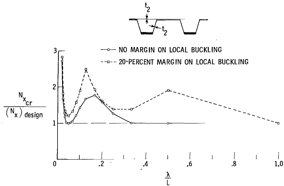
Figure 14.- Ratio of buckling load to design load as a function of buckling half-wavelength for two hat-stiffened panels designed for N_x/L = 5520 \text{ kPa} ( 800 \text{ lbf/in}^2 ); t_2 = 1.12 \text{ mm} ( 0.044 \text{ in.} ).
