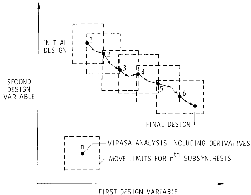
Figure 4.- Synthesis strategy including move limits during subsynthesis in two-design-variable space.
