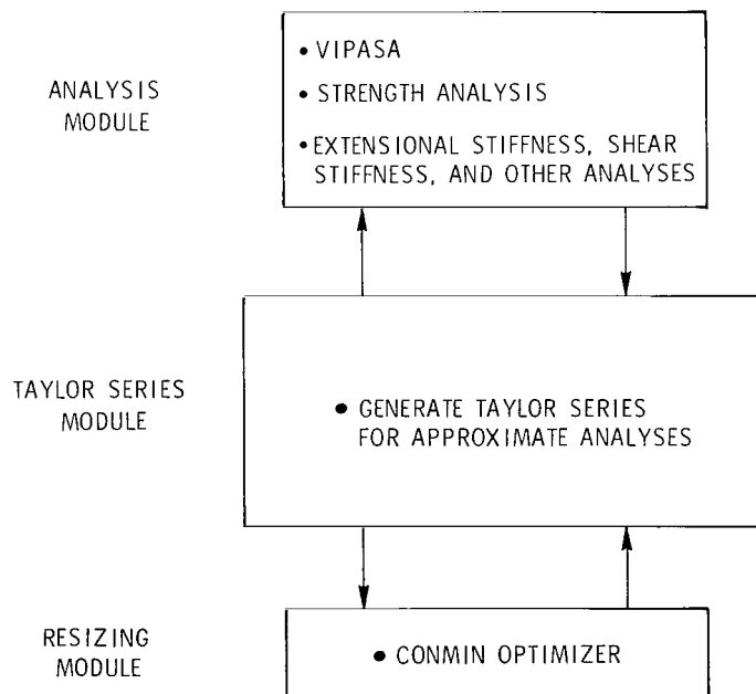
Figure 3.- General approach used in present procedure.
