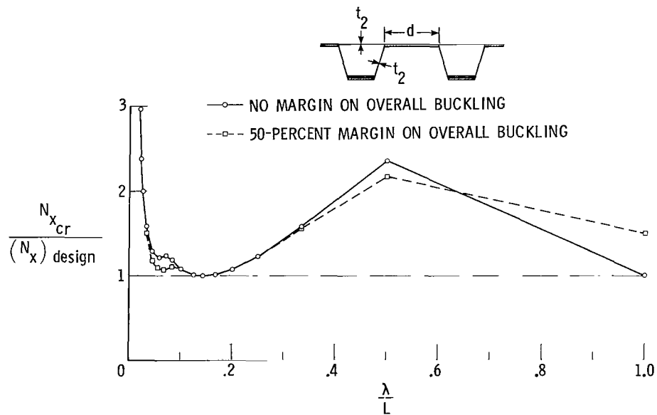
Figure 15.- Ratio of buckling load to design load as a function of buckling half-wavelength for two hat-stiffened panels designed for N_x/L = 689 \text{ kPa} ( 100 \text{ lbf/in}^2 ); d = 12.7 \text{ cm} ( 5.0 \text{ in.} ).
