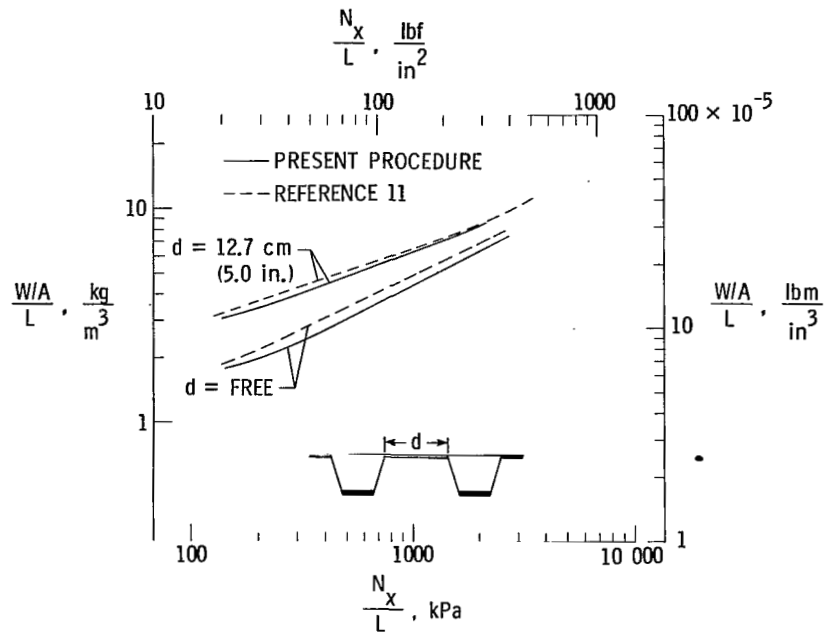
Figure 11.- Structural efficiency of graphite-epoxy, hat-stiffened panels designed for longitudinal compression; with and without constraint on distance d between stiffeners.
