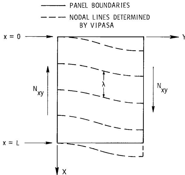
Figure 20.- Nodal lines determined by VIPASA in the case of a shear loading and/or anisotropy.
