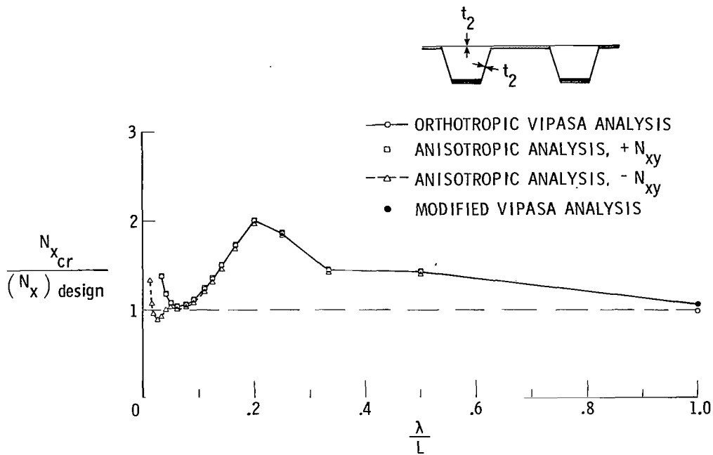
Figure 22.- Ratio of buckling load to design load as a function of buckling half-wavelength for a hat-stiffened panel designed using the procedure of reference 11 for a loading of N_x/L = 689 \text{ kPa} ( 100 \text{ lbf/in}^2 ); N_{xy}/N_x = 0.1 ; t_2 = 0.56 \text{ mm} ( 0.022 \text{ in.} ).
