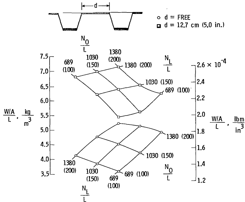
Figure 16.- Mass index as a function of required local buckling load N_L/L and required overall buckling load N_O/L for graphite-epoxy, hat-stiffened panels with and without design requirements on distance d between stiffeners. Required buckling loads given in kPa (lbf/in 2 ).
