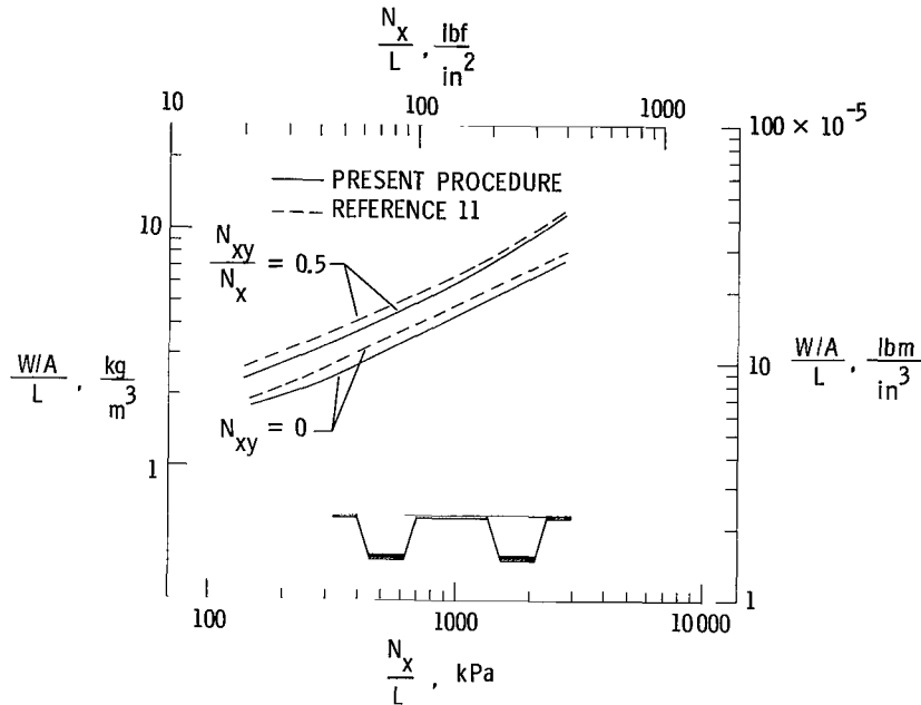
Figure 9.- Structural efficiency of graphite-epoxy, hat-stiffened panels designed for pure longitudinal compression and for longitudinal compression and shear.
