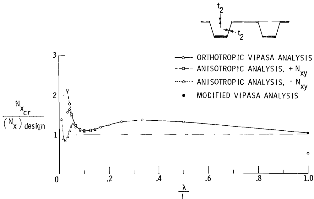
Figure 23.- Ratio of buckling load to design load as a function of buckling half-wavelength for a hat-stiffened panel designed using the procedure of reference 11 for a loading of N_x/L = 207 \text{ kPa} ( 30 \text{ lbf/in}^2 ); N_{xy}/N_x = 1.0 ; t_2 = 0.56 \text{ mm} ( 0.022 \text{ in.} ).
