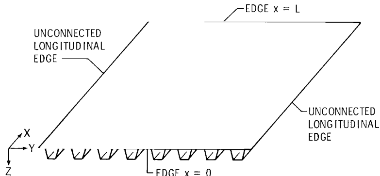
Figure 18.- Eight-stiffener mathematical model of hat-stiffened panel.
