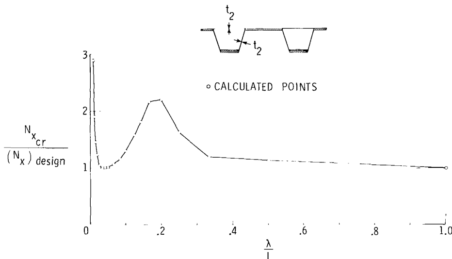
Figure 5.- Ratio of buckling load to design load as a function of buckling half-wavelength for a hat-stiffened panel designed for a loading of N_x/L = 689 \text{ kPa} ( 100 \text{ lbf/in}^2 ); t_2 = 0.56 \text{ mm} ( 0.022 \text{ in.} ).
