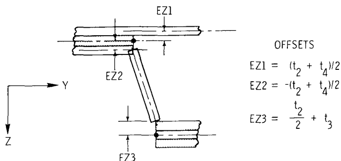
(b) Mathematical model used in VIPASA.
