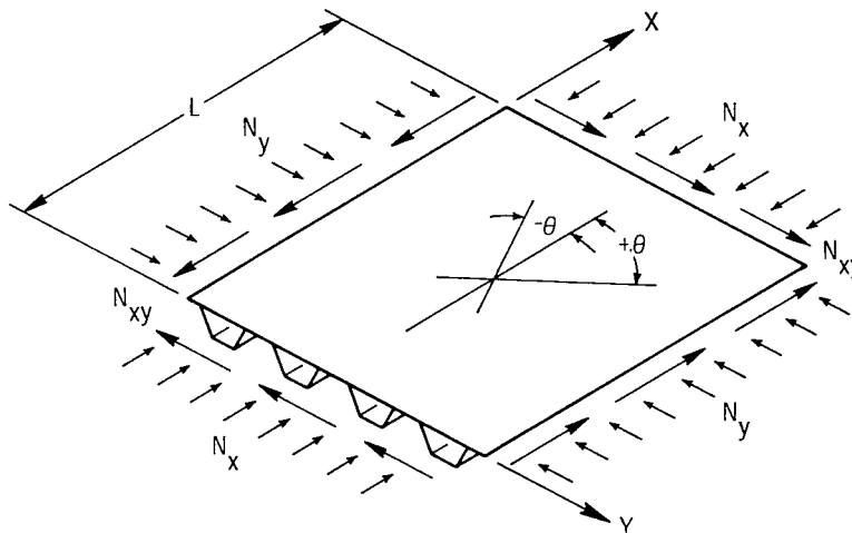
Figure 1.- Loadings considered.
