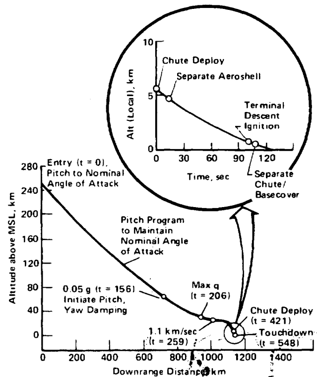
Figure II-2 Lander Entry Sequence
