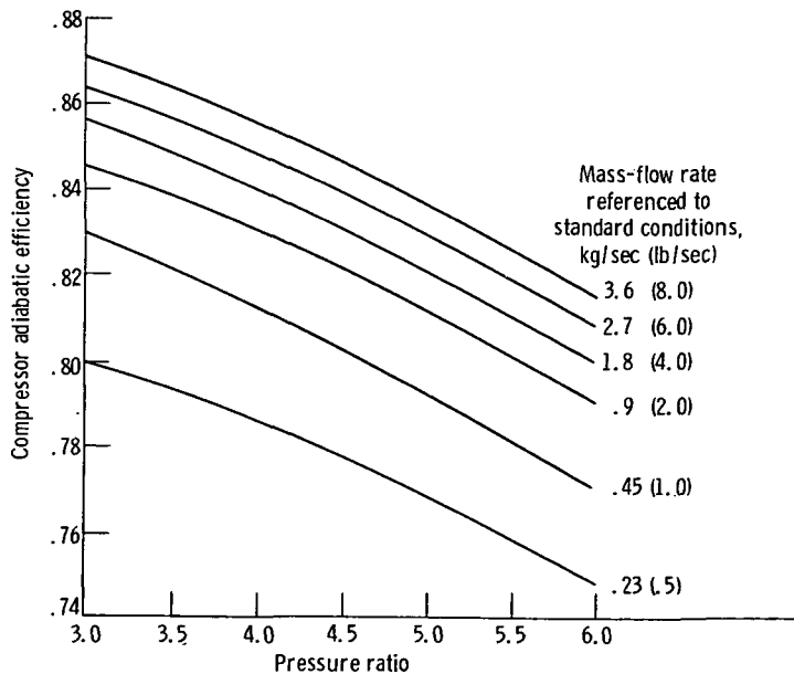
Figure 3. - Variation of compressor efficiency with design pressure ratio and mass-flow rate. Compressor specific speed, 0.775.
