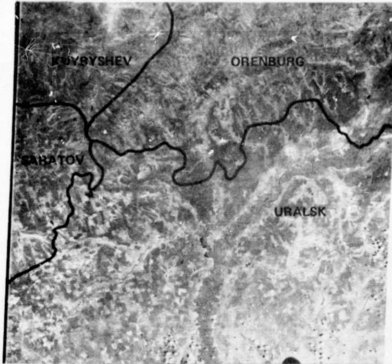
Figure 3. Saratov, U.S.S.R., region under normal moisture conditions. Full-frame Landsat image, 17 June 1976.
