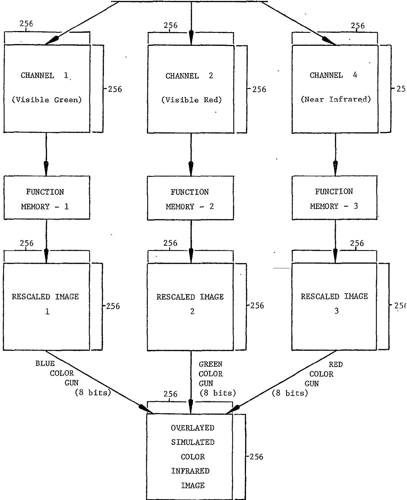
Figure A-5. Block diagram of Mode 2 of the Color Video Display
