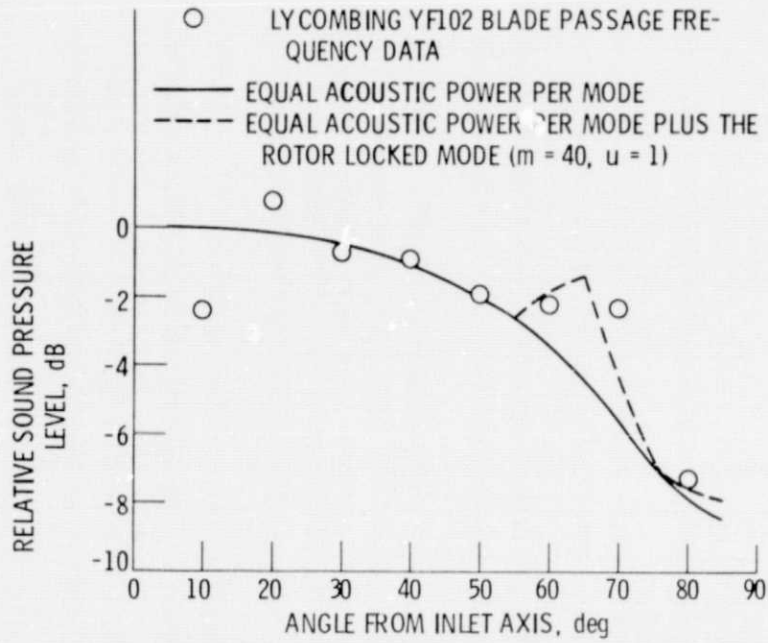
Figure 9. - Comparison of experimental data with calculated multimodal directivity pattern.
