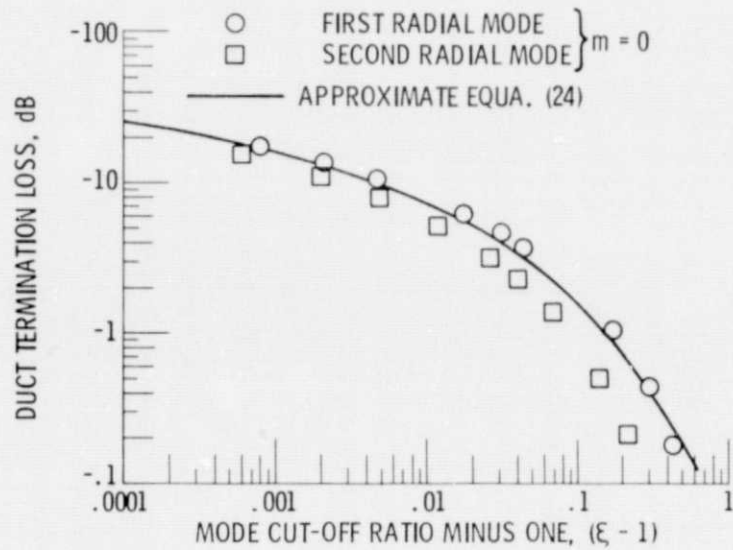
Figure 5. - Modal transmission loss at duct termination.
