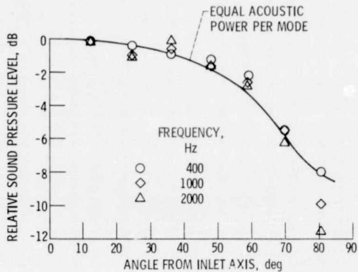
Figure 7. - Comparison of equal power per mode multimodal directivity to experimental data from NASA Fan B (ref. 14).
