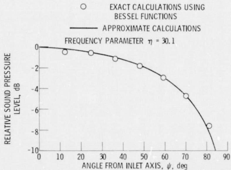
Figure 2. - Comparison of exact and approximate multi-modal far-field directivity patterns for equal acoustic power per mode.
