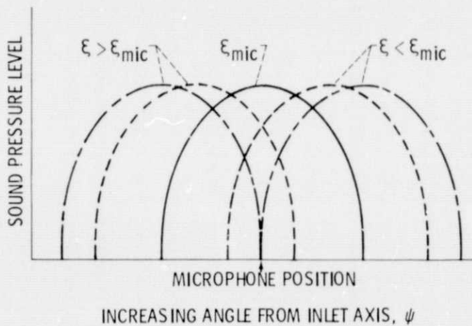
Figure 1. - Schematic of modal principle lobes of radiation contributing to a far-field microphone signal.
