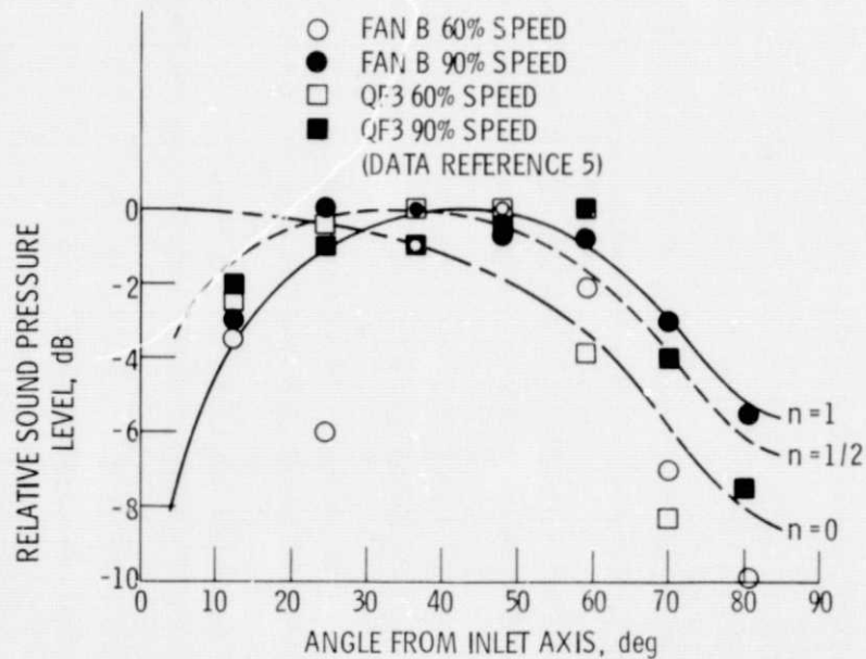
Figure 8. - Comparison of fan blade passage frequency data with calculated far-field multimodal directivity patterns.
