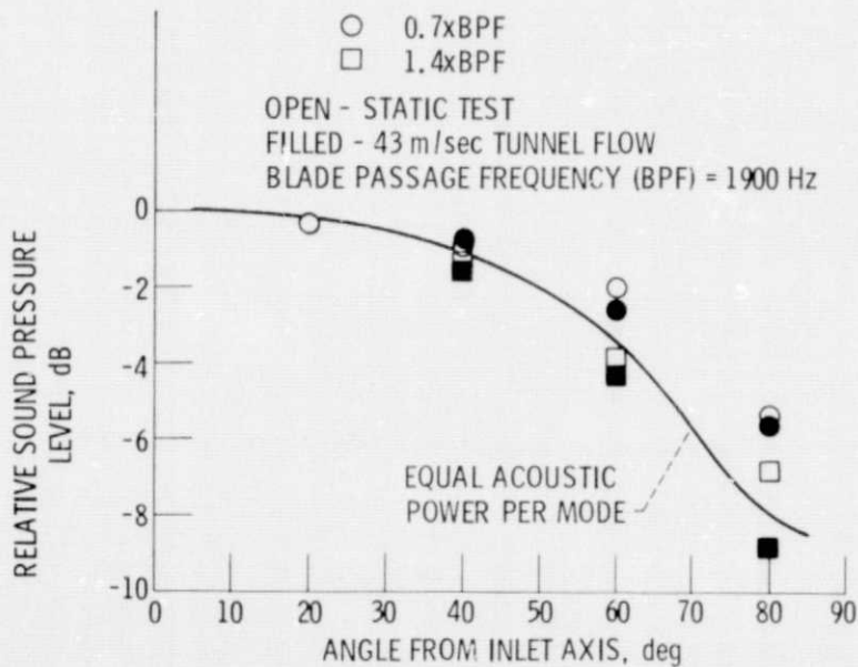
Figure 6. - Comparison of multimodal equal power per mode directivity to experimental data obtained in a wind tunnel (ref. 13).
