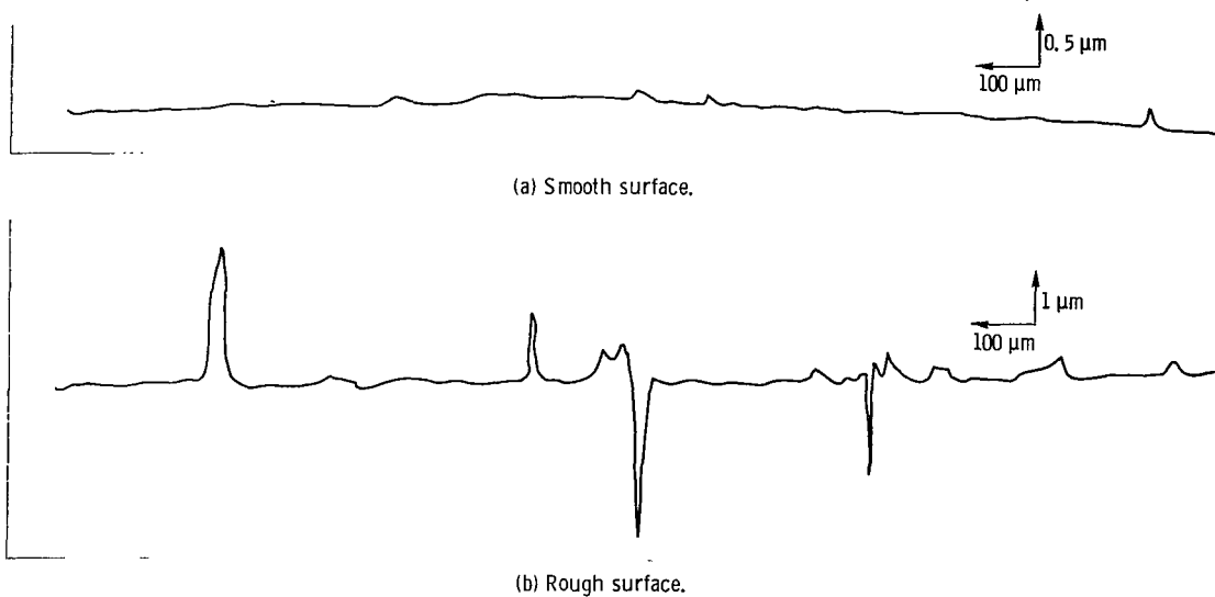
Figure 12. - Surface profile curves for silicon carbide after sputter cleaning.
