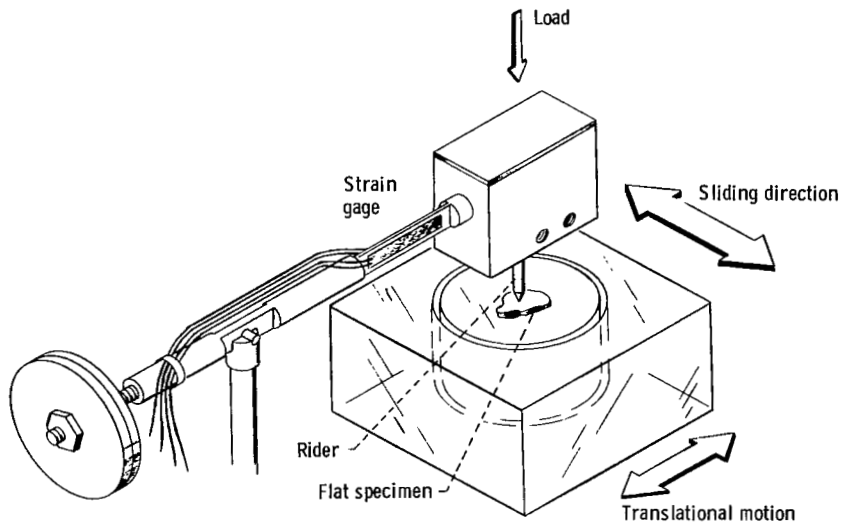
(a) Apparatus used in argon.
