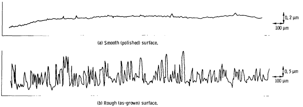
Figure 2. - Surface profile curves for silicon carbide.
