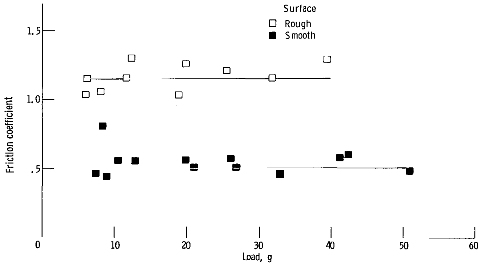
Figure 13. - Friction coefficient as function of load for titanium sliding on single-crystal silicon carbide (0001) surface in vacuum ( 10^{-8} N/m 2 ). Sliding velocity, 0.7 mm/min; temperature, 25° C.
