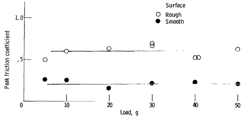
Figure 3. - Friction coefficient as function of load for titanium sliding on single-crystal silicon carbide (0001) surfaces in argon at atmospheric pressure. Sliding velocity, 3 mm/min; temperature, 25 o C.
