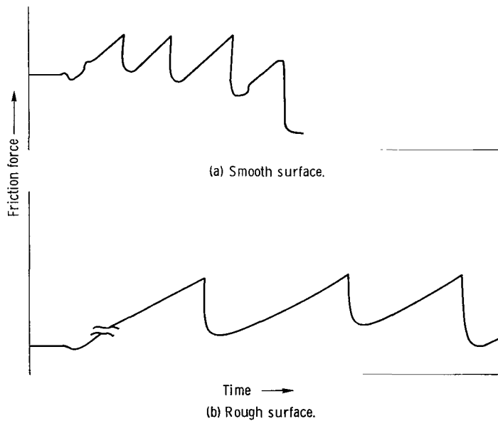
Figure 14. - Friction force traces for titanium sliding on single-crystal silicon carbide (0001) surfaces in vacuum. Sliding velocity, 0.7 mm/min; load 40 grams; temperature, 25° C; pressure, 10^{-8} N/m 2 .
