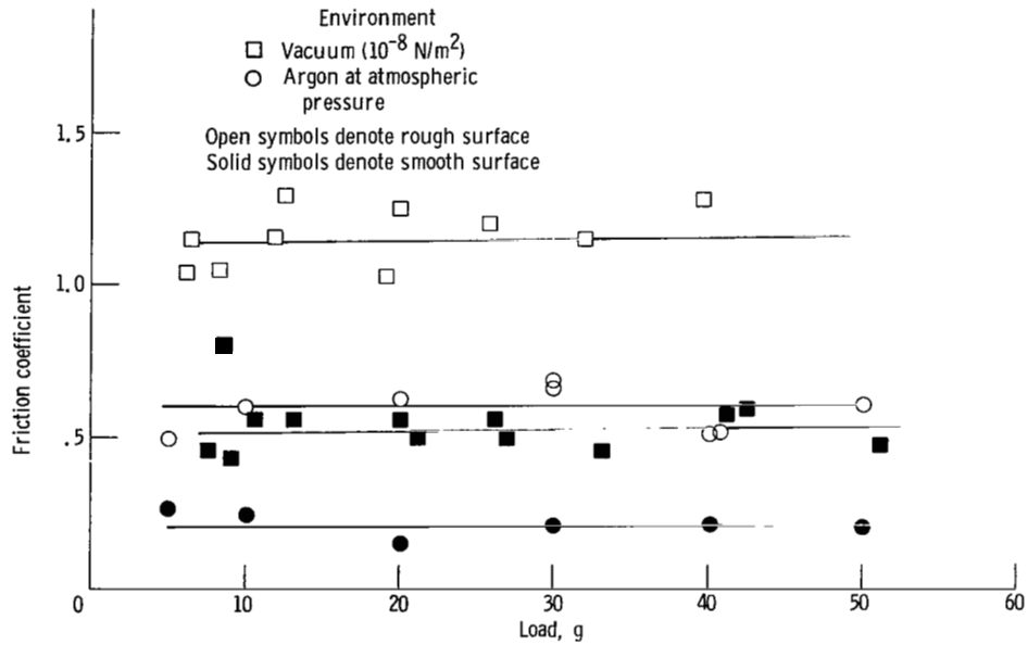
Figure 24. - Friction coefficient as function of load for titanium sliding on single-crystal silicon carbide (0001) surfaces both in argon at atmospheric pressure and in high vacuum. Sliding velocity, 3 mm/min in argon at atmospheric pressure and 0.7 mm/min in vacuum; temperature, 25° C.
