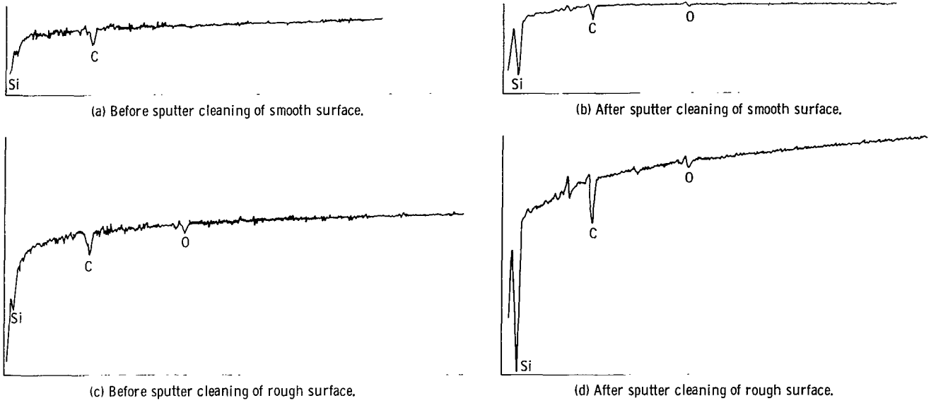
Figure 11. - Auger emission spectroscopy spectra for silicon carbide single-crystal surfaces.
