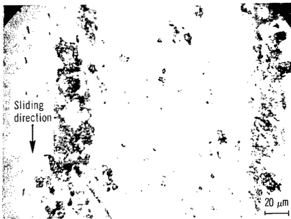
Figure 20. - Wear tracks on smooth silicon carbide surface. Sliding velocity, 0.7 mm/min; load, 40 grams; temperature, 25° C; pressure, 10^{-8} N/m 2 .
