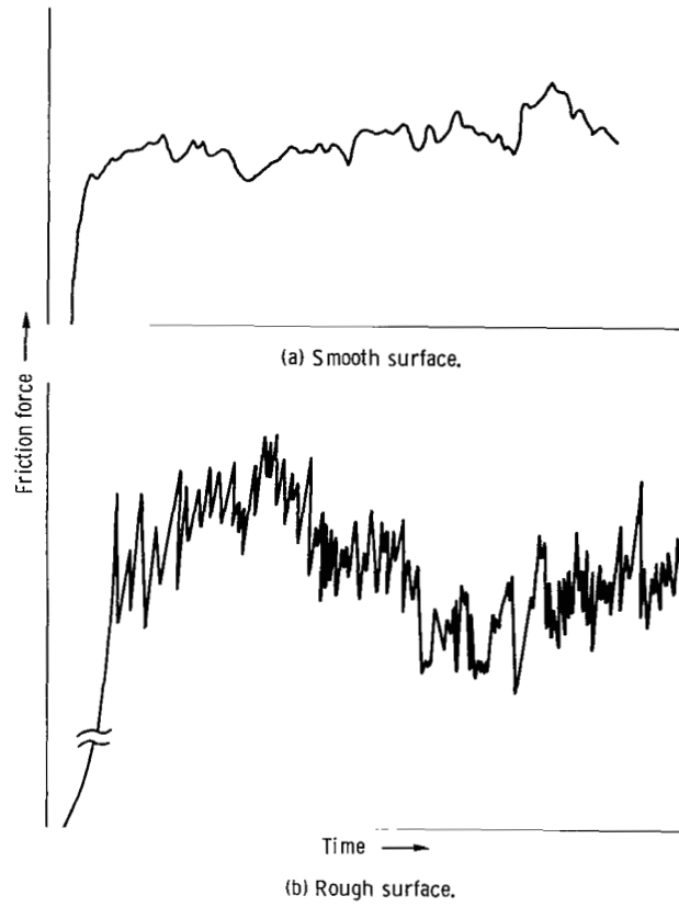
Figure 4. - Friction force traces for titanium sliding on single-crystal silicon carbide (0001) surfaces in argon. Sliding velocity, 3 mm/min; load, 20 grams; temperature, 25° C; environment, argon; pressure, atmospheric.
