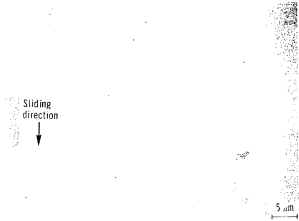
Figure 21. - Silicon carbide wear debris generated by fracture. Sliding velocity, 0.7 mm/min; load, 40 grams; temperature, 25°C; pressure, 10^{-8} N/m 2 .
