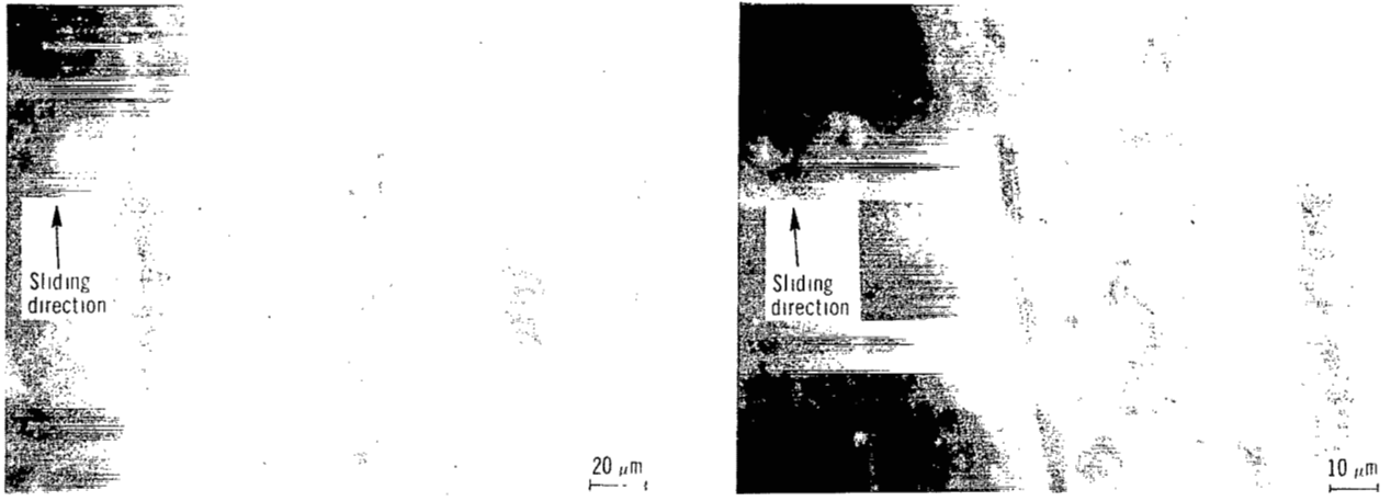
Figure 23. - Wear track on rough silicon carbide surface. Sliding velocity, 0.7 mm/min; load, 40 grams; temperature, 25° C; pressure, 10^{-8} N/m 2 .
