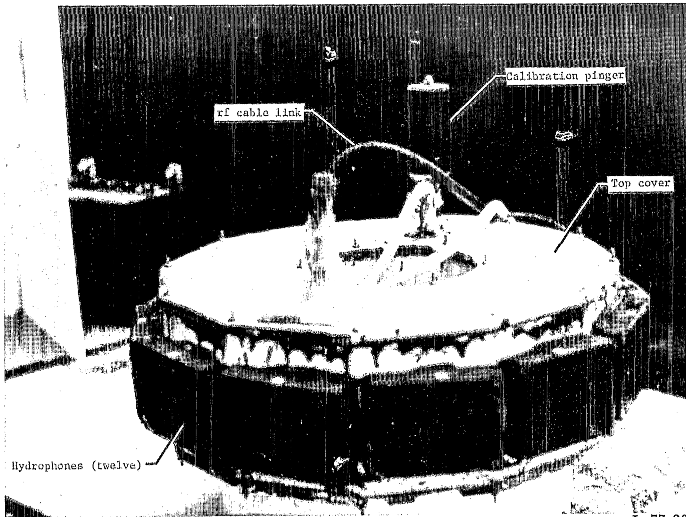
(a) Listening-station assembly.
