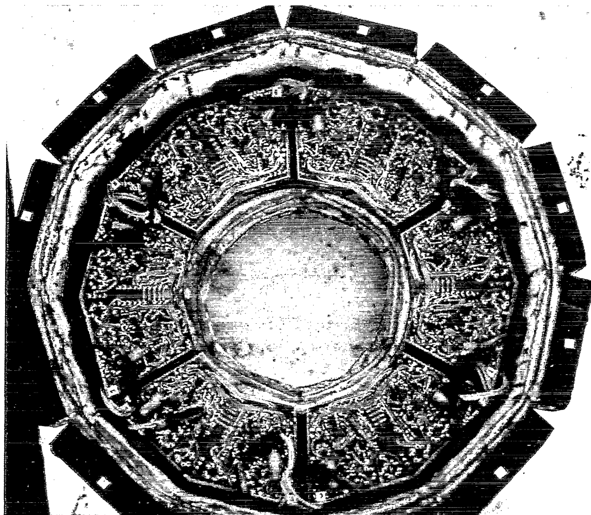
(b) Electronic receivers (top cover removed).
