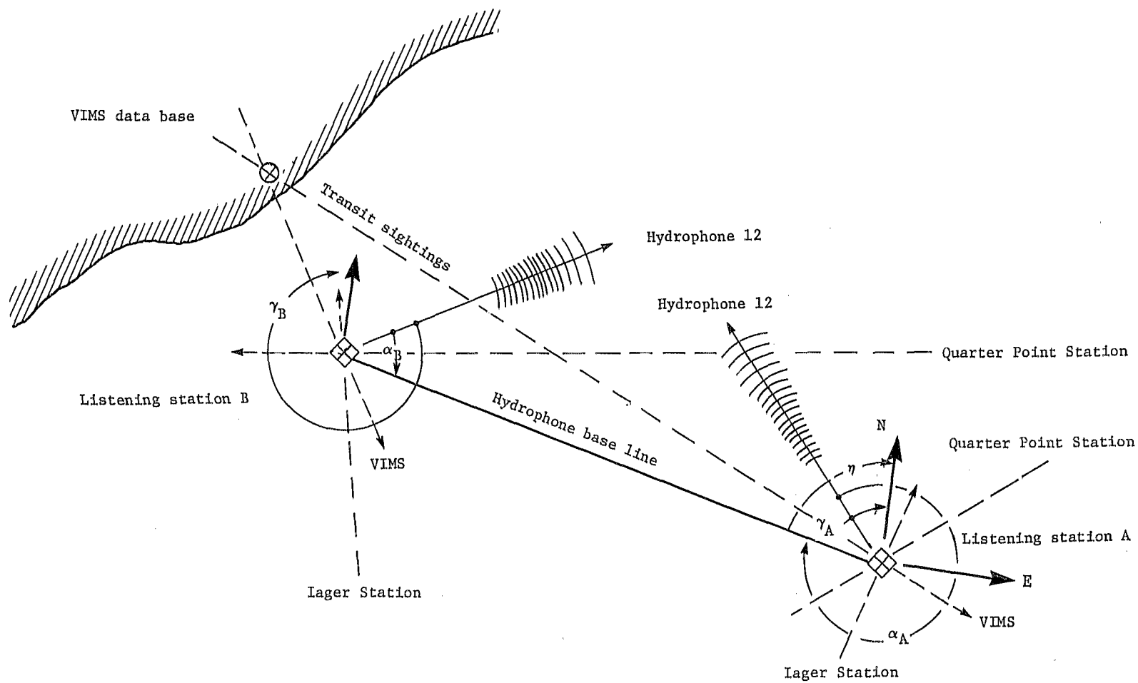
Figure 10.- Parameters for listening-station calibration.
