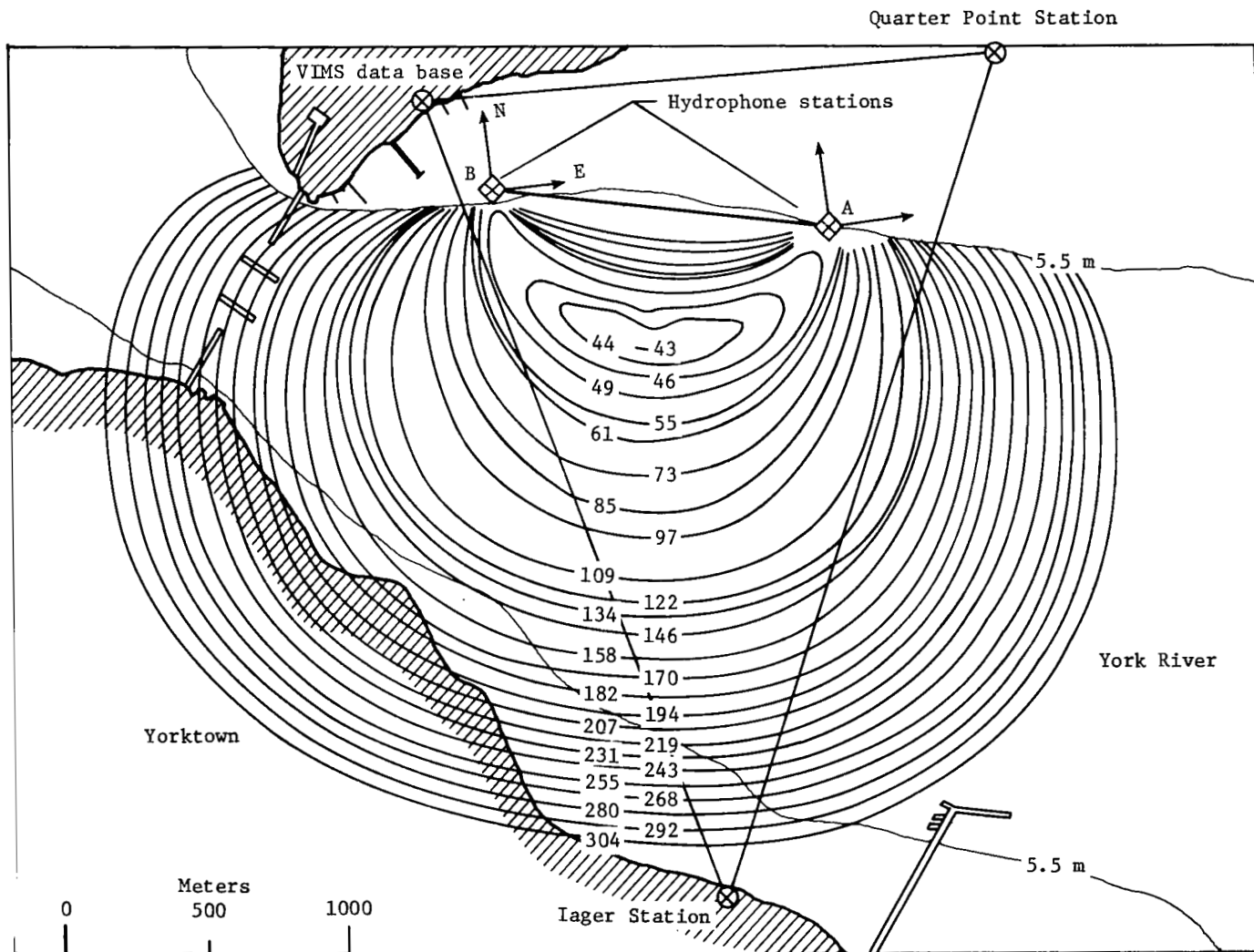
Figure A1. - Accuracy contours in meters (95 percent confidence with \pm 2.5^{\circ} error).
