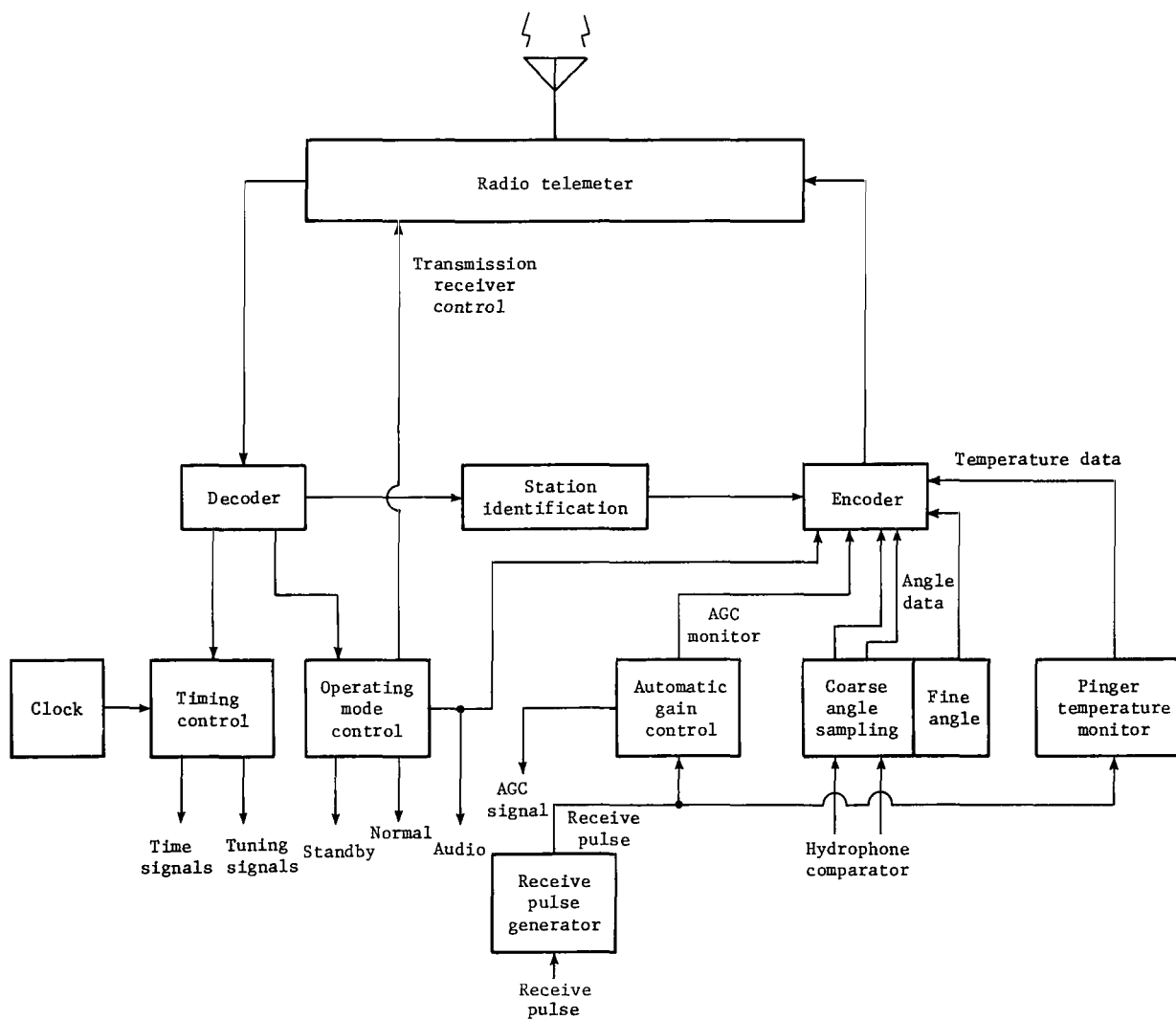
(b) Listening-station logic electronics.
