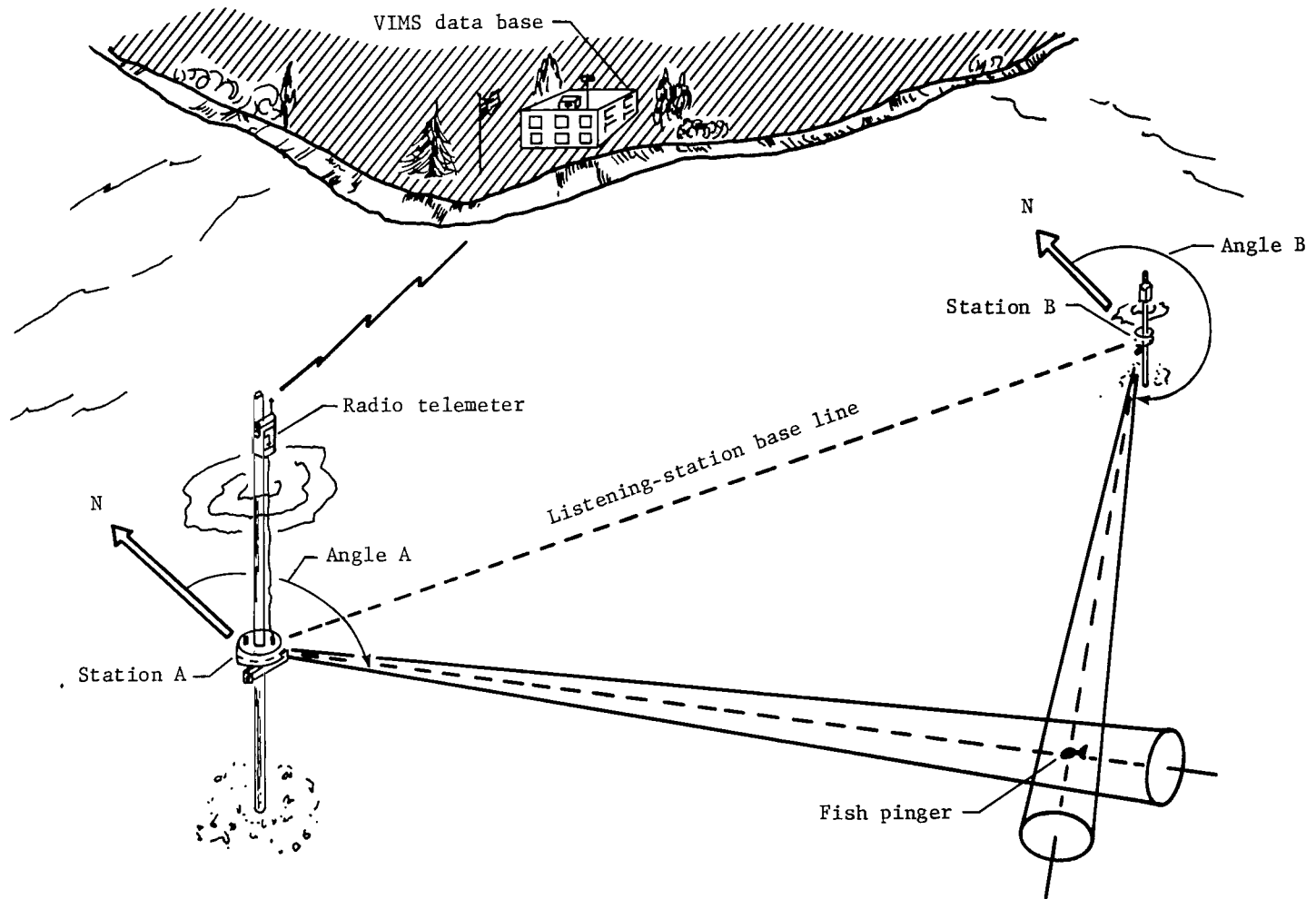
Figure 1.- Prototype test installation in York River:
