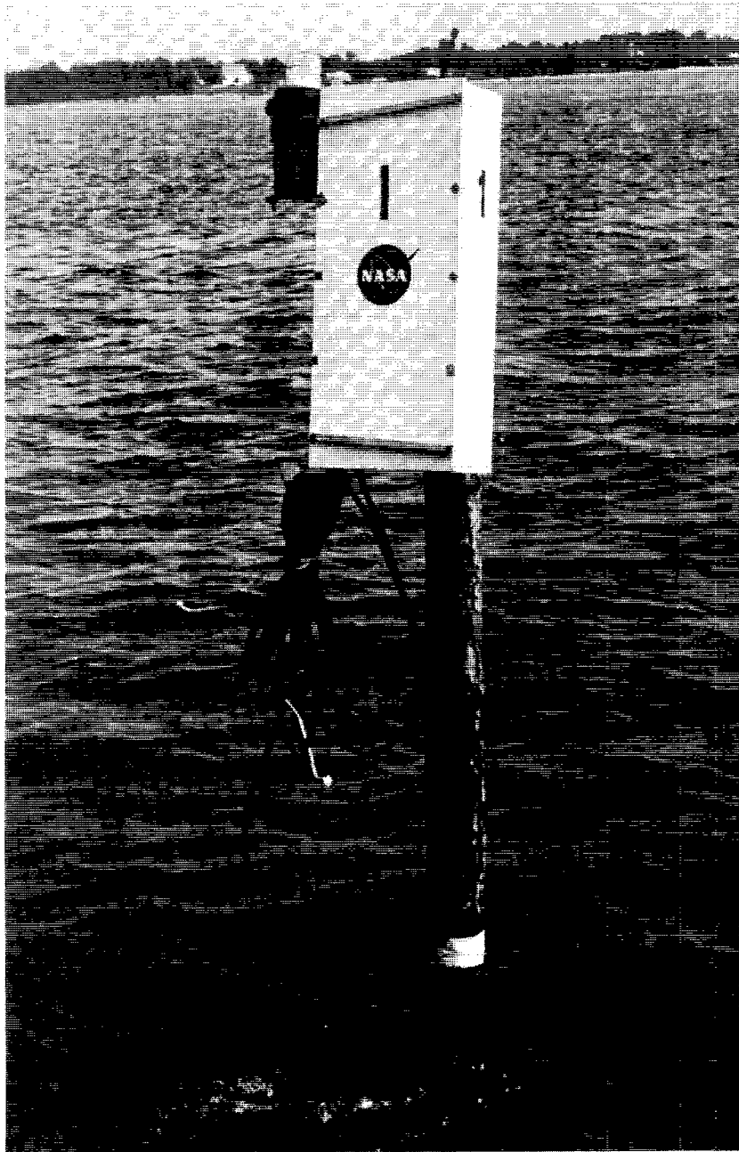
Figure 8. - Field installation of listening station.
