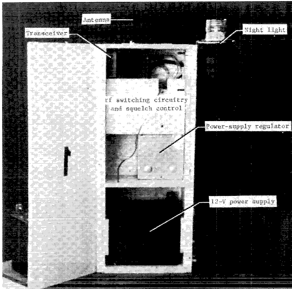
Figure 6.- Radio telemeter.
