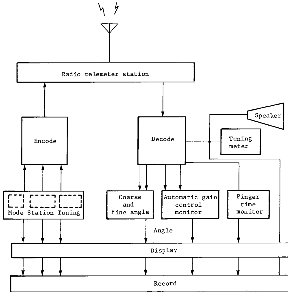
(c) Shore data base circuitry.
