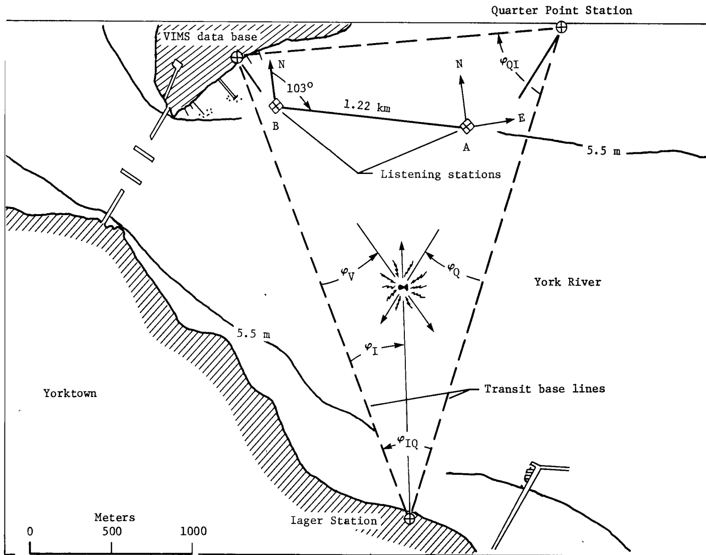
Figure 9.- Locations of fish-tracking system and transit-tracking range.
