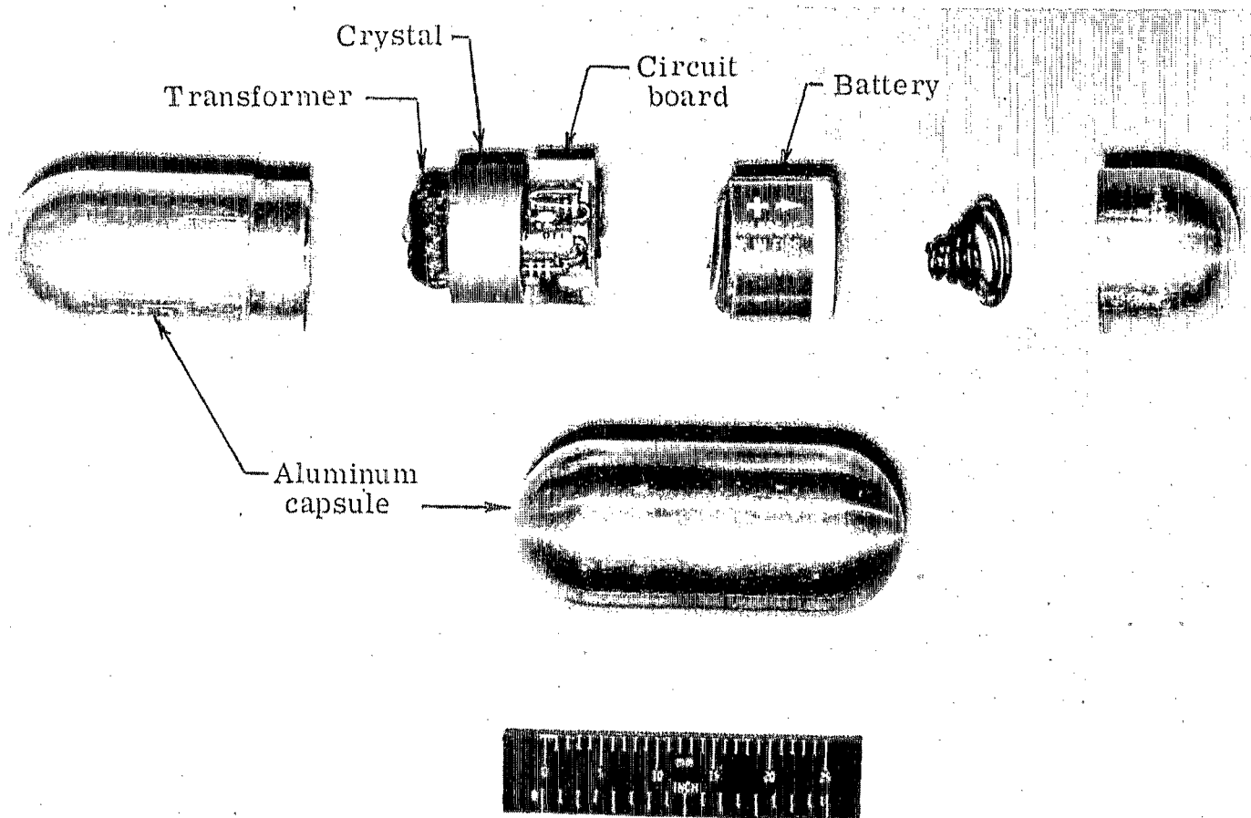
Figure 2. - Fish pinger.
