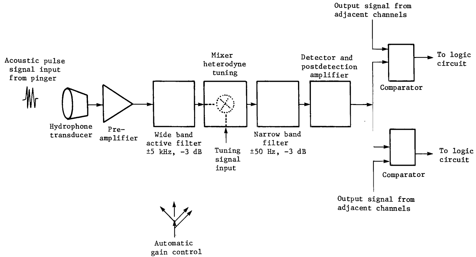
(a) Hydrophone receiver channel.
