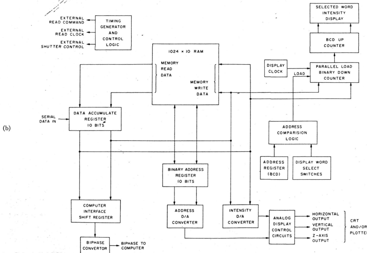
FIG. 5. Block diagram of data-handling and display electronics. (a) Pulse-counting and coincidence-detection circuits; (b) digital and analog display circuits.
