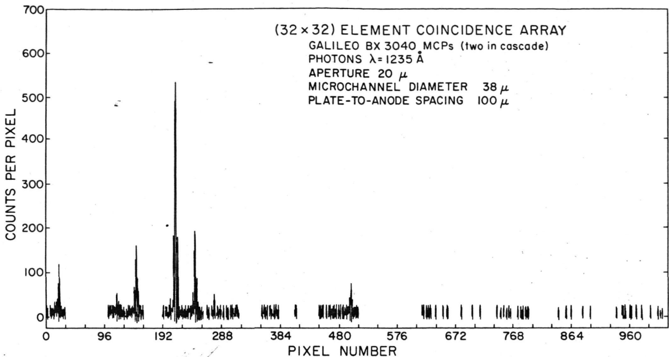
FIG. 11. Image of 20- \mu pinhole recorded with breadboard (32 \times 32)-element array. Analog plotter output. Discriminator threshold 1 \times 10^6 electrons \cdot pulse ^{-1} .
