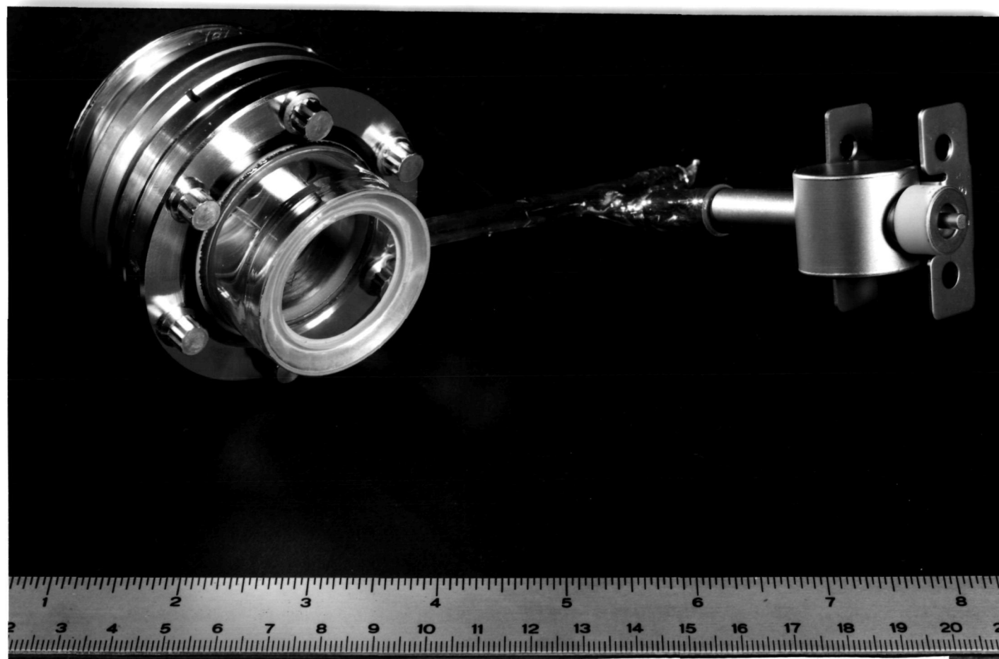
Figure 18. Demountable UV tube assembly with MgF_2 window and appendage ion-pump for outgassing tests.
