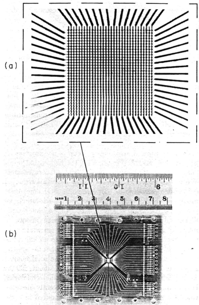
FIG. 2. Breadboard (32 \times 32) -element array. (a) Photomask; (b) assembled array of aluminum electrodes on quartz substrate.
