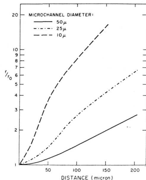
Fig. 19. Variation in the radius of the electron beam as a function of the distance between the MCP output and the anode array for a MCP gain of 2 \times 10^7 and a MCP-to-anode bias potential +150 V.
