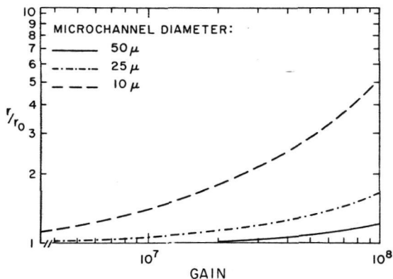
Fig. 21. Variation in the radius of the electron beam as a function of the gain of the MCP. MCP-to-anode spacing 25 μm and MCP-to-anode bias potential +150 V.
