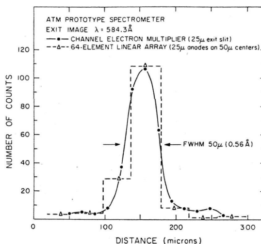
Fig. 15. Exit profile of the EUV spectrometer recorded with a CEM mounted behind a 25- \mu m exit slit and with the MCP array (discriminator threshold 3.0 \times 10^7 electrons pulse ^{-1} ).
