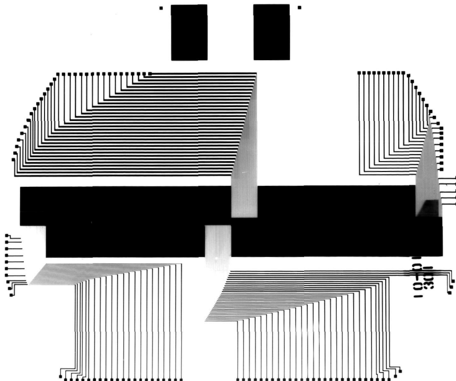
Figure 13. Photographic masks for production of (2 \times 1024) -pixel coincidence-anode array.
