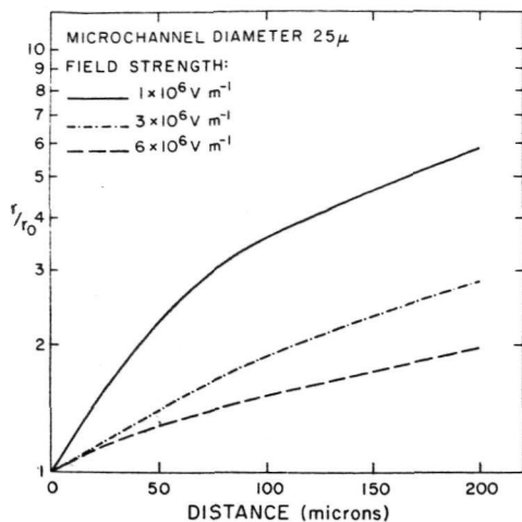
Fig. 20. Variation in the radius of the electron beam as a function of the accelerating electrostatic field for MCP with 25-μm diam microchannels and a gain of 2 × 10 7 .
