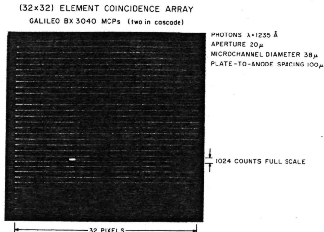
FIG. 10. Image of 20\text{-}\mu pinhole recorded with breadboard (32 \times 32) -element array. Video display output. Discriminator threshold 2 \times 10^6 electrons \cdot pulse -1 .
