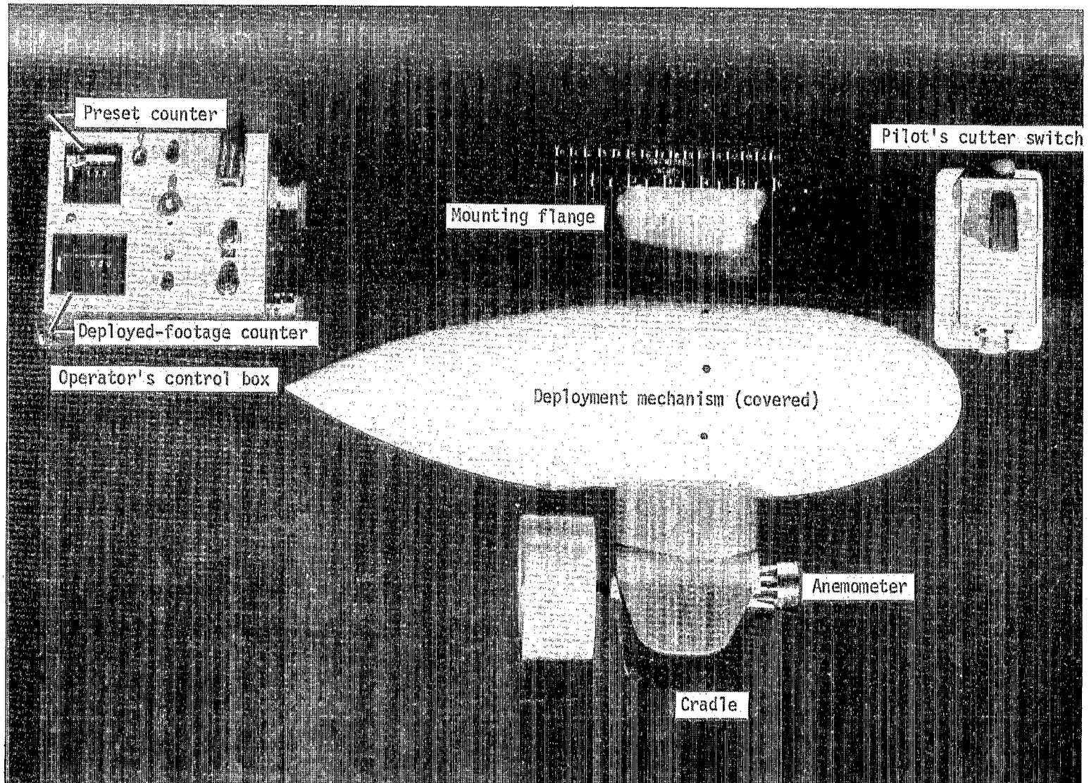
Figure 5.- Complete system with anemometer retracted.
