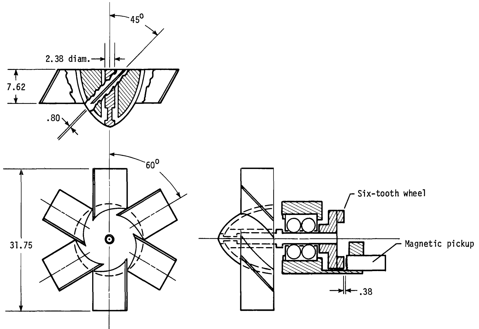
Figure 4.- Propeller-tachometer assembly. (Linear dimensions are in mm.)
