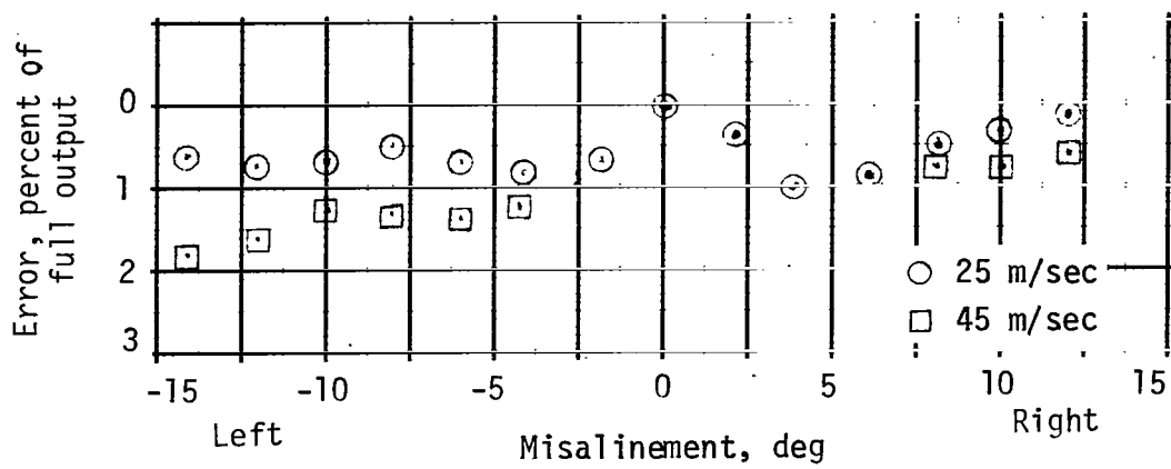
Figure 11.- Variation of anemometer output with misalignment.
