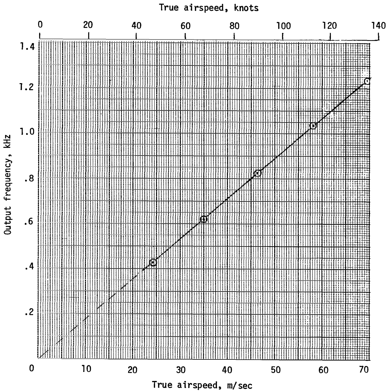
Figure 10.- Anemometer calibration based on wind-tunnel cross-section velocity profile.
