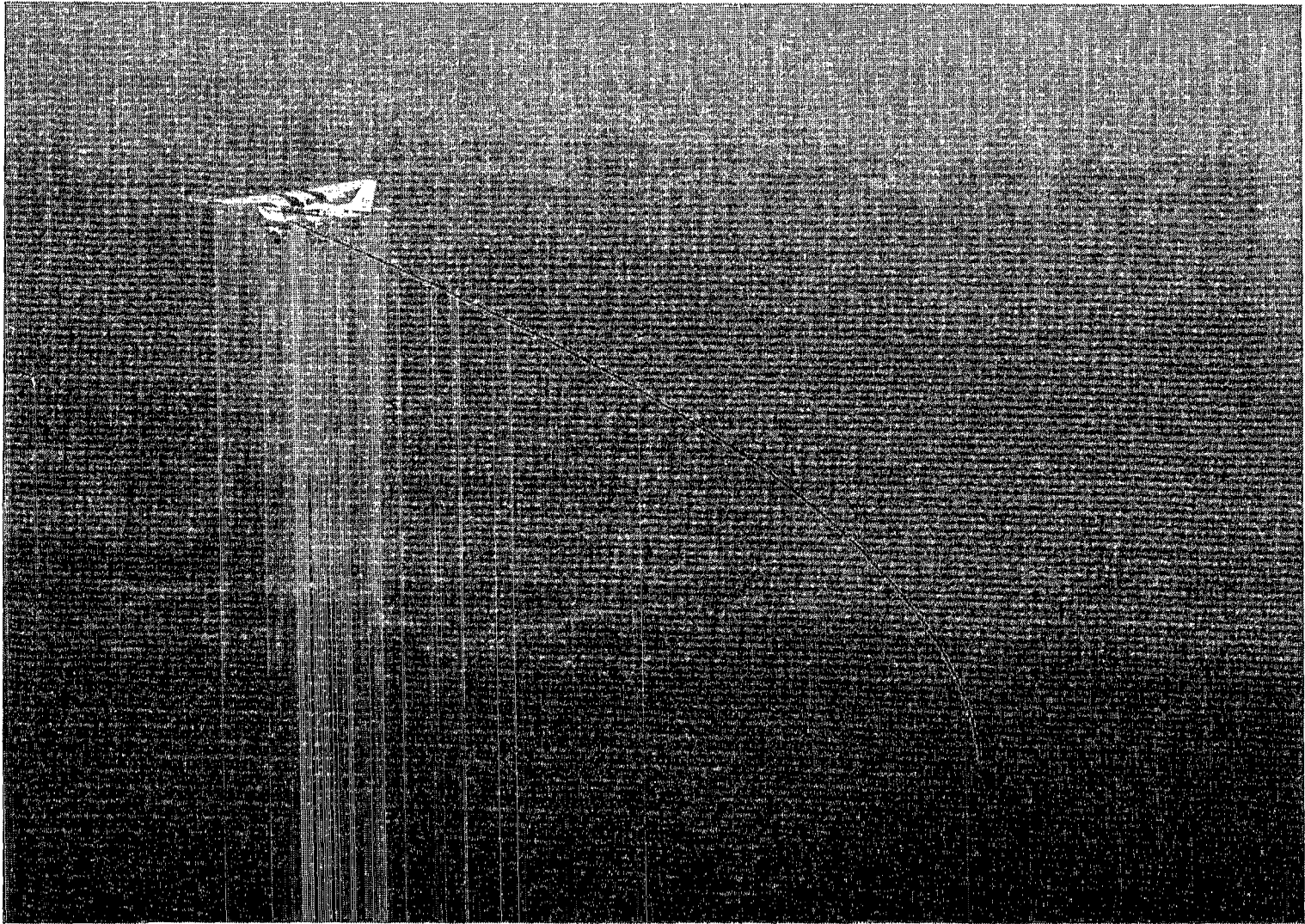
Figure 13.- Anemometer suspended from light airplane. (Image of cable has been enhanced.)
