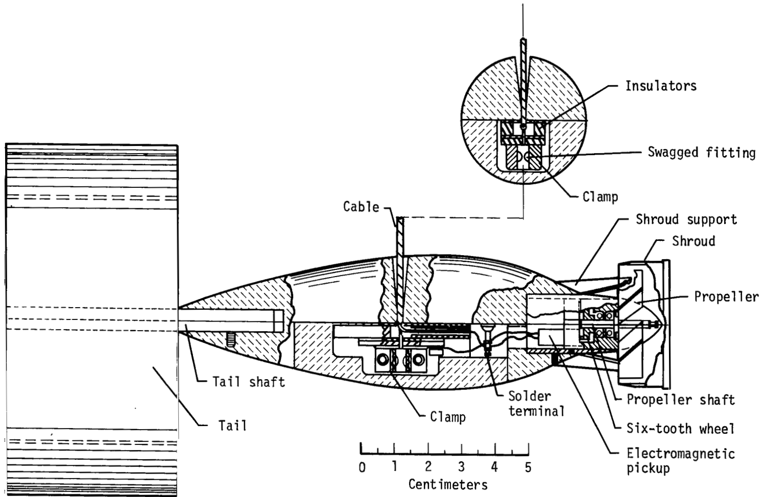
Figure 3.- Anemometer body.
