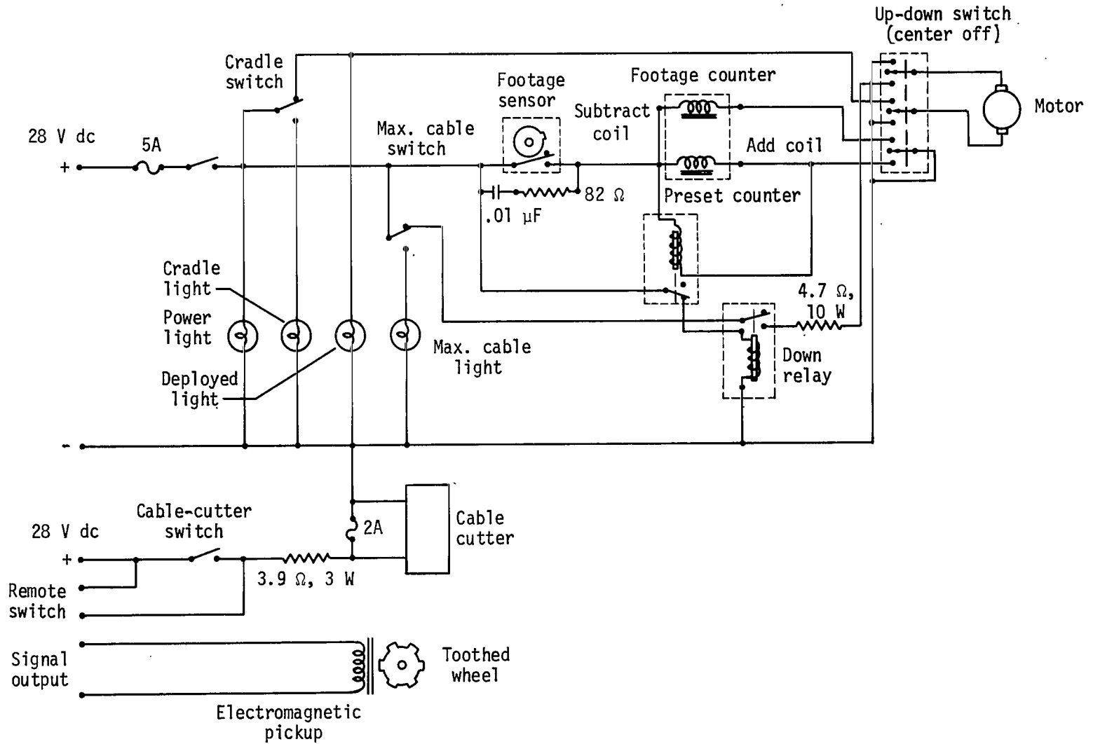
Figure 8.- Schematic of electrical system.
