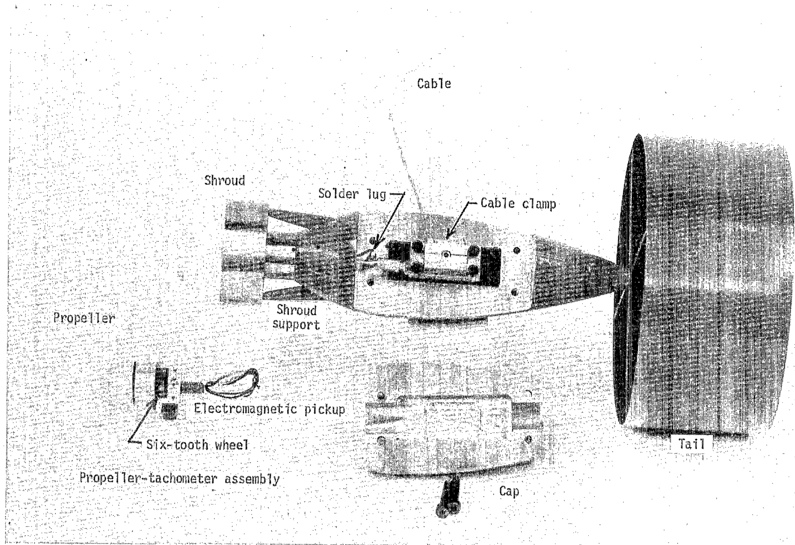
Figure 2.- Partially disassembled anemometer.
