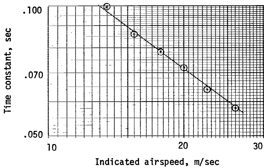
Figure 12.- Variation of anemometer time constant with indicated airspeed.
