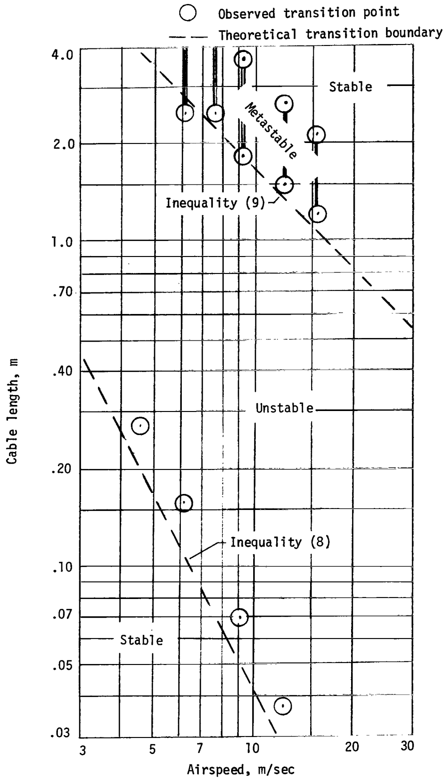
Figure 15.- Comparison of theoretical and observed lateral-pendulum stability of anemometer.
