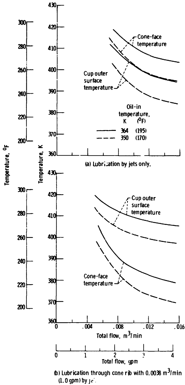
Figure 11. - Effect of oil-in temperature on cone-face and cup outer surface temperatures. Shaft speed, 10 000 rev/min; thrust load, 53 400 N (12 000 lb); radial load, 6 800 N (1 500 lb).
