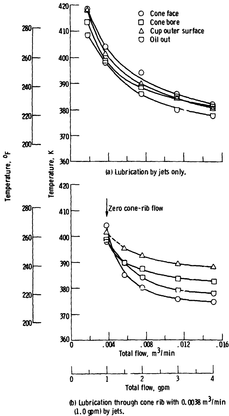
Figure 4. - Temperature as a function of flow rate at shaft speed of 6000 rpm. Thrust load, 53 400 N (12 000 lb); radial load, 26 700 N (6000 lb); oil-in temperature, 364 K (195° F).
