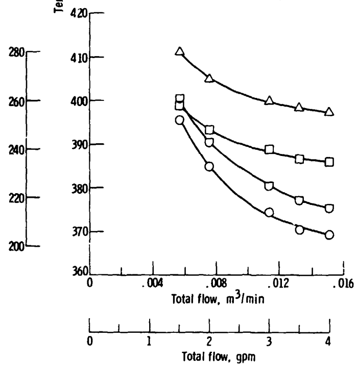
Figure 5. - Temperature as a function of flow rate at a shaft speed of 10 000 rpm. Thrust load, 53 400 N (12 000 lb); radial load, 26 700 N (6000 lb); oil-in temperature, 350 K (170° F).
