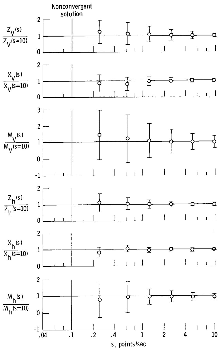
Figure 14. Effect of sampling rate on velocity and altitude derivatives for phugoid maneuver A.
