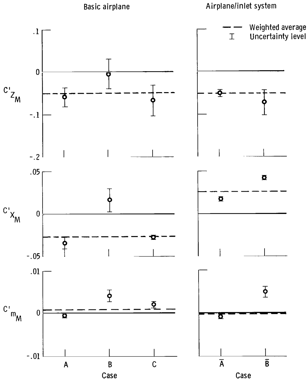
Figure 8. Velocity and altitude derivatives obtained from phugoid maneuvers.
