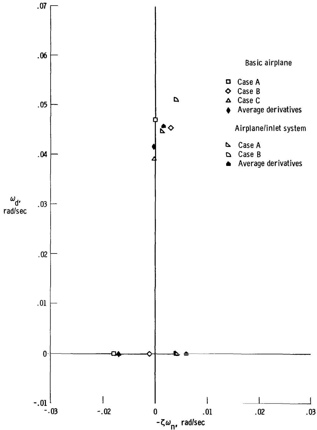
Figure 11. Phugoid and height mode roots for individual cases and weighted average derivatives from figure 8 for M = 2.9 and h = 21,900 m (72,000 ft).
