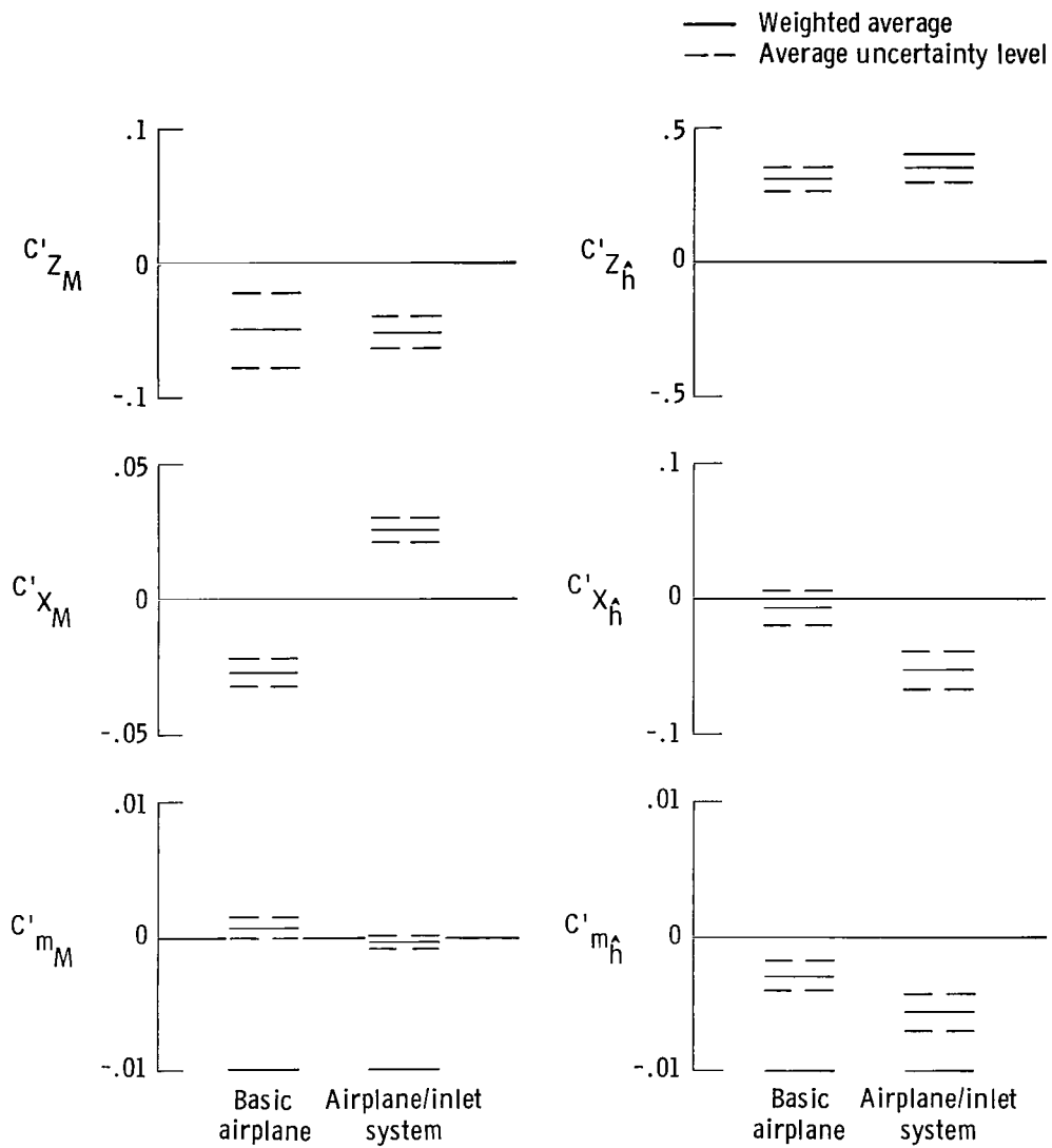
Figure 9. Summary of velocity and altitude derivatives and average uncertainties for M \approx 2.9 , h \approx 21,900 m (72,000 ft).
