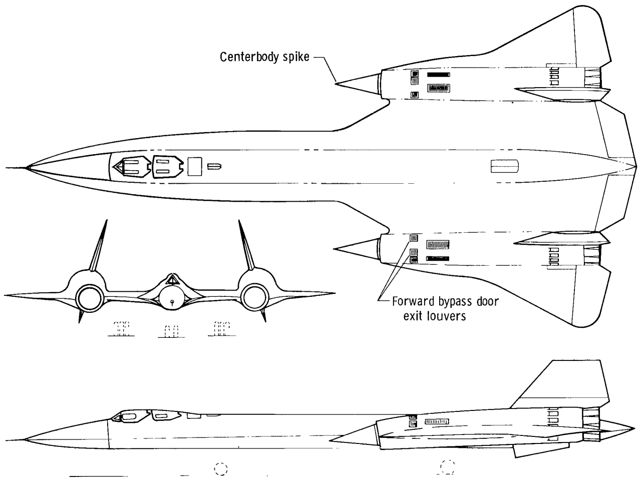
Figure 2. Three-view drawing of test airplane.
