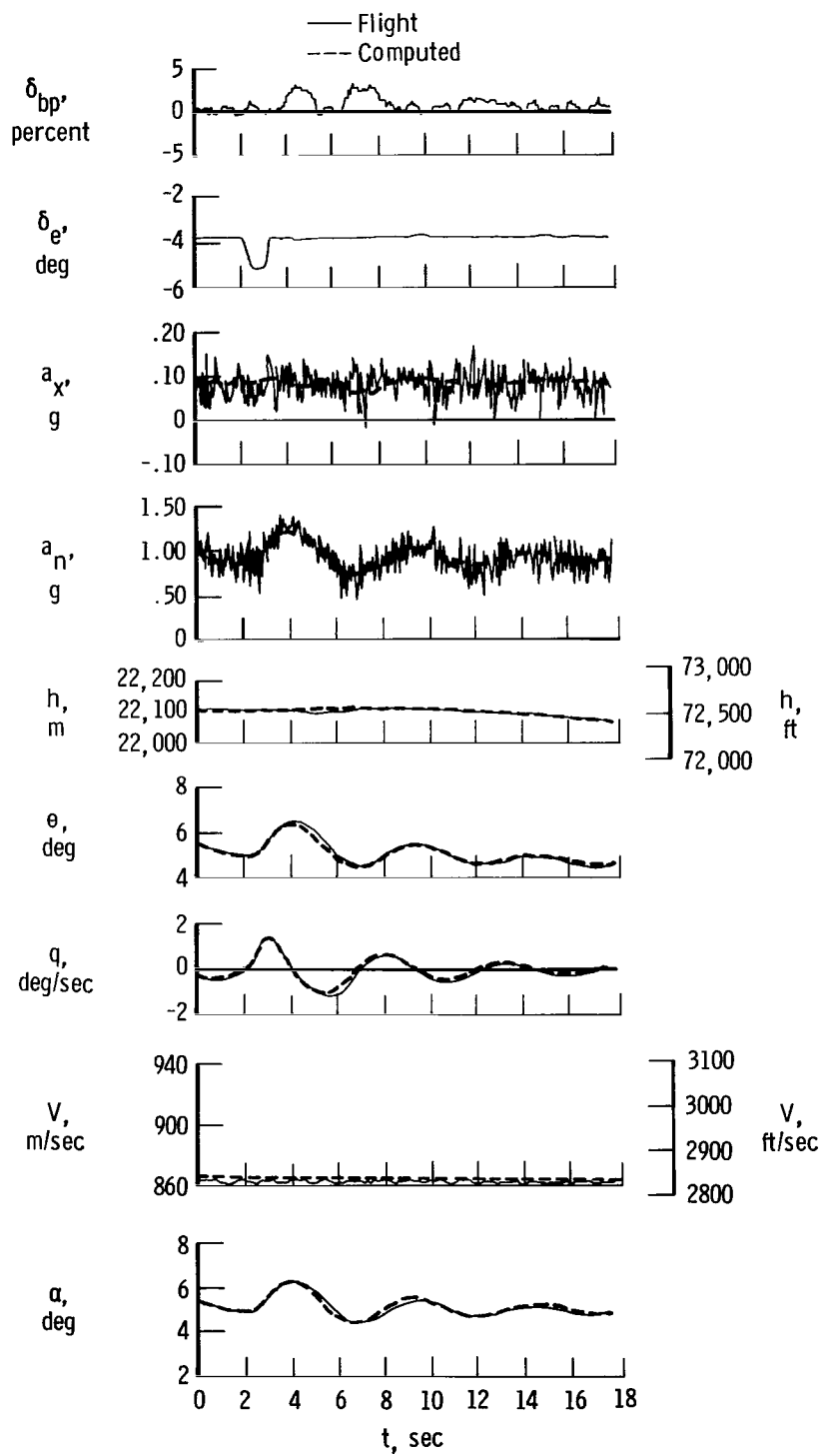
Figure 6. Typical short-period match using average derivatives. Case A1.
