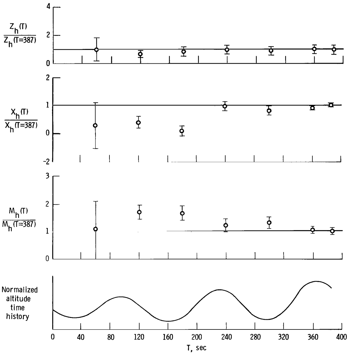
Figure 15. Effect of observation time on velocity and altitude derivatives for fixed sample rate of 2 points per second with phugoid maneuver A. (Derivatives shown at T correspond to observation of time history from 0 to T.)
