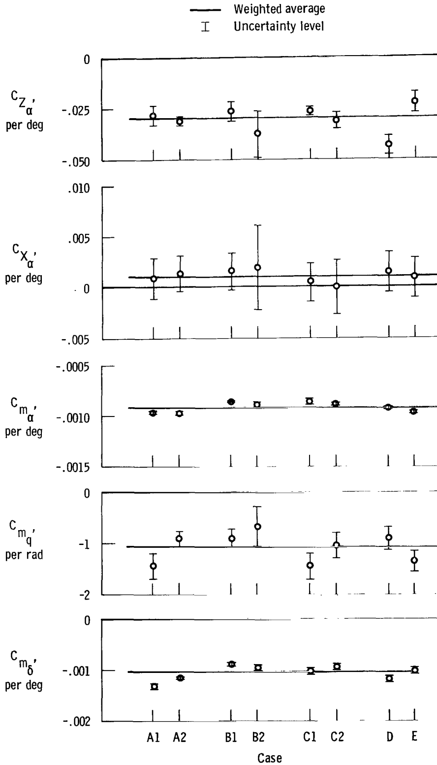
Figure 5. Short-period derivatives. M \approx 2.9 .
