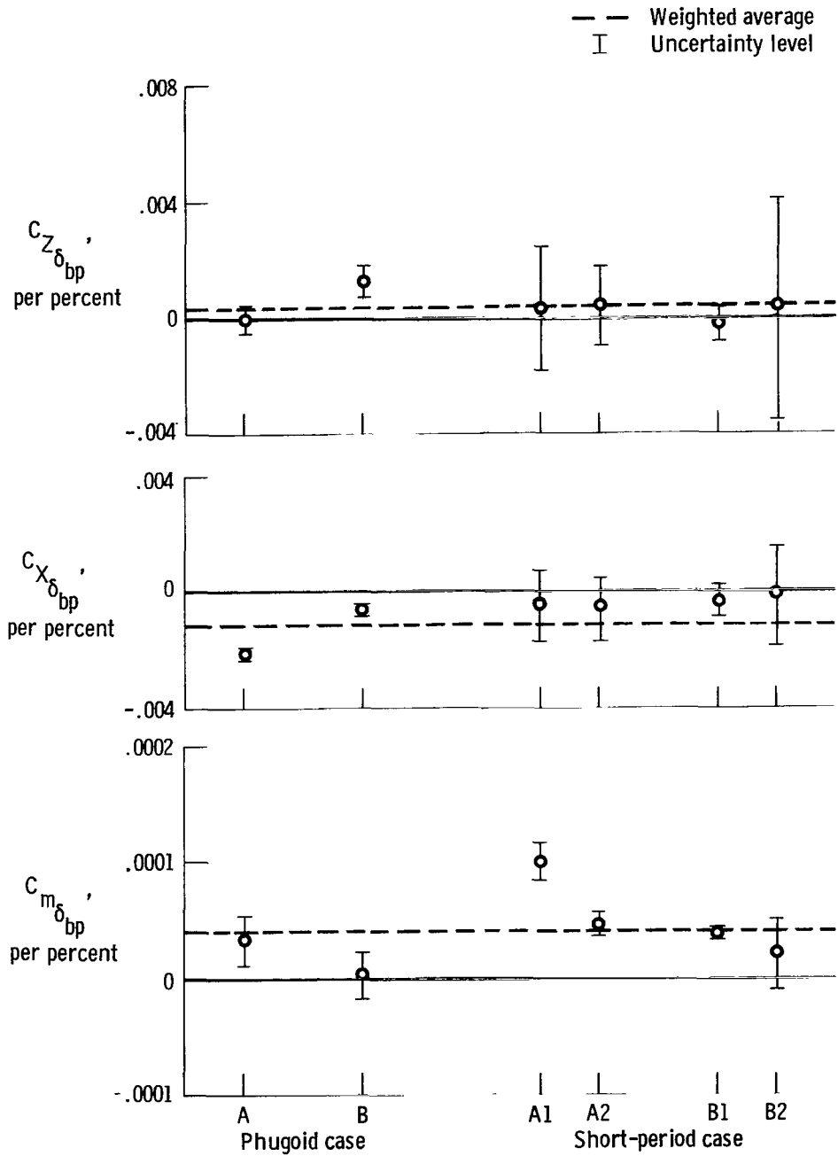
Figure 10. Inlet derivatives.
