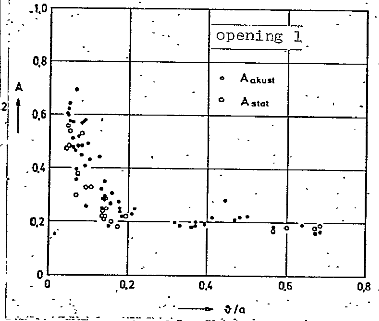
Figure 13: A is a function of boundary layer thickness.
