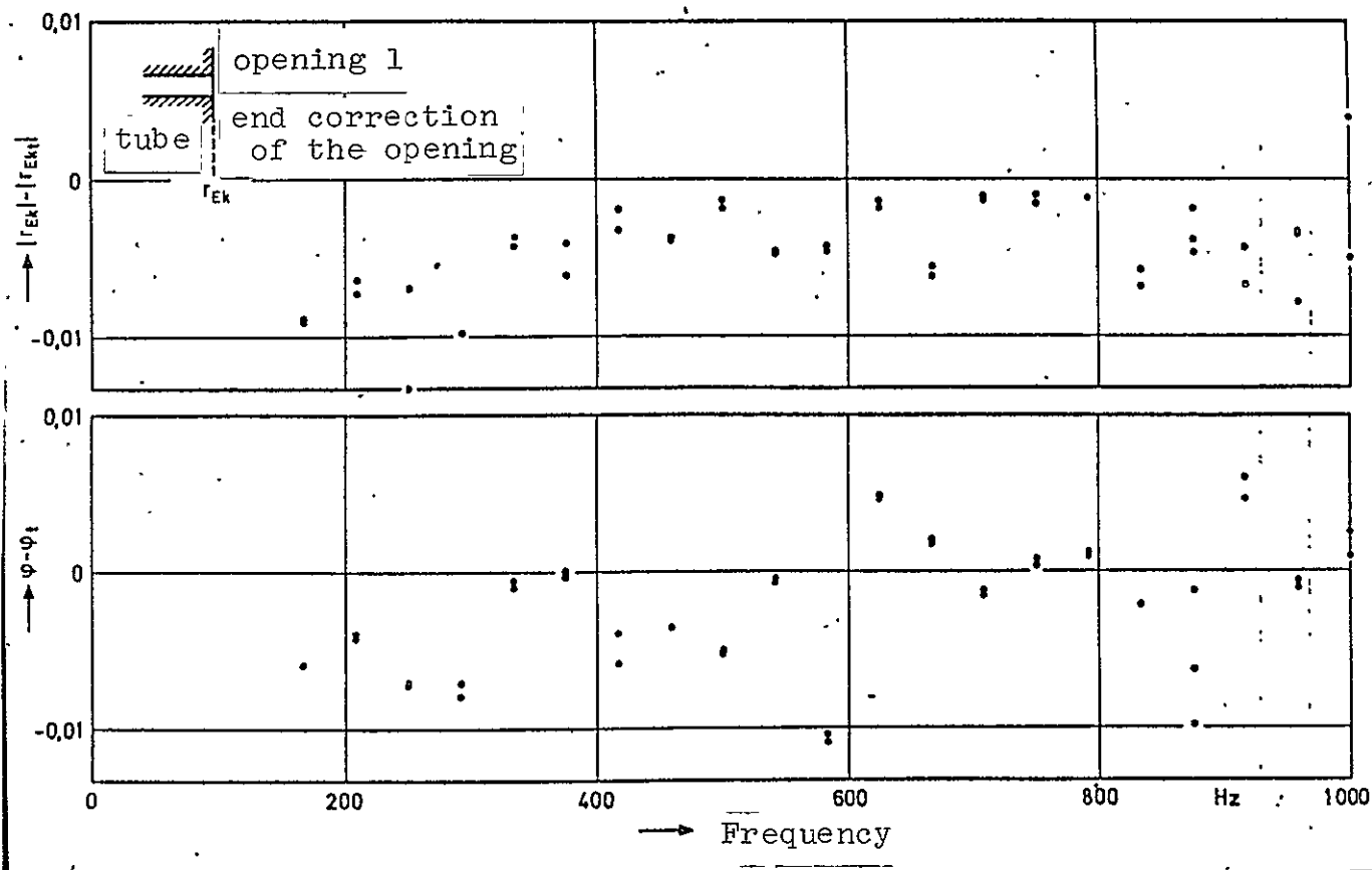
Figure 4: Difference between the measured and theoretical reflection factors in the plane of the opening upper edge, magnitude and phase (arc scale) ( a = 2 \text{ mm} , |r_{Ek}| \sim 1 , \phi \sim \pi )
