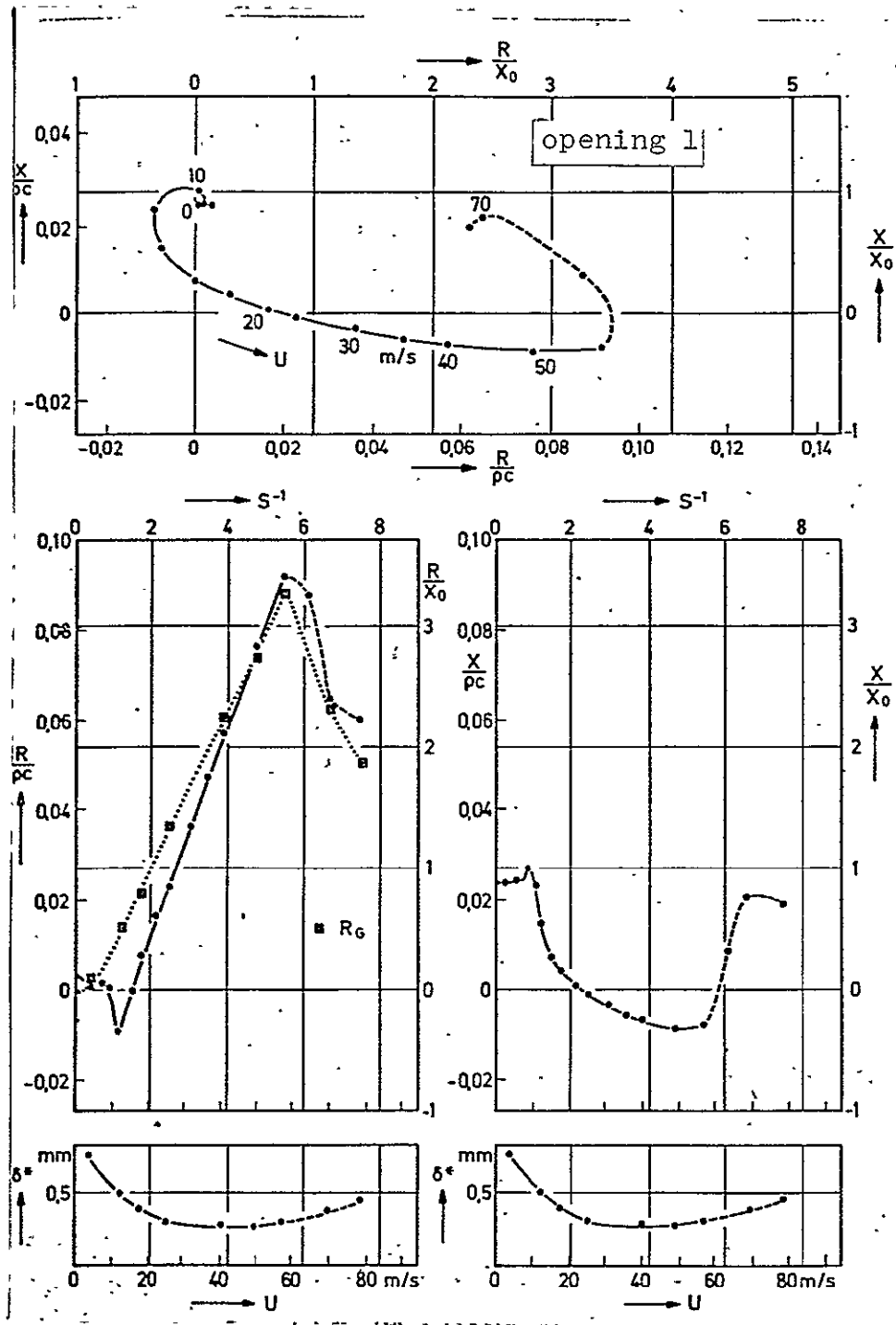
Figure 9: Impedance of the end correction of an opening ( a = 2 mm) as a function of the flow velocity at f = 833 Hz. ( R_G : uniform flow resistance of opening).
