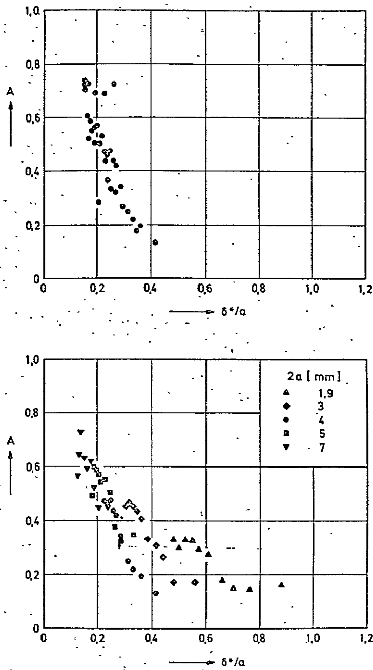
Figure 22: Value of A from uniform flow measurements.
