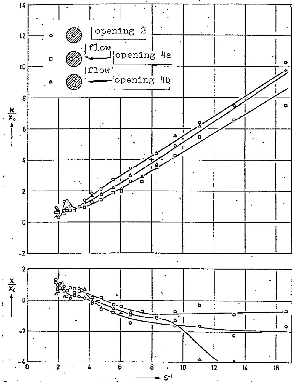
Figure 18: Real and imaginary parts of the impedance of the end correction of an opening ( a = 2 mm) for 2 adjacent openings ( U = 69.8 m/s, \delta^* = 0.68 mm).
