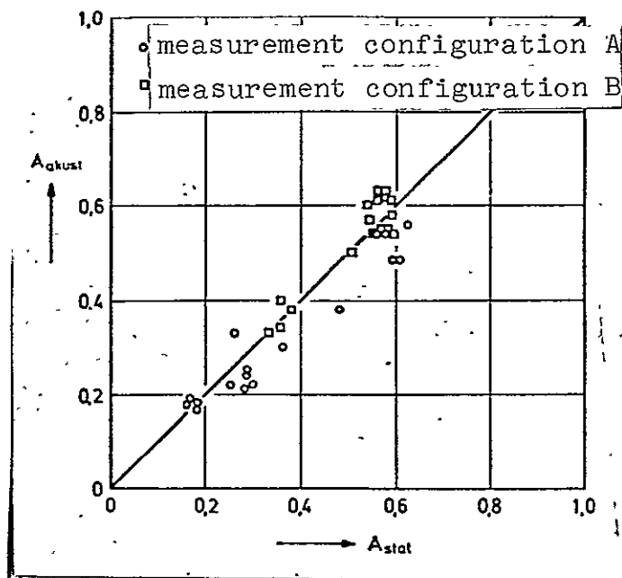
Figure 12: Comparison between the acoustic and the uniform flow measurements used to determine A.
