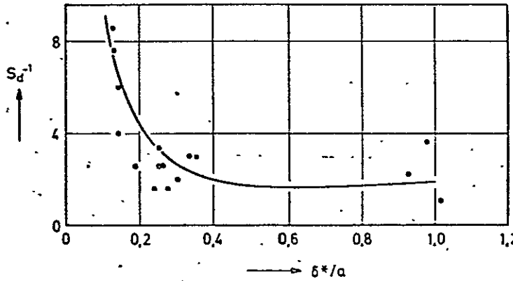
Figure 16: Imaginary part of impedance of the end correction opening (a = 2 mm). a) for different boundary layer thicknesses U = 40.3 m/s) b) Second maximum of the imaginary part, center. c) Reciprocal Strouhal number, where the curve deviated from the curve for the thinnest boundary layer.
