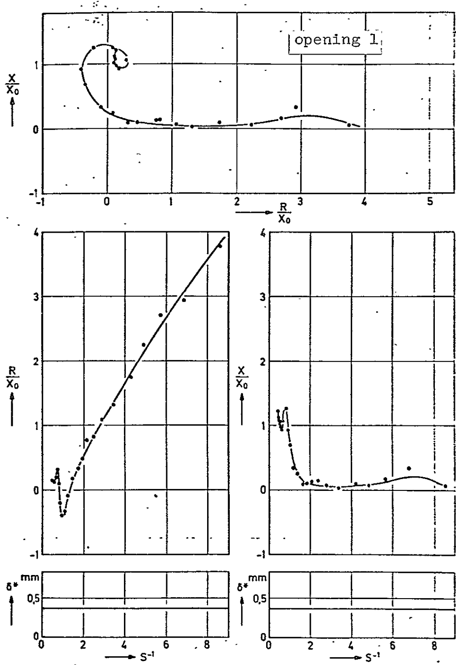
Figure 10: Impedance of end correction of an opening ( a = 2 mm) as a function of reciprocal Strouhal number ( \delta^* = 0.38 mm, U = 18 m/s).
