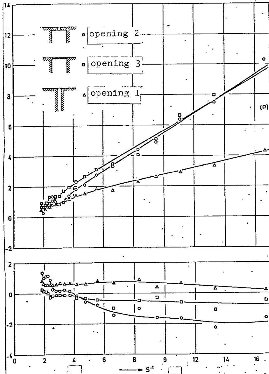
Figure 17: Real and imaginary part of the impedance of the end correction of an opening ( a = 2 \text{ mm} ) for different opening lengths ( \Delta measurement configuration A, \circ , \square measurement configuration B). U = 69.8 \text{ m/s} , \delta^* = 0.68 \text{ mm} ).
