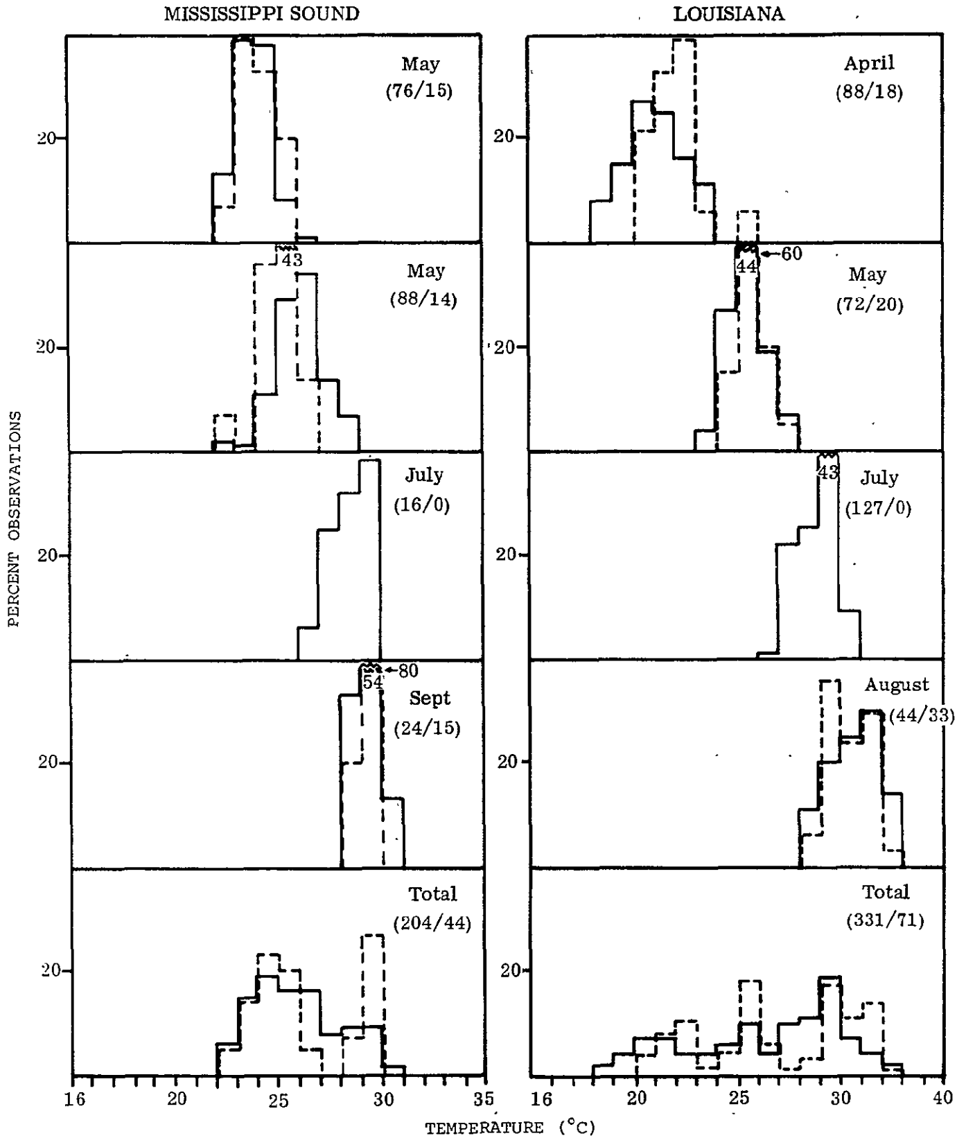
Figure 10-7. Comparison of Temperature ( ^{\circ}\text{C} ) Measurements from Locations of Menhaden Capture (solid lines) and Oceanographic Stations (broken lines) in the Mississippi Sound and Louisiana Study Areas. Numbers in Parentheses Represent Sample Sizes for the Menhaden and Oceanographic Samples Respectively.
