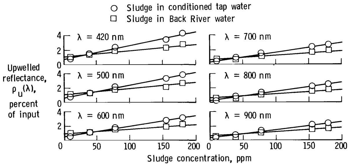
Figure 5.- Linearity of reflectance with concentration for various wavelengths.
