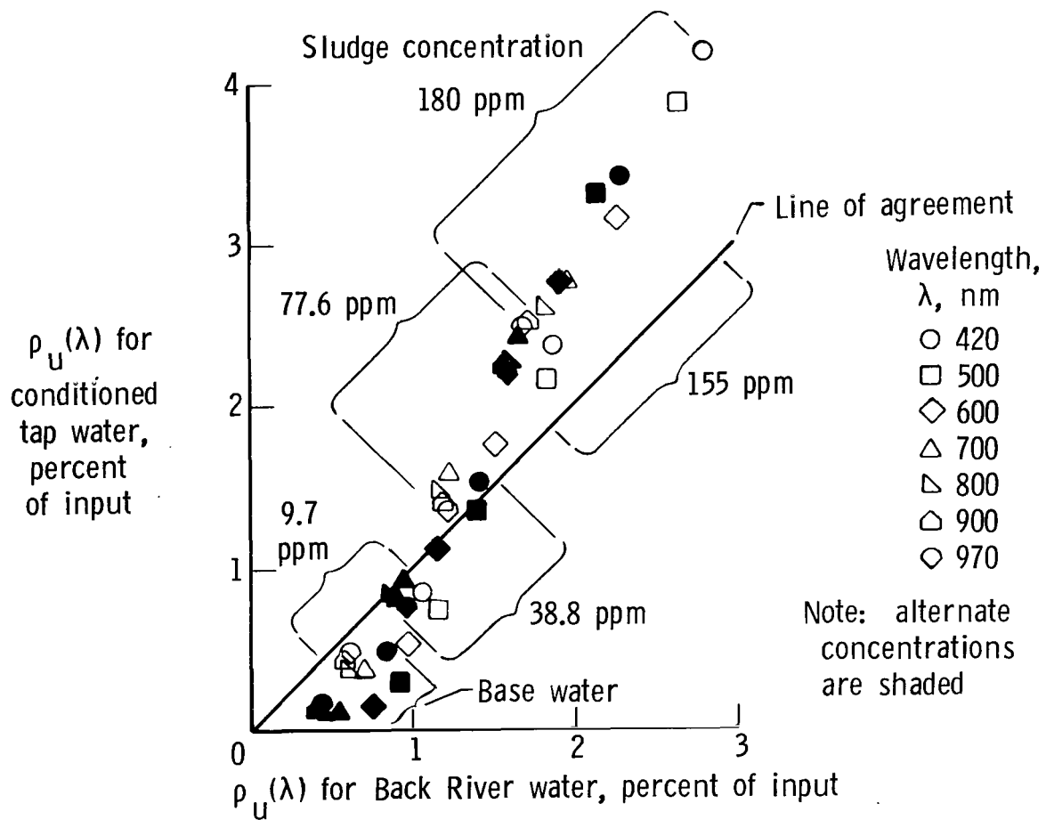
Figure 6.- Comparison of reflectance data for conditioned tap water and Back River water.
