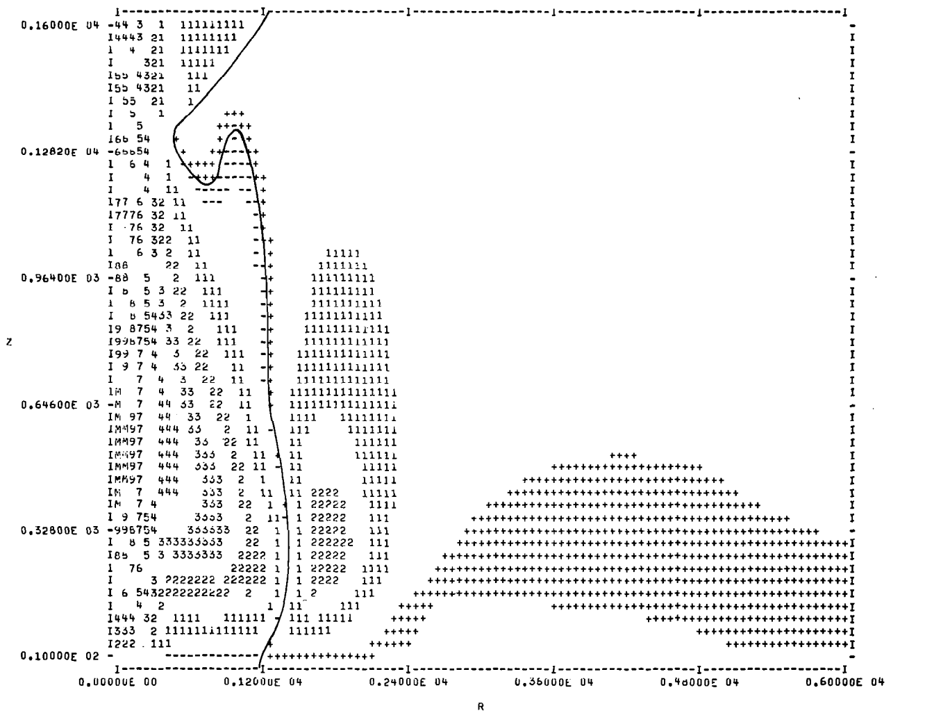
Figure 4.2.5. Normalized mean vertical velocity contours as a function of z and R for an axisymmetric gust front with a 500 m radius downdraft at t = 200 sec. [See figure 2.3.2 for explanation of notation.]
