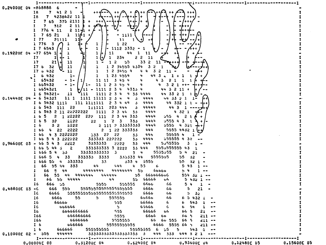
Figure 4.4.2. Normalized temperature contours as a function of z and y for a two-dimensional gust front with a 2000 m radius downdraft at t = 1000 sec. [See figure 2.3.2 for explanation of notation.]
