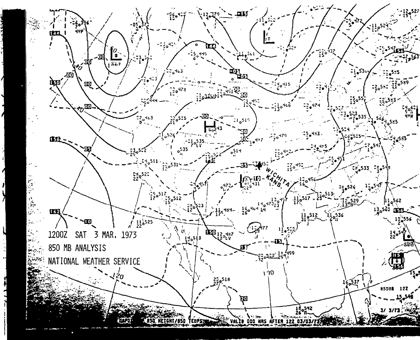
Figure 3.4.2. Early 850 mb chart for Wichita, Kansas, March 3, 1973 accident.
