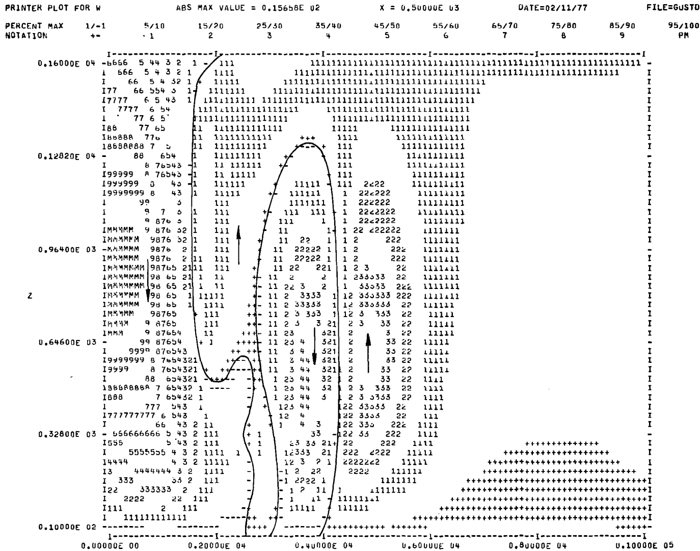
Figure 2.3.12. As above but t = 500 sec. [See figure 2.3.2 for explanation of notation.]
