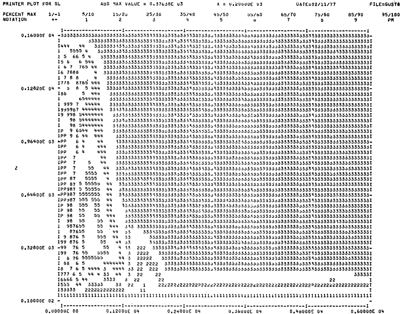
Figure 4.2.7. Normalized scale of turbulence contours as a function of z and R for an axisymmetric gust front with a 500 m radius downdraft at t = 200 sec. [See figure 2.3.2 for explanation of notation.]
