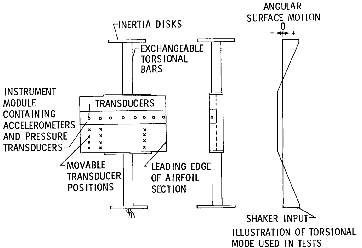
Figure 2.- Experimental model with illustration of torsional mode employed in tests.
