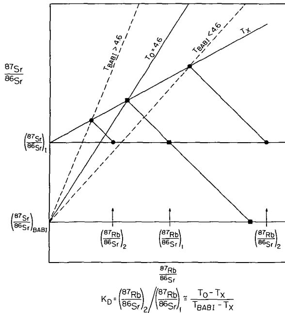
Figure 1.—Rb-Sr evolution diagram. Material formed at T_0 with (^{87}\text{Sr}/^{86}\text{Sr}) equal to (^{87}\text{Sr}/^{86}\text{Sr})_{BABI} is represented by a square. Fractionation at time T_x results in a portion enriched and a portion depleted in Rb relative to Sr (circles) and an unfractionated portion (square), all of which lie along the T_x isochron. The unfractionated portion yields a model age, T_{BABI} , equal to T_0 , whereas fractionated portions yield model ages different from T_0 .
