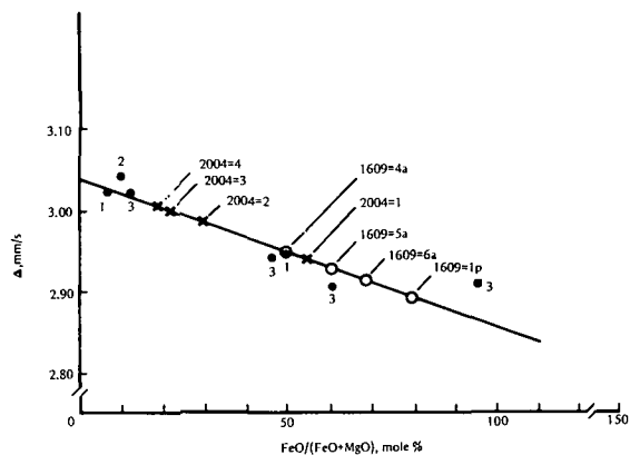
Figure 3.—Quadrupole splitting as a function of iron content of olivine, f = \frac{\text{FeO}}{\text{FeO} + \text{MgO}} mole %. Point 1 is from reference 3, point 2 is from reference 4, and point 3 is from reference 5. Luna 20 regolith specimens, 2004-4, 2004-3, 2004-2, and 2004-1 have grain sizes 0.250–0.400, 0.127–0.250, 0.083–0.127, and \leq 0.083 mm, respectively. Luna 16 regolith samples, 1609-4a, 1609-5a, 1609-6a, and 1609-1p have grain sizes 0.250–0.400, 0.127–0.250, 0.083–0.0127, and \leq 0.083 mm, respectively.
