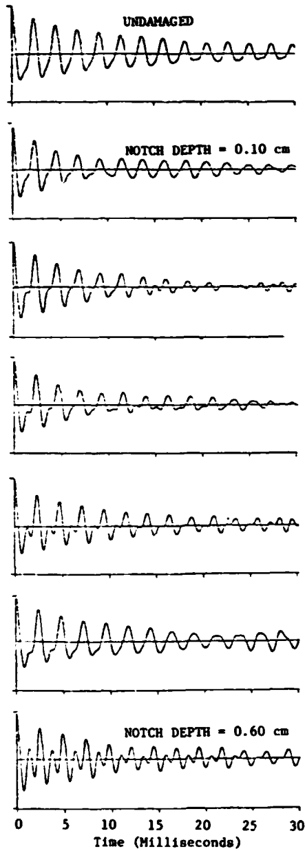
Figure 10. Damage Effects on Signature of Beam 3 Broadband Response
