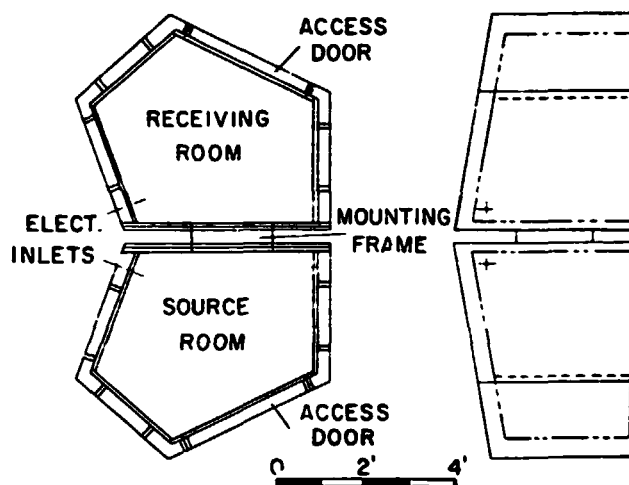
Fig. 2. Schematic view of the twin reverberation chambers.
