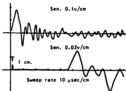
Fig. 13 Strain histories due to explosive loading on a two-inclusion steel-brass specimen, 0^\circ ray.
