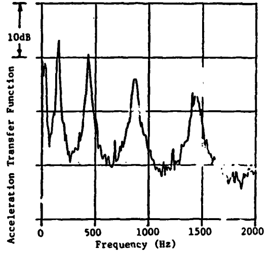
Figure 7. Typical Transfer Function Plot
