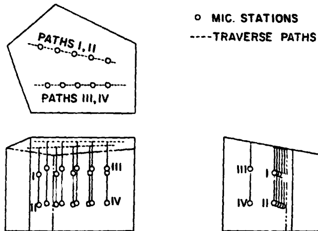
Fig. 3. Microphone traverse paths and measurement stations.
