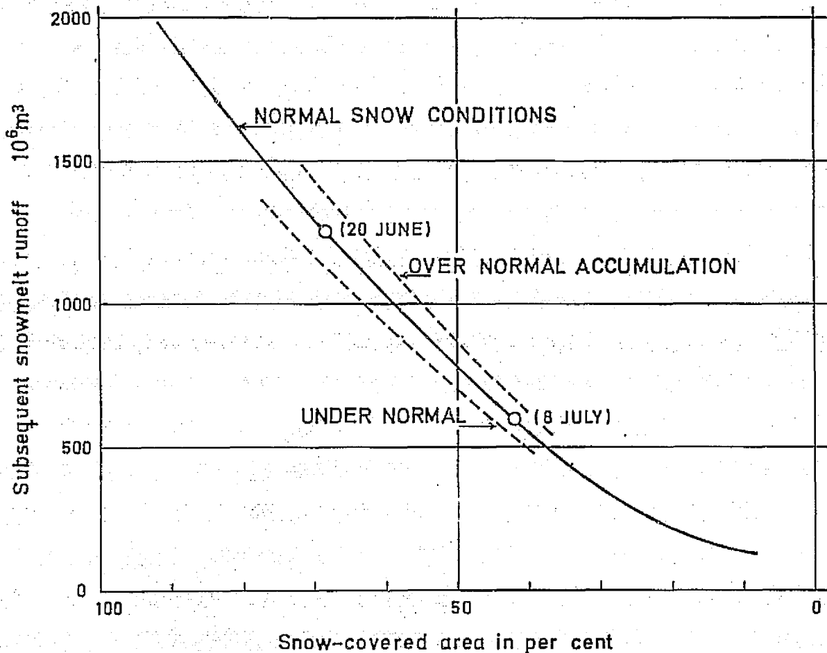
Fig. 10 The catchment basin for a relatively large power plant in Northern Norway (Røssåga) has been studied in some detail. Its total area is 1935 \text{ km}^2 , almost entirely above the tree line.
