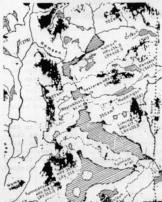
Fig. 7 A catchment area draining to the river Namsen is shown on the map. Overlays were produced from three LANDSAT passes, viz.
