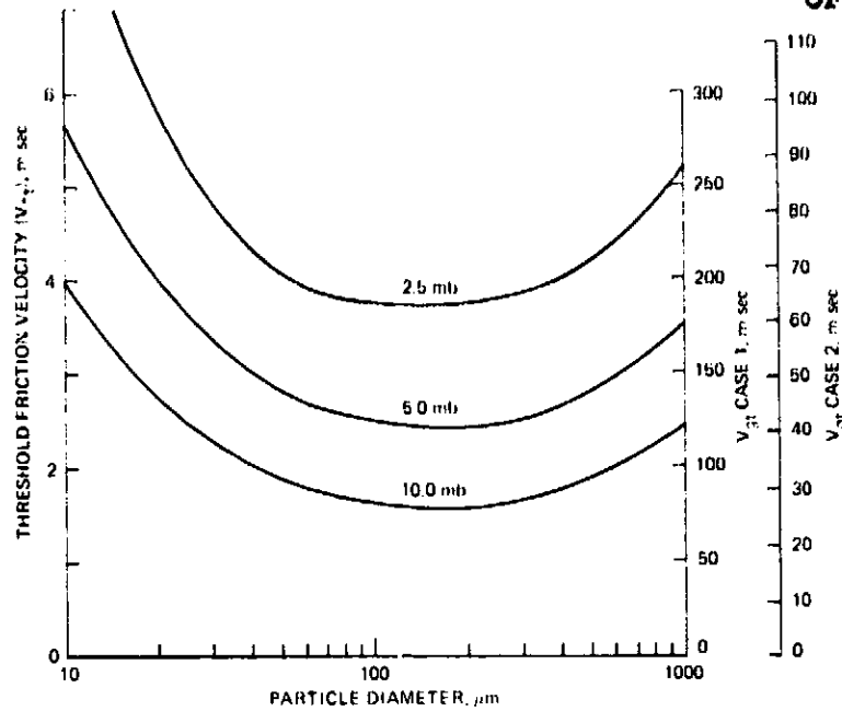
Figure 16.— Martian particle threshold curves as a function of particle size at three pressures. Scale on left is V_{*} in m/sec, two scales on right are equivalent free-stream (above the boundary layer) wind velocities ( V_{gt} ), based on atmospheric models by Pollack et al. (refs. 16 and 17). Case 1 is for winds blowing over a flat smooth surface composed of erodible grains; Case 2 is for a surface containing cobbles and small boulders.
