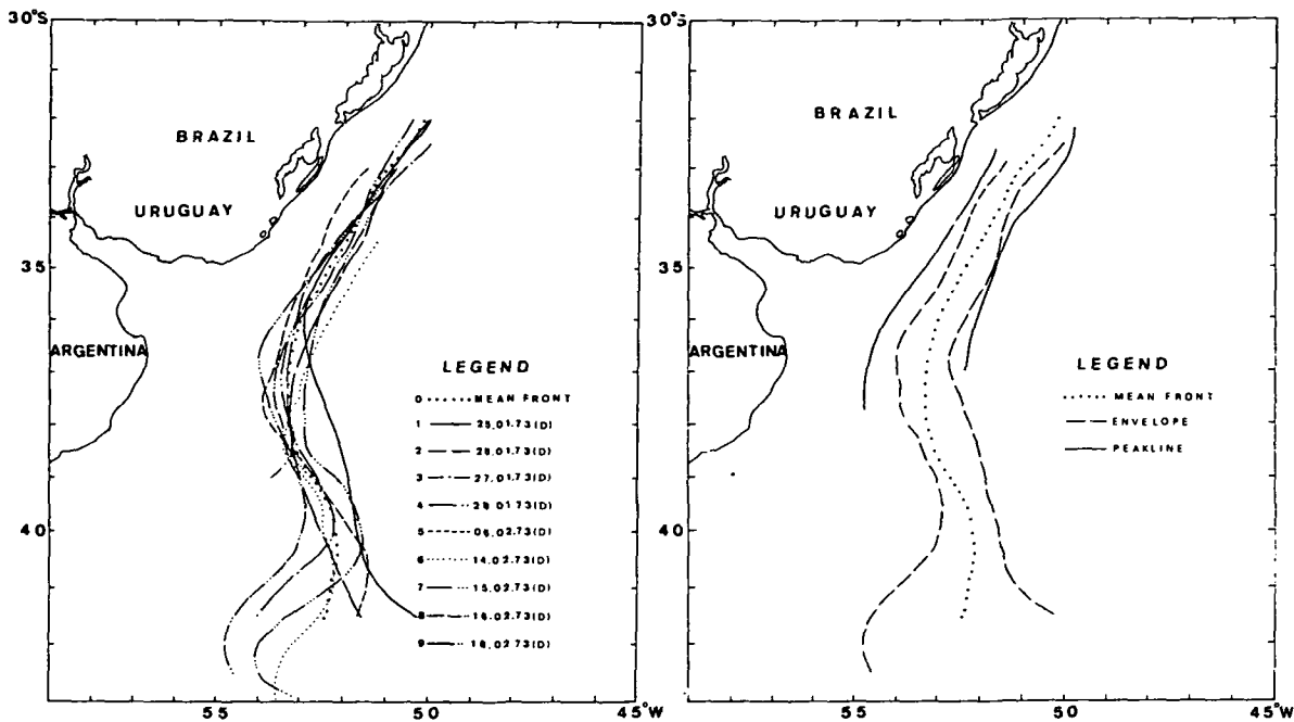
FIG. III.1 - FRONT LINES OF SUMMER SECOND PERIOD OF 1973.
