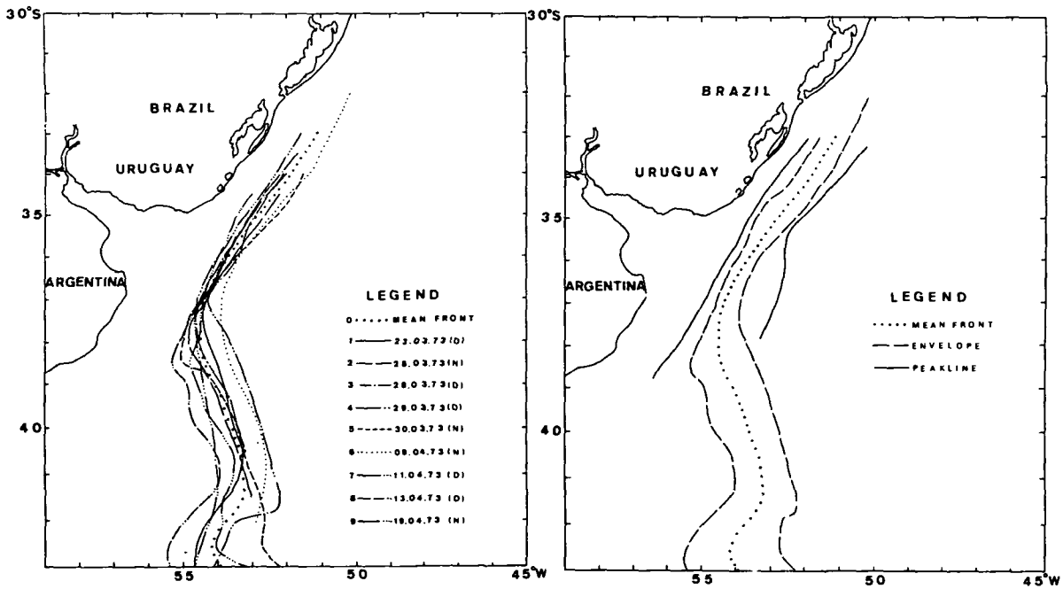
FIG. III.3 - FRONT LINES OF AUTUMN FIRST PERIOD OF 1973.
