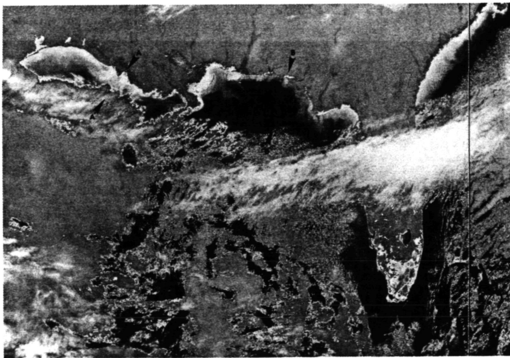
FIGURE 5. NOAA-5 INFRARED IMAGE, ORBIT 2134, 18 JANUARY 1977, 0204Z. Sharp thermal gradient formed off Florida coast as a result of heat loss by the shallow water column. Continuation of offshore cooling.
