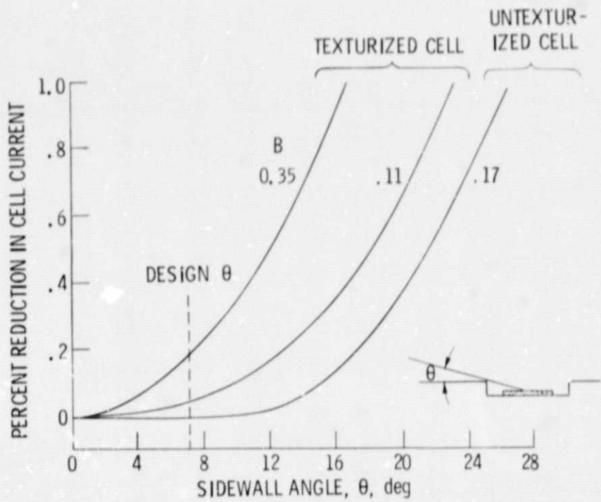
Figure 1. - Reduction in cell current due to sidewall shadowing.
