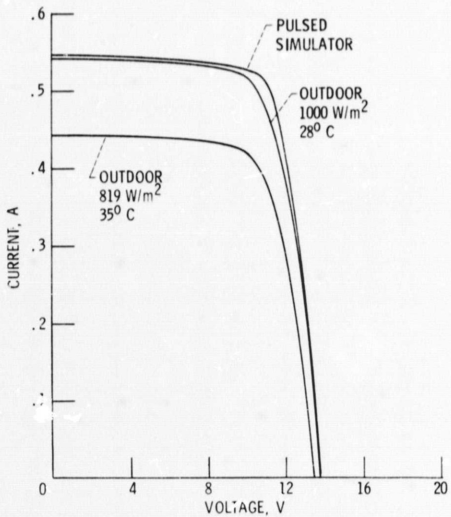
Figure 9. - Comparison of indoors-outdoors I-V measurements.
