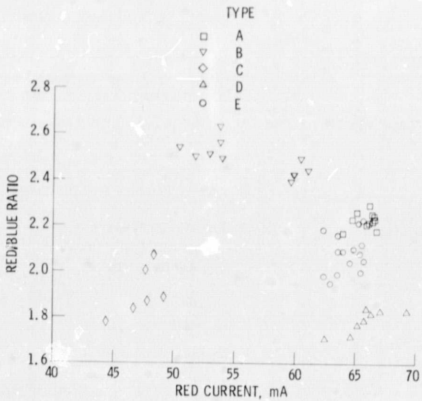
Figure 8. - Distribution of red/blue ratios of typical cells.
