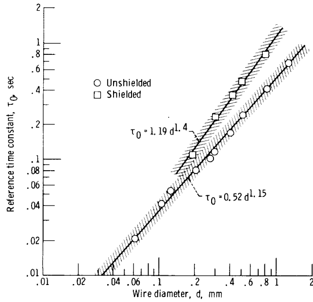
Figure 13. - Reference time constant as function of wire diameter for unshielded and shielded thermocouple probes.
