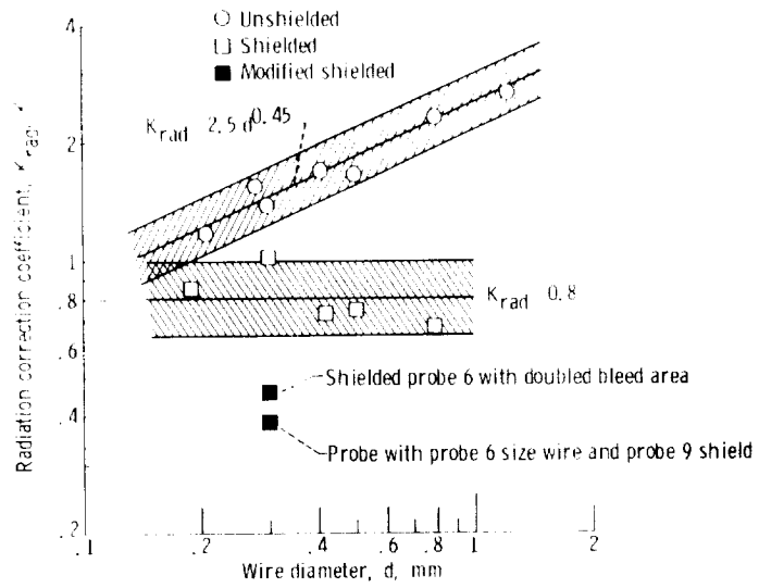
Figure 14. - Radiation correction coefficient as function of wire diameter for shielded and unshielded probes.
