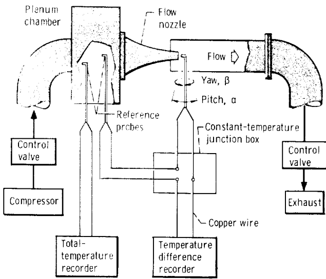
Figure 4. - Recovery test apparatus.
