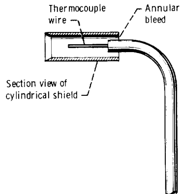
Figure 15. - Head detail of proposed shielded-probe design with annular bleed.
