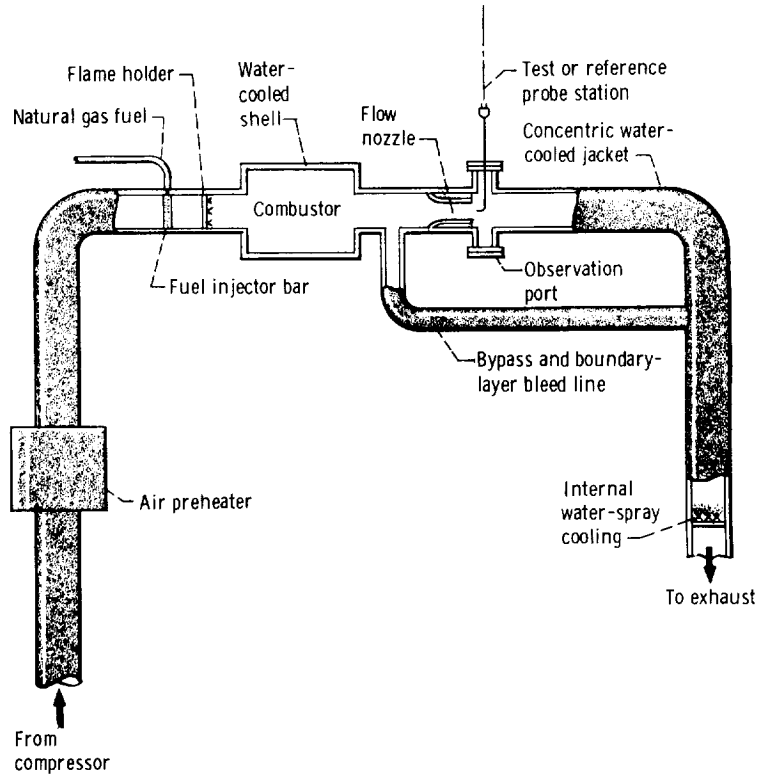
Figure 6. - High-temperature tunnel.
