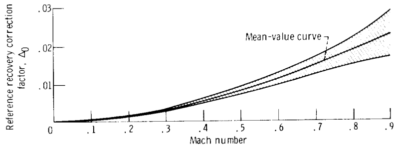
Figure 7. - Reference recovery correction factor as function of Mach number for unshielded wedge-type thermocouple probes.
