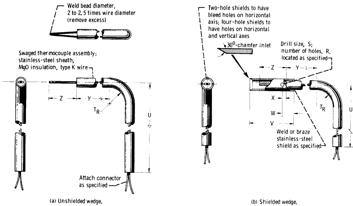
Figure 1. - Design details of shielded and unshielded thermocouple probes. (Probes subjected to high humidity should be baked at 425 K for 4 hr and a sealant applied to insulation at each end of swaged assembly.)
