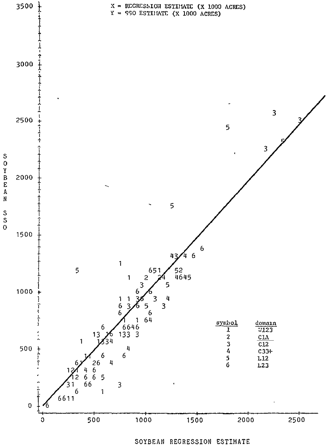
Figure 6. Comparison of regression and SSO county estimates for soybeans.
