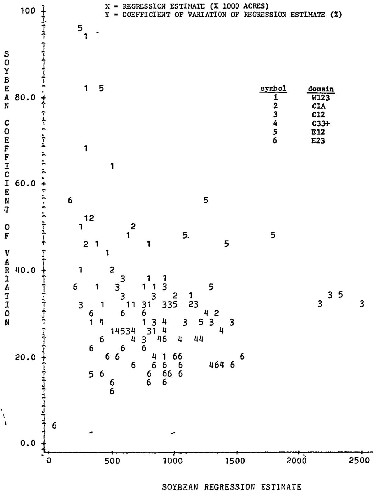
Figure 11. Coefficient of variation of regression estimates as a function of the regression estimates for soybeans in individual counties.
