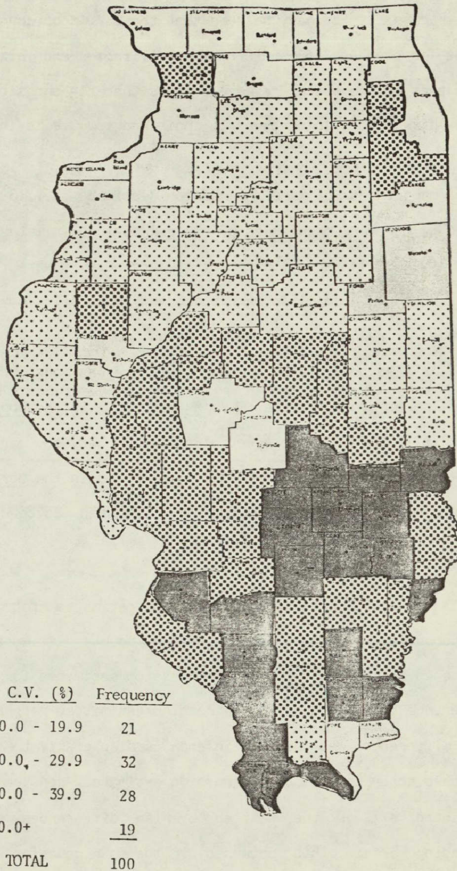
Figure 9. Distribution of Coefficients of Variation (C.V.'s) of County Regression Estimates for Soybeans
