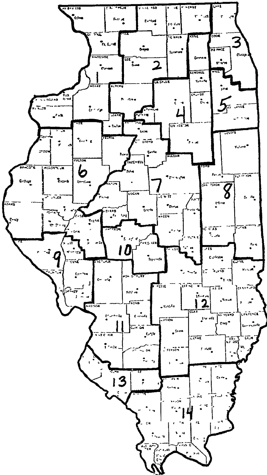
Figure 2. Analysis Districts for 1975 Illinois Acreage Estimation Project.
