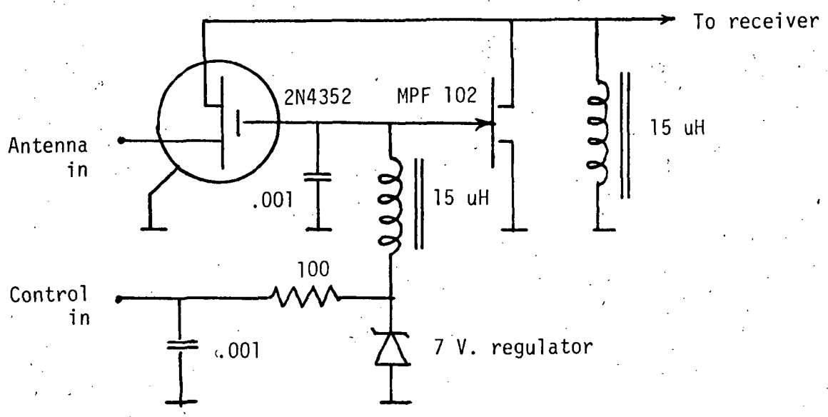
Fig 15 Antenna switch
