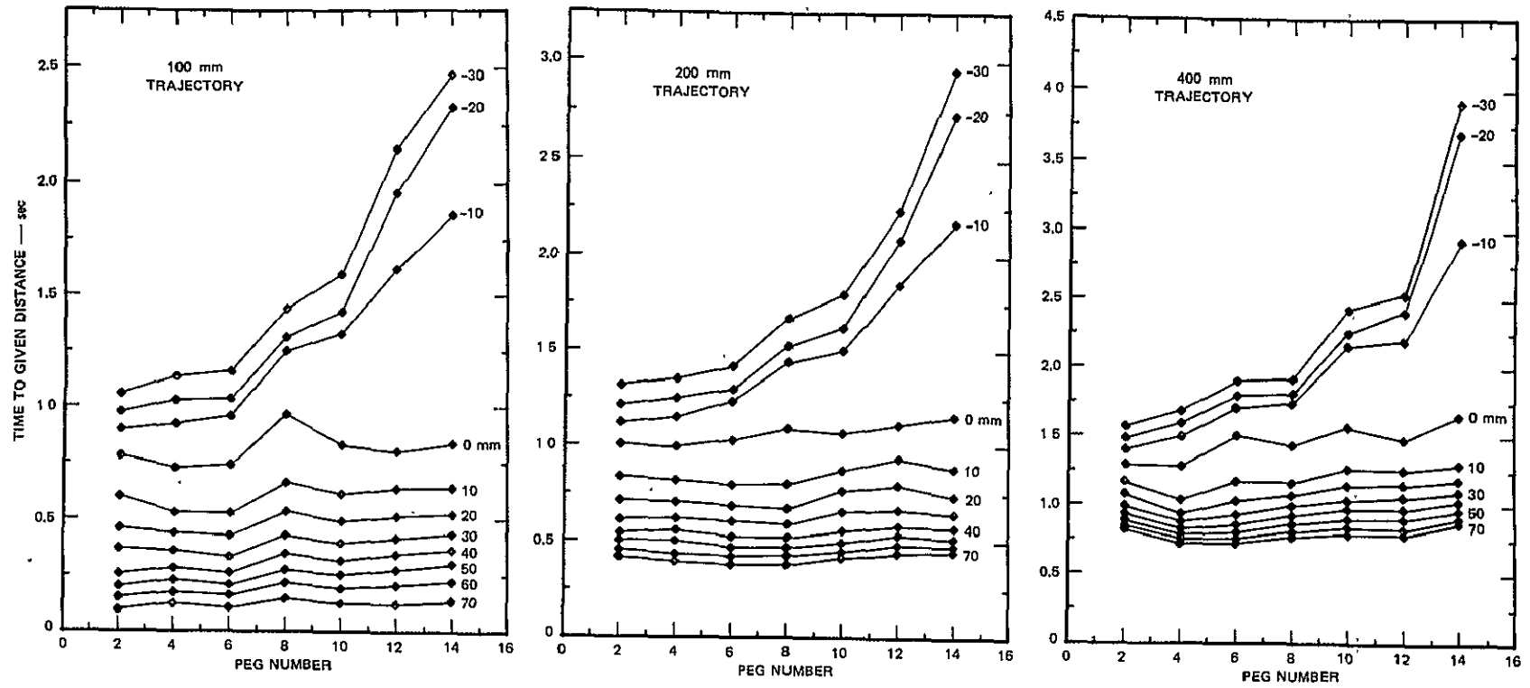
FIGURE 19 MA-11 APPROACH TIMES FOR DIFFERENT DISTANCES TO THE RECEPTACLE
