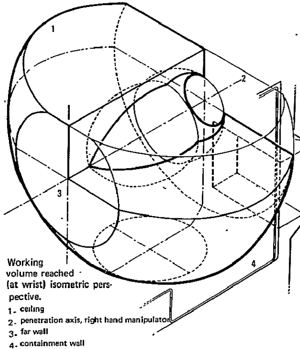
FIGURE D-1 DESCRIPTION OF MA-11 (Concluded)
