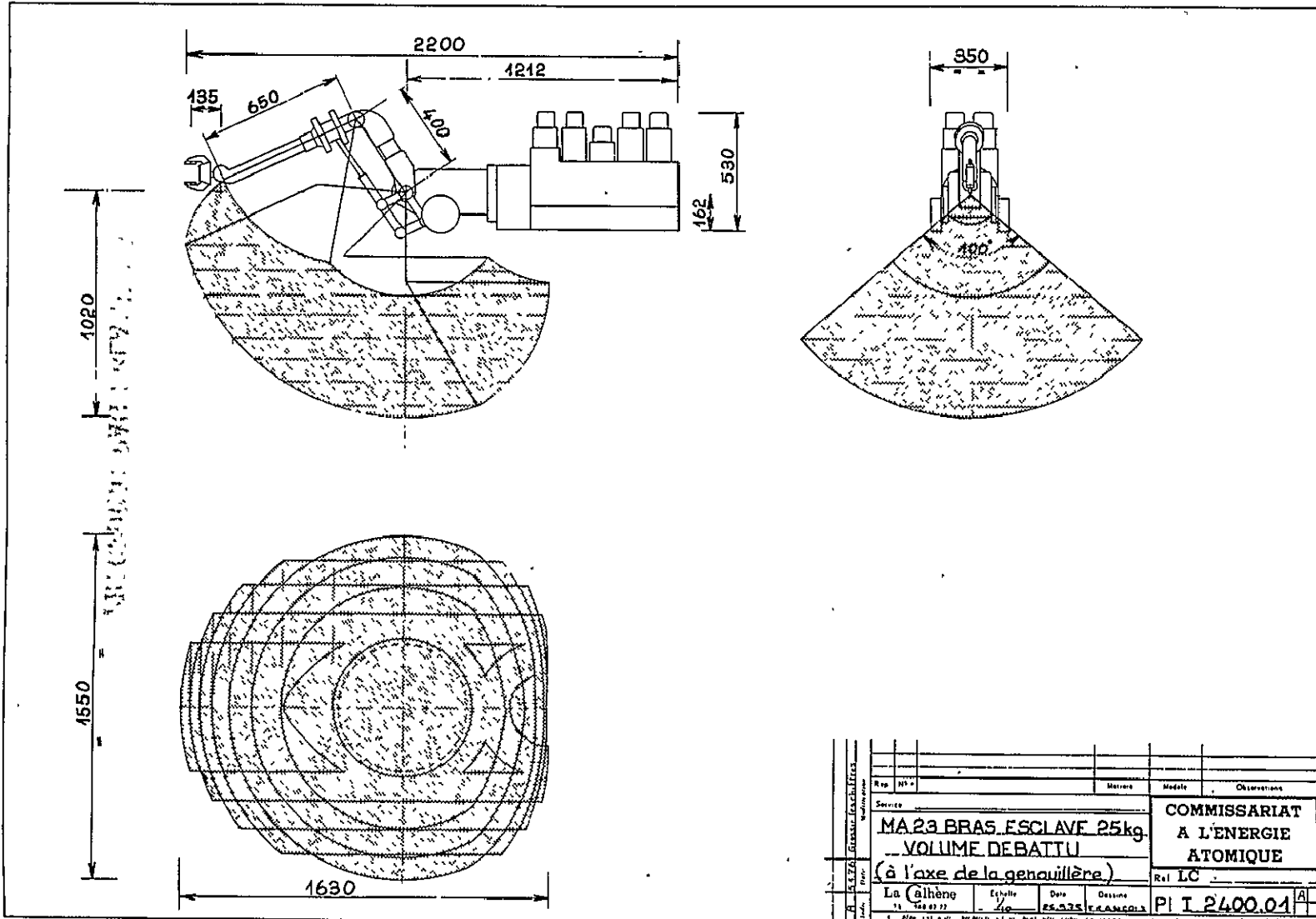
FIGURE E-1 MA-23 SLAVE WORKING VOLUME (25 kg)
