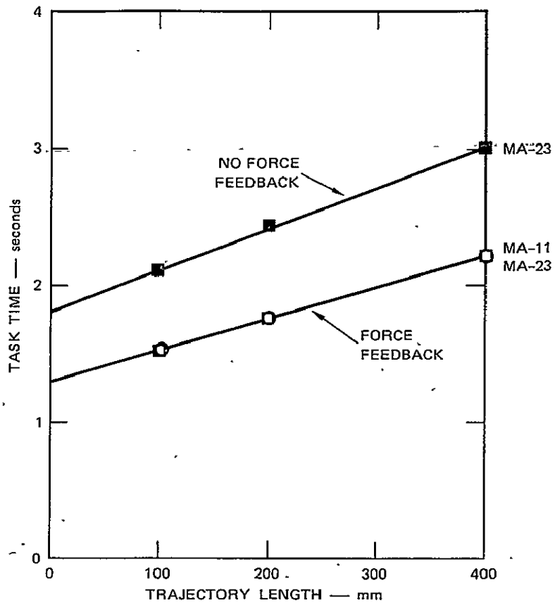
FIGURE 11 AVERAGE TASK TIME VERSUS TRAJECTORY LENGTH
