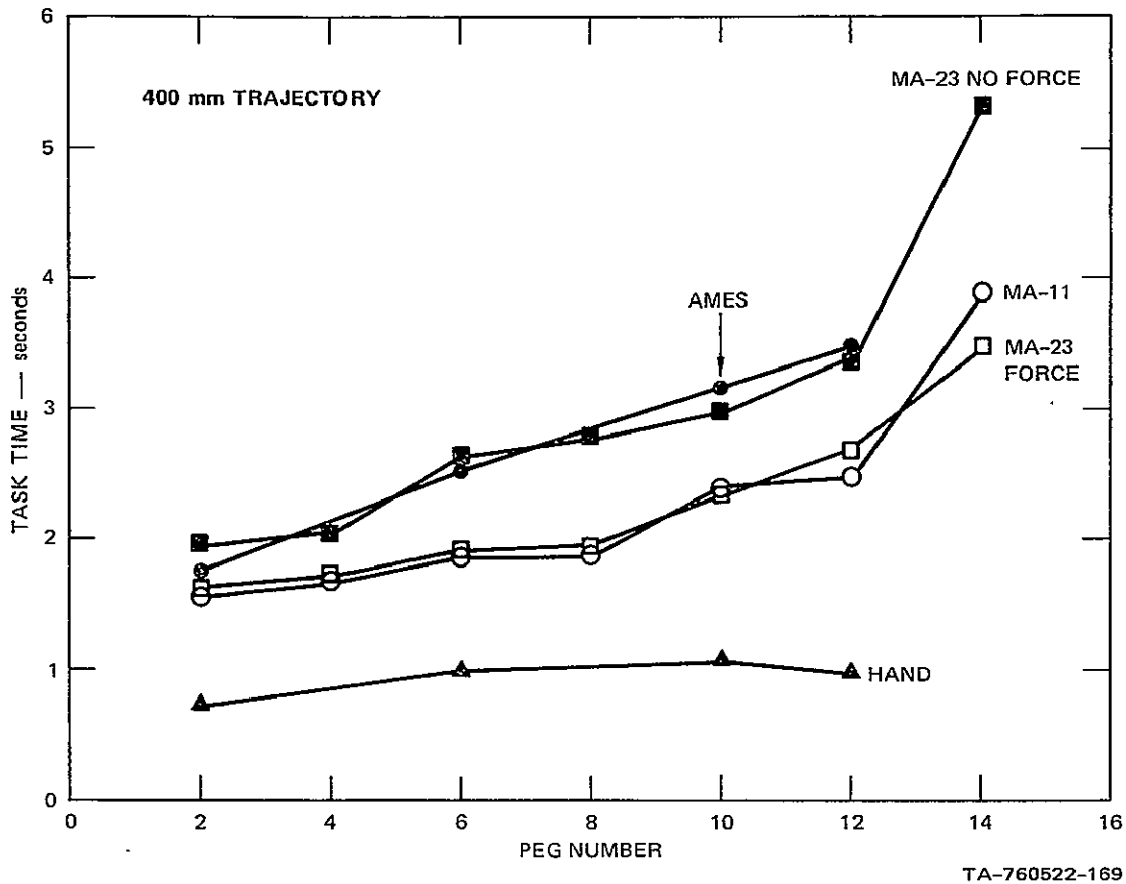
FIGURE 10 TASK TIMES FOR FIVE DIFFERENT PEG-IN-HOLE EXPERIMENTS
