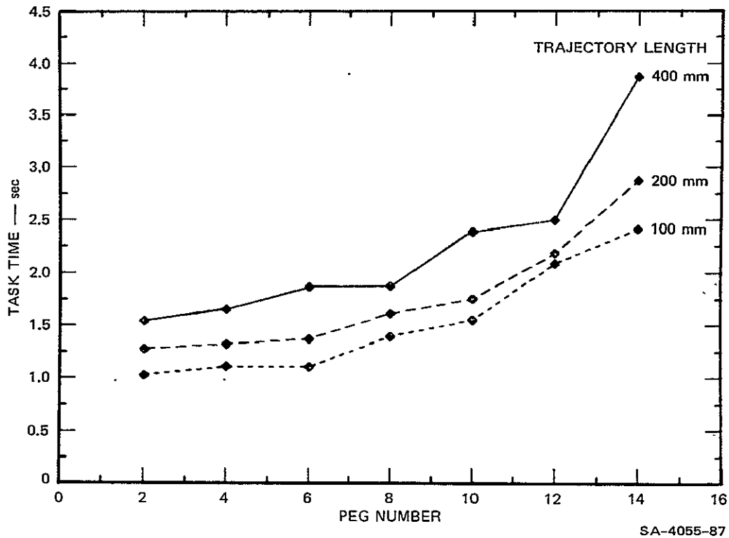
FIGURE 6 MA-11 TASK COMPLETION TIMES
