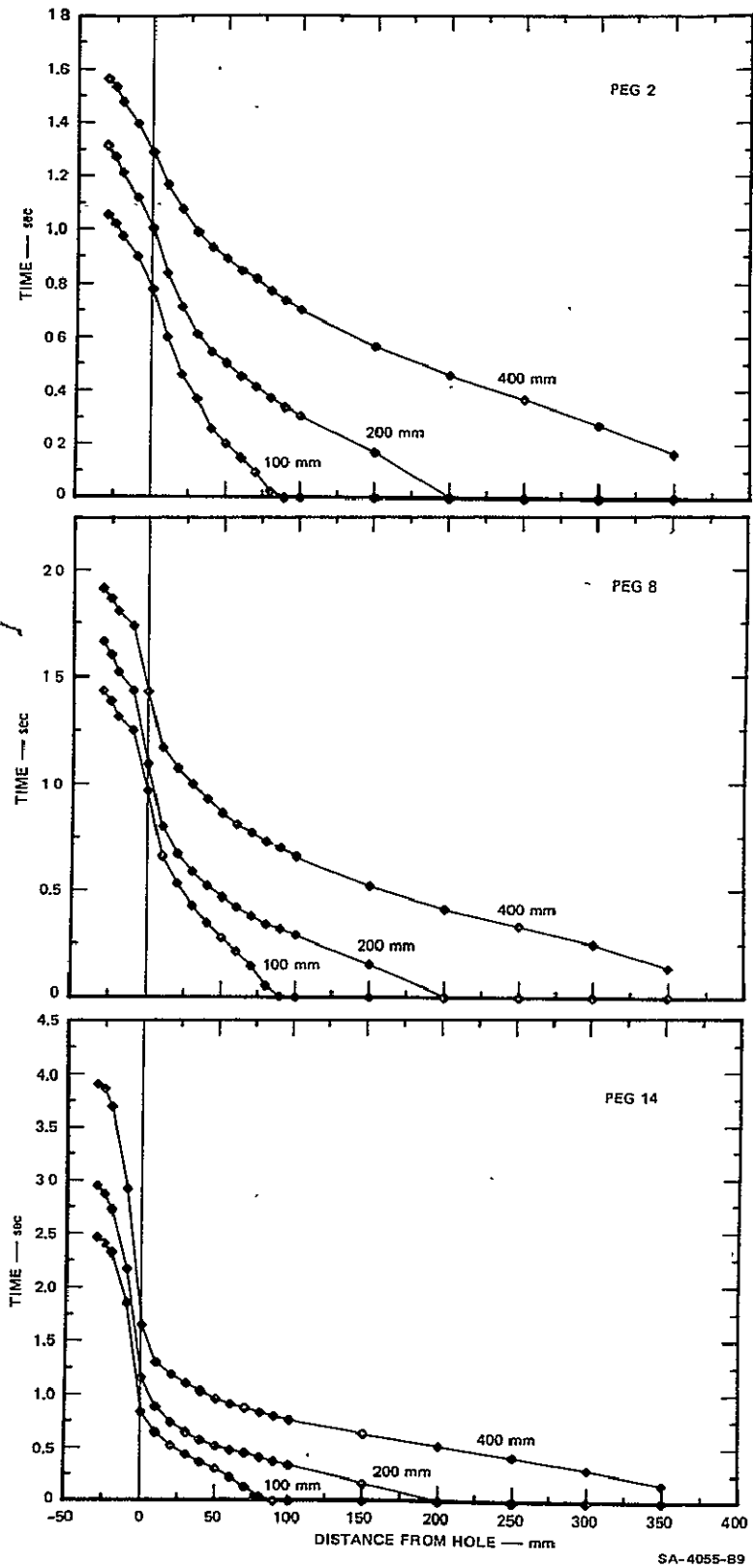
FIGURE 7 MA-11 TRAJECTORIES WITH INCREASINGLY DIFFICULT PEGS
