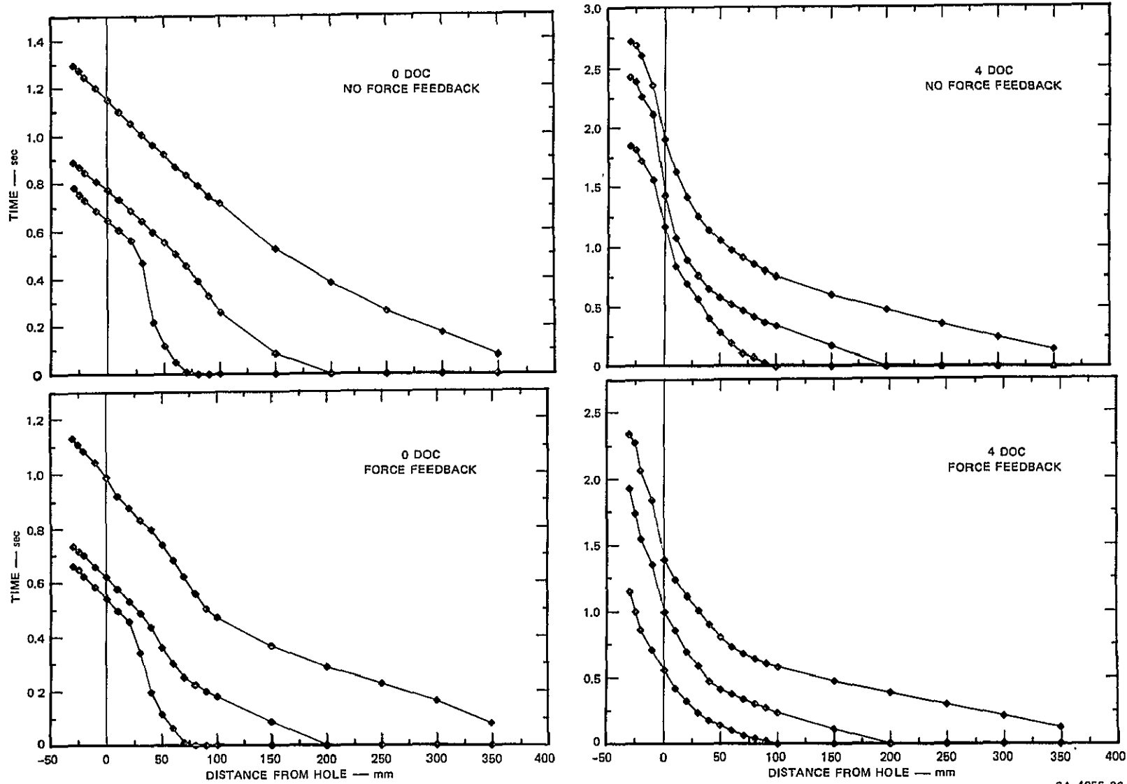
FIGURE 17 COMPARISON OF MA-23 TRAJECTORIES WITH AND WITHOUT FORCE FEEDBACK
