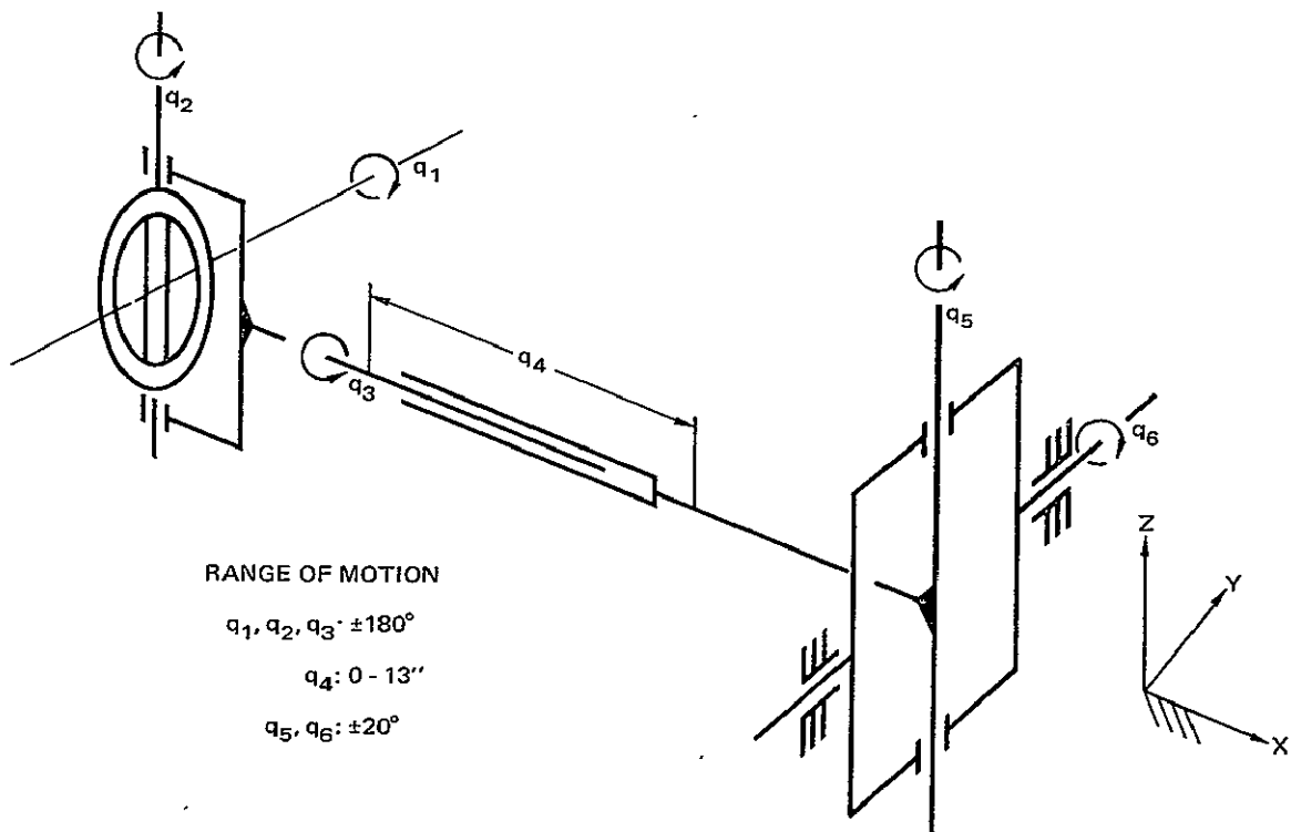
FIGURE 29 CONTROLLER KINEMATICS
