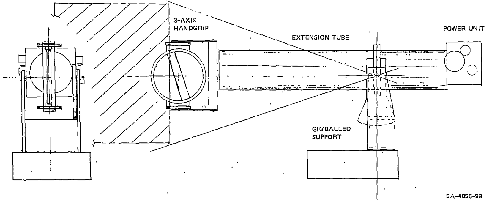
FIGURE 28 SIX-AXIS, FORCE-REFLECTING CONTROLLER
