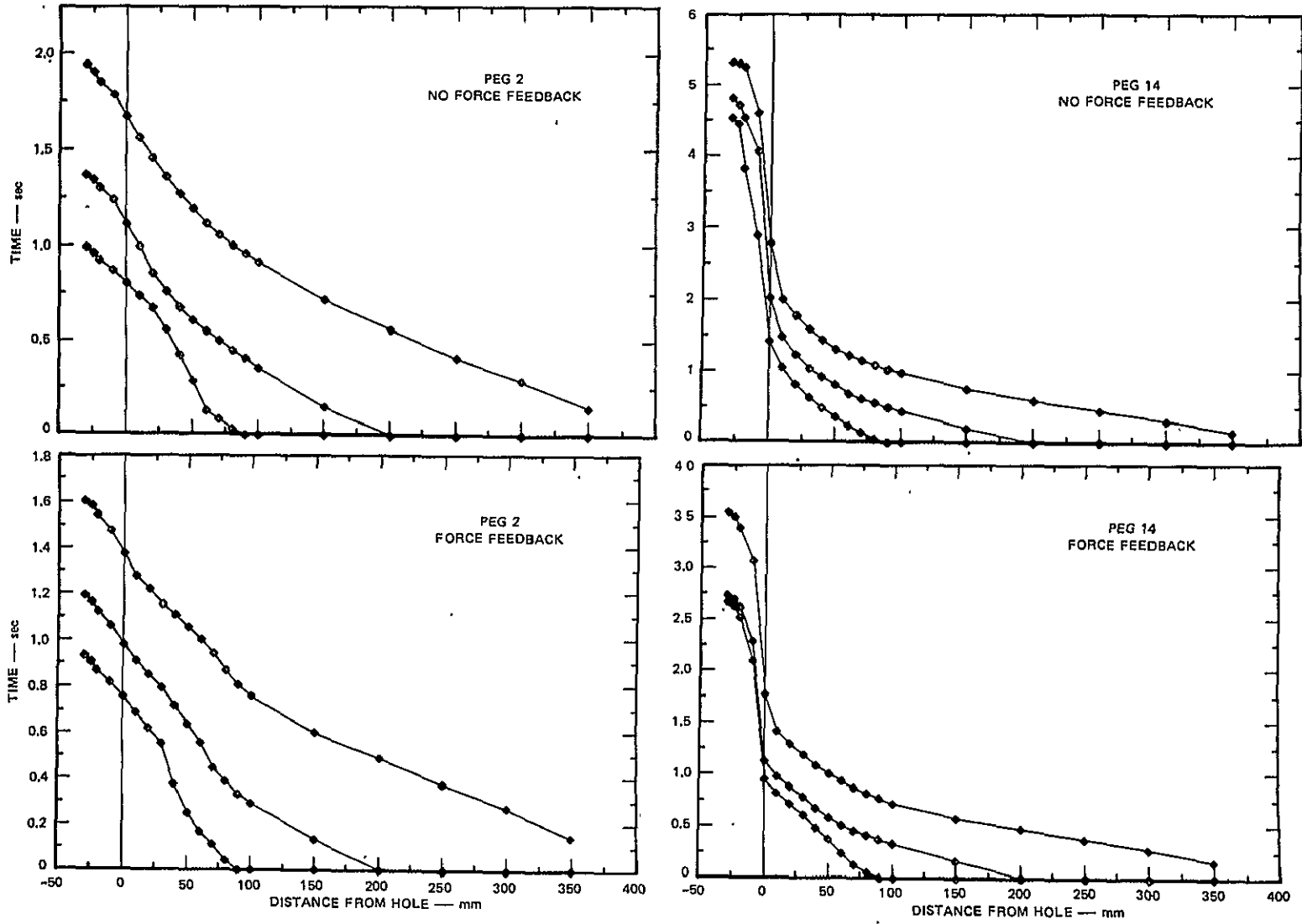
FIGURE 23 COMPARISON OF MA-23 TRAJECTORIES WITH AND WITHOUT FORCE FEEDBACK
