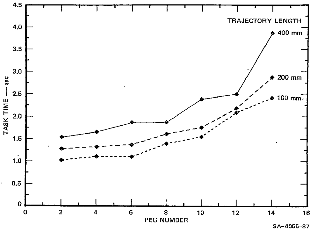
FIGURE 18 MA-11 TASK COMPLETION TIMES
