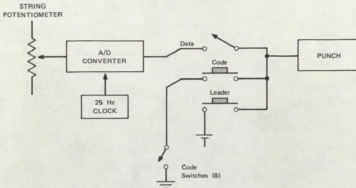
FIGURE 5 BLOCK DIAGRAM OF DATATAKER
