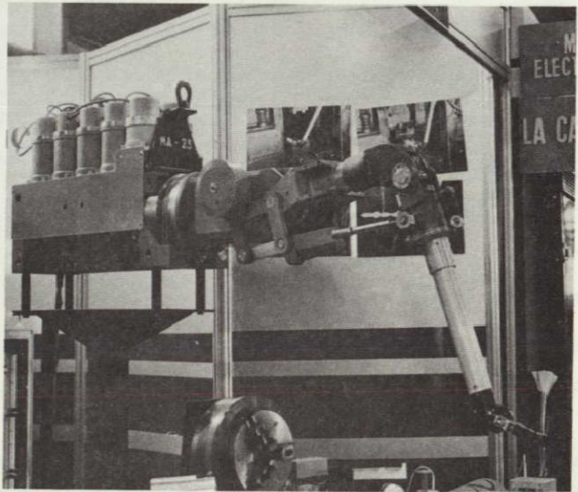
(b) MA-23/200 HEAVY DUTY SLAVE (25 kg)
