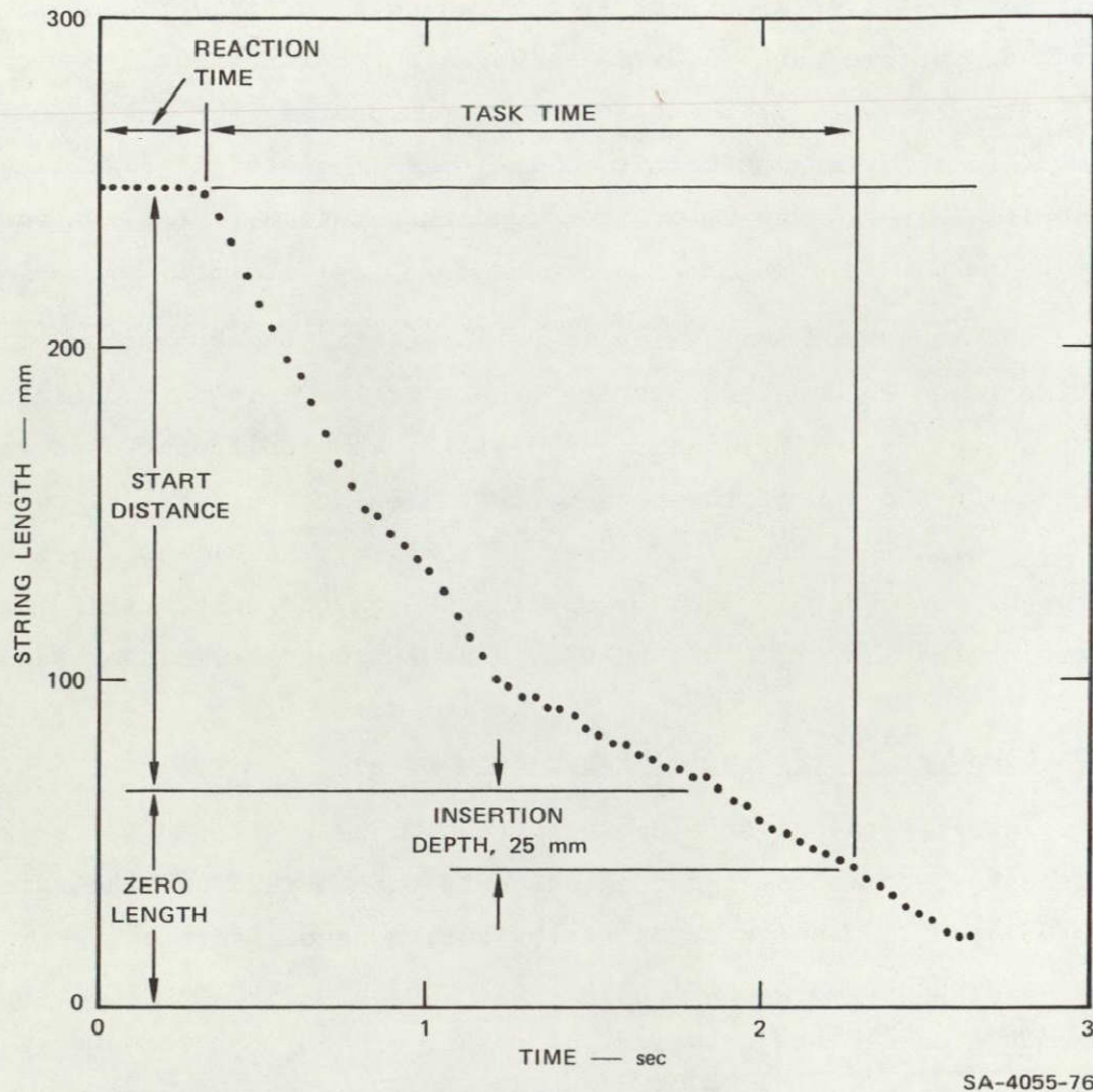
FIGURE 6 SAMPLE TRAJECTORY MEASURED BY DATATAKER
