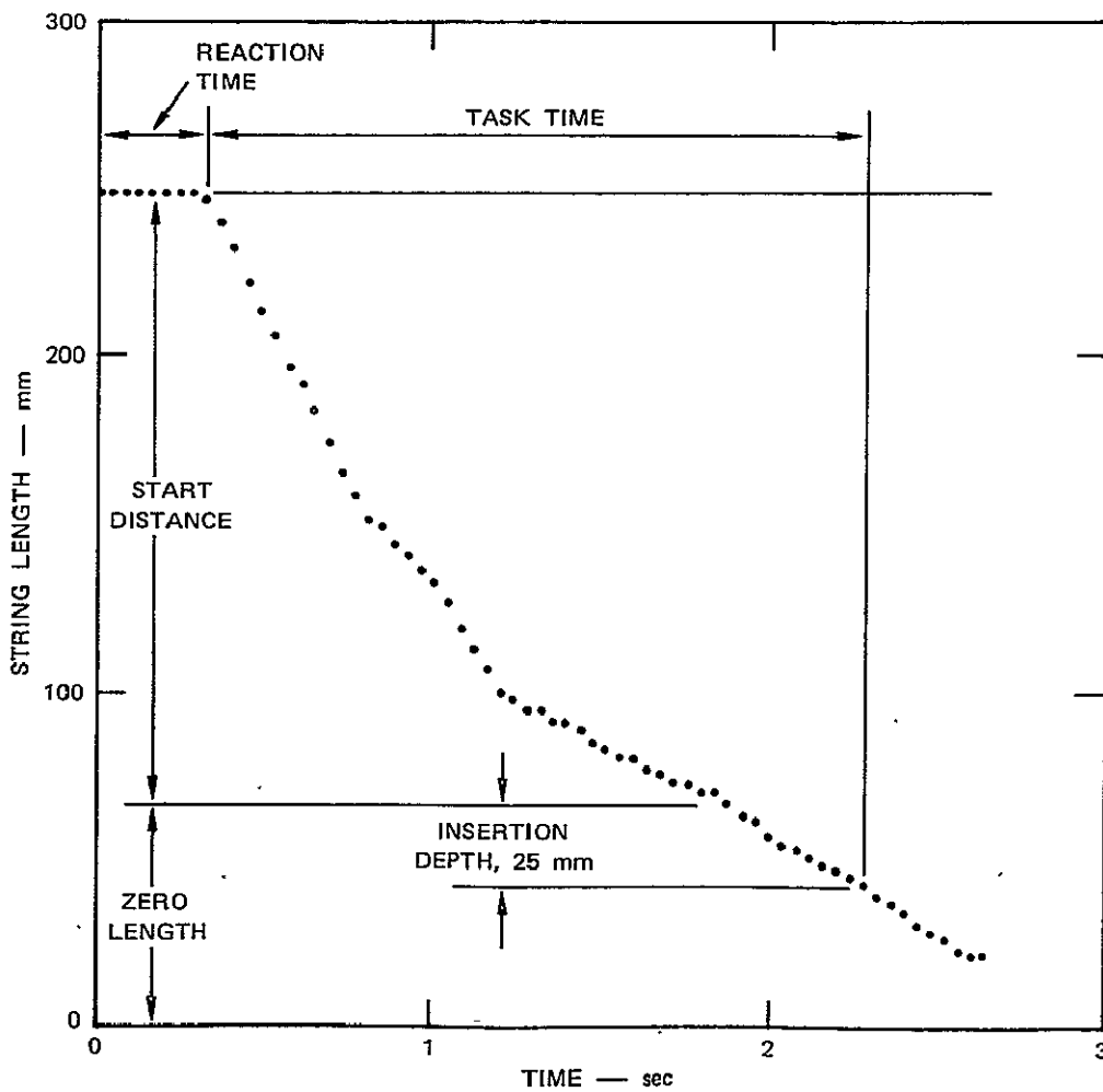
FIGURE 2 SAMPLE TRAJECTORY MEASURED BY DATATAKER
