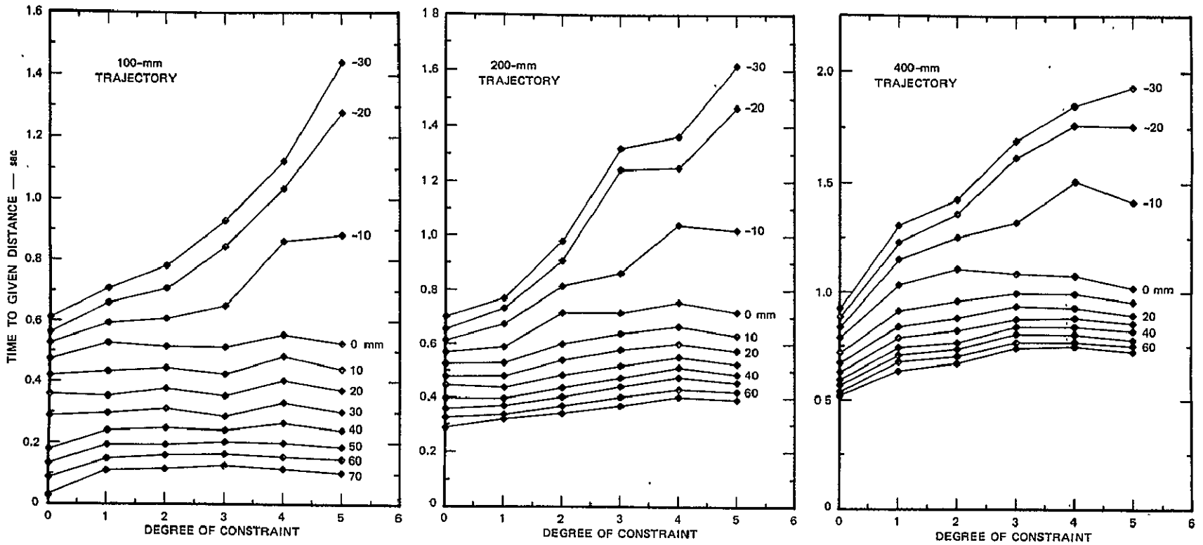
FIGURE 13 MA-11 APPROACH TIMES FOR DIFFERENT DISTANCES TO THE RECEPTACLE
