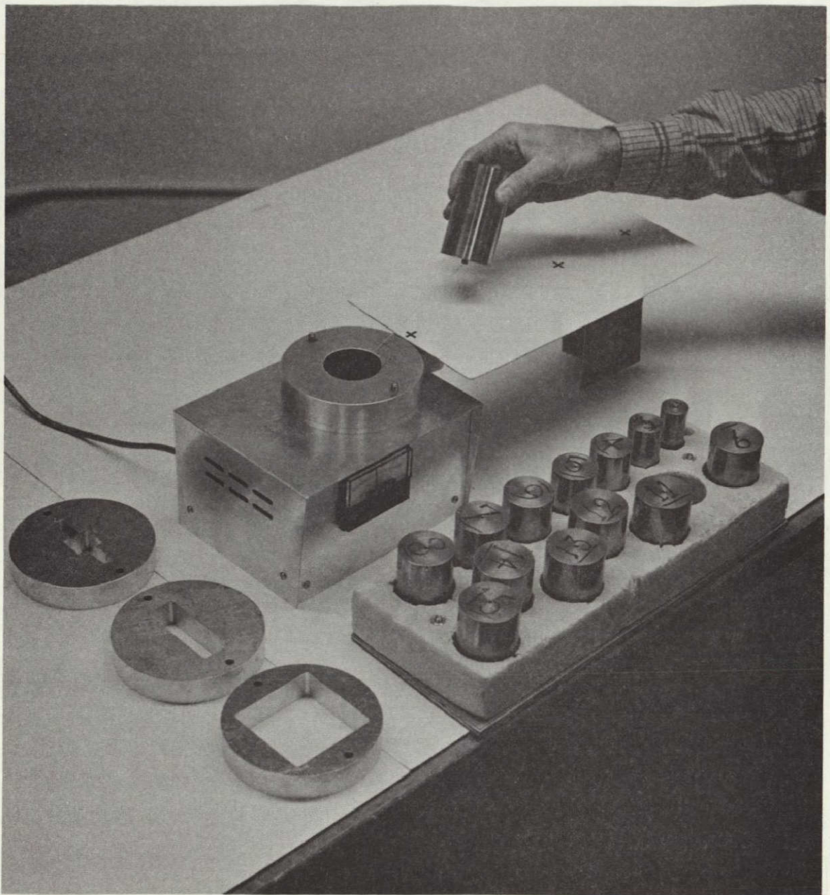
FIGURE 3 MEASURING UNIT SHOWING SET OF RECEPTACLES AND PEGS
