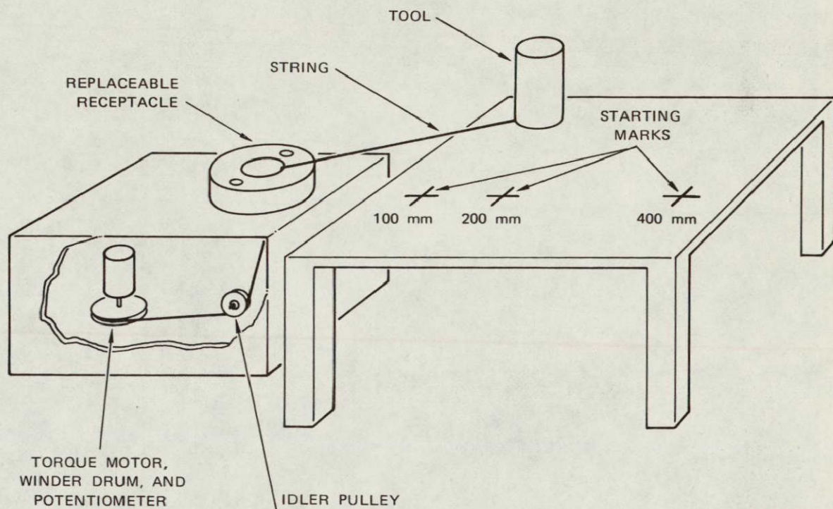
FIGURE 2 TASK CONFIGURATION WITH MEASURING UNIT AND ACCESSORY TABLE
