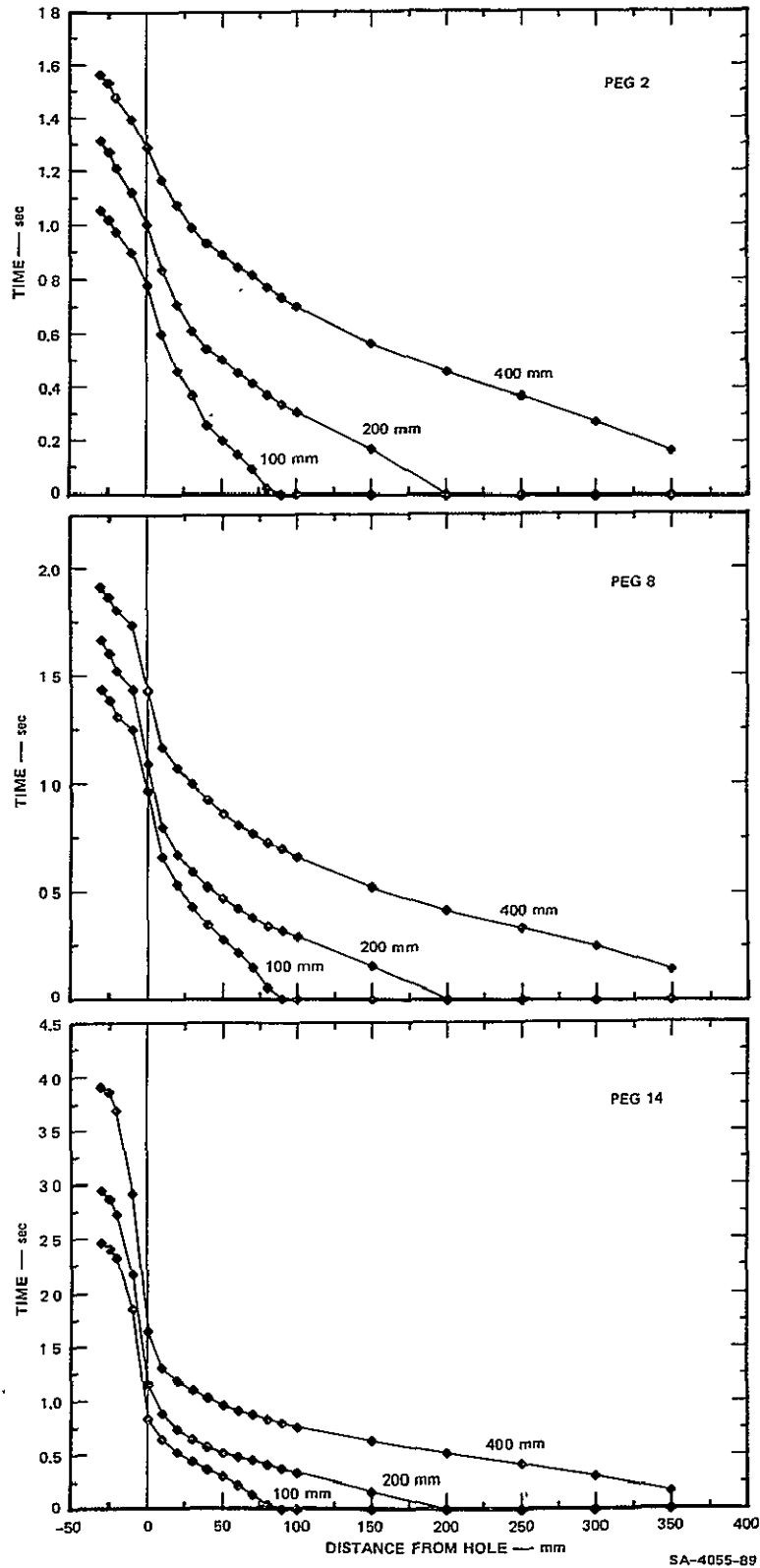
FIGURE 20 MA-11 TRAJECTORIES WITH INCREASINGLY DIFFICULT PEGS
