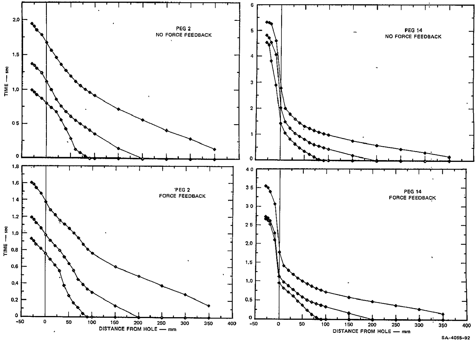
FIGURE 9 COMPARISON OF MA-23 TRAJECTORIES WITH AND WITHOUT FORCE FEEDBACK
