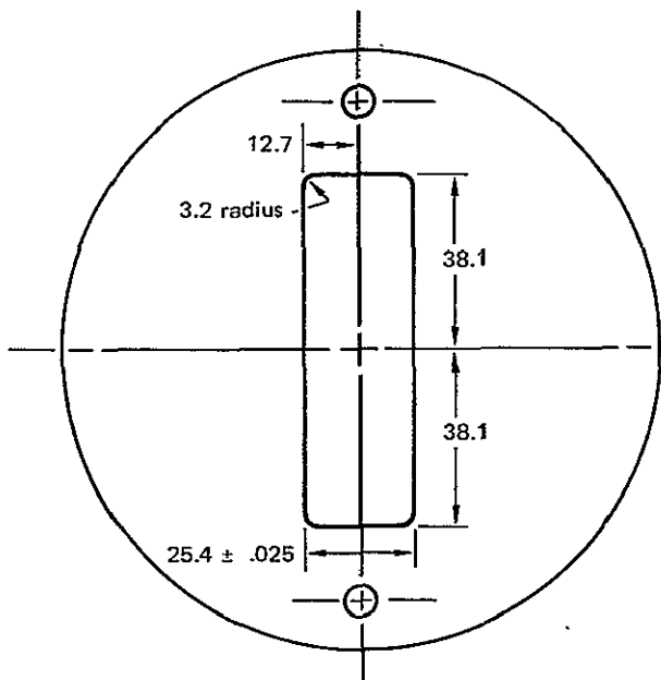
(c) RECEPTACLE 2
