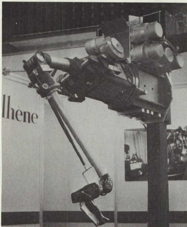
(a) MA-23 FORCE-REFLECTING MASTER (5 kg)
