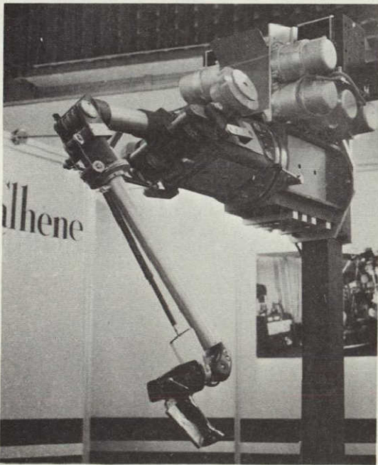
(a) MA-23 FORCE-REFLECTING MASTER (5 kg)
