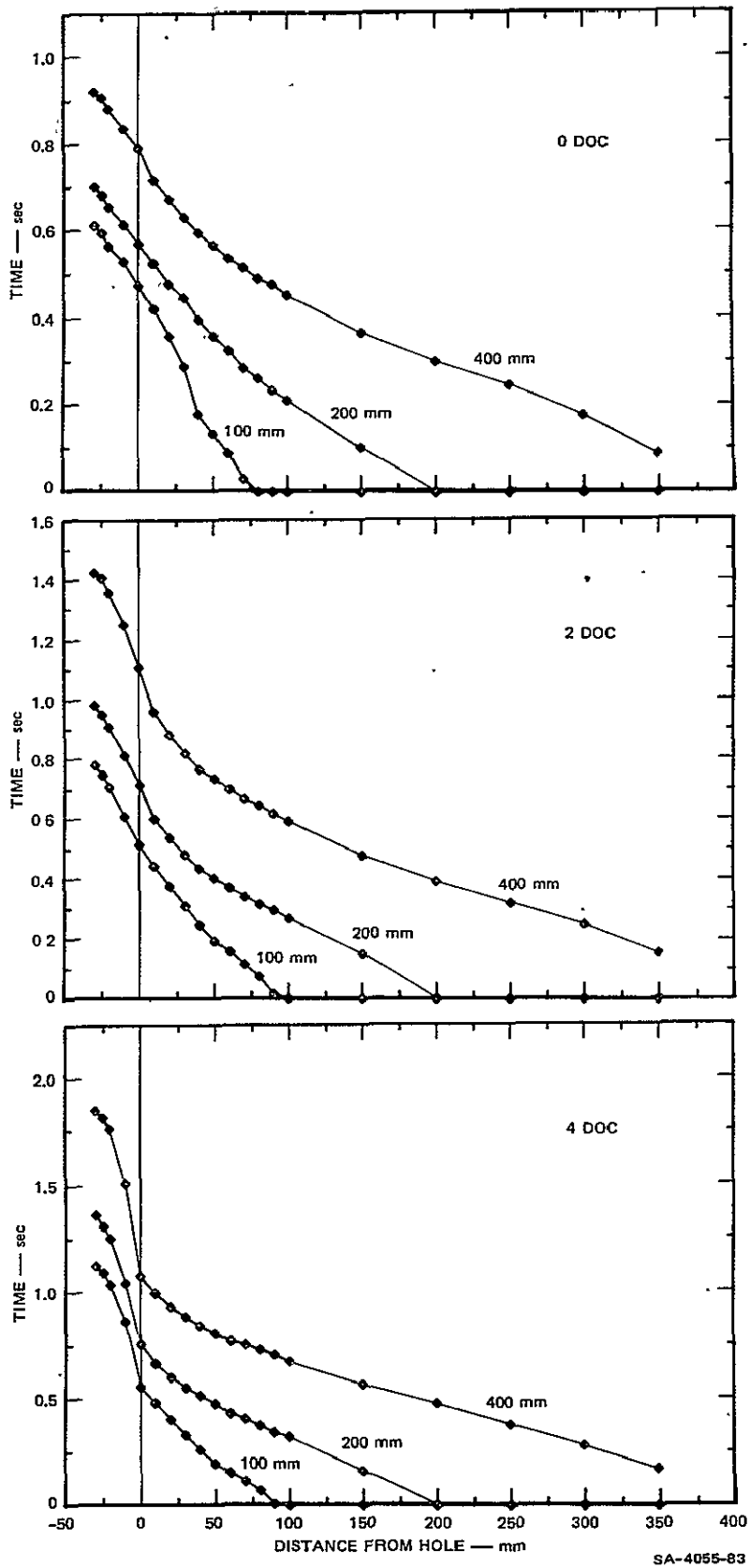
FIGURE 14 MA-11 TRAJECTORIES WITH INCREASING DEGREES OF CONSTRAINT
