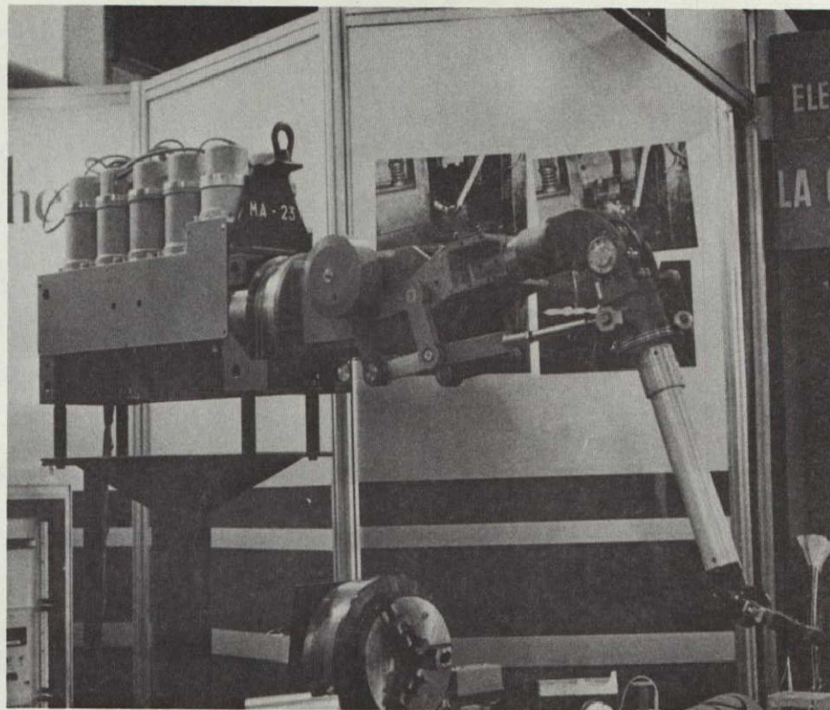
(b) MA-23/200 HEAVY DUTY SLAVE (25 kg)
