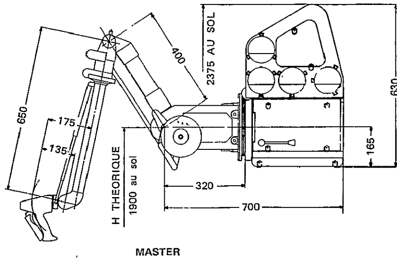
FIGURE E-2 DIMENSIONS OF THE MA-23 MASTER AND SLAVE
