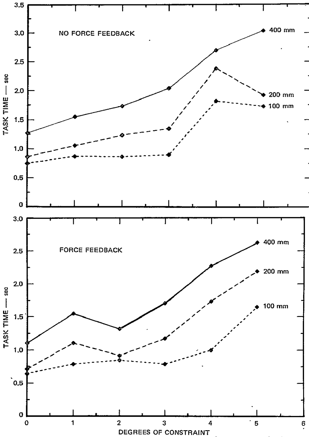
FIGURE 15 COMPARISON OF MA-23 COMPLETION TIMES WITH AND WITHOUT FORCE FEEDBACK
