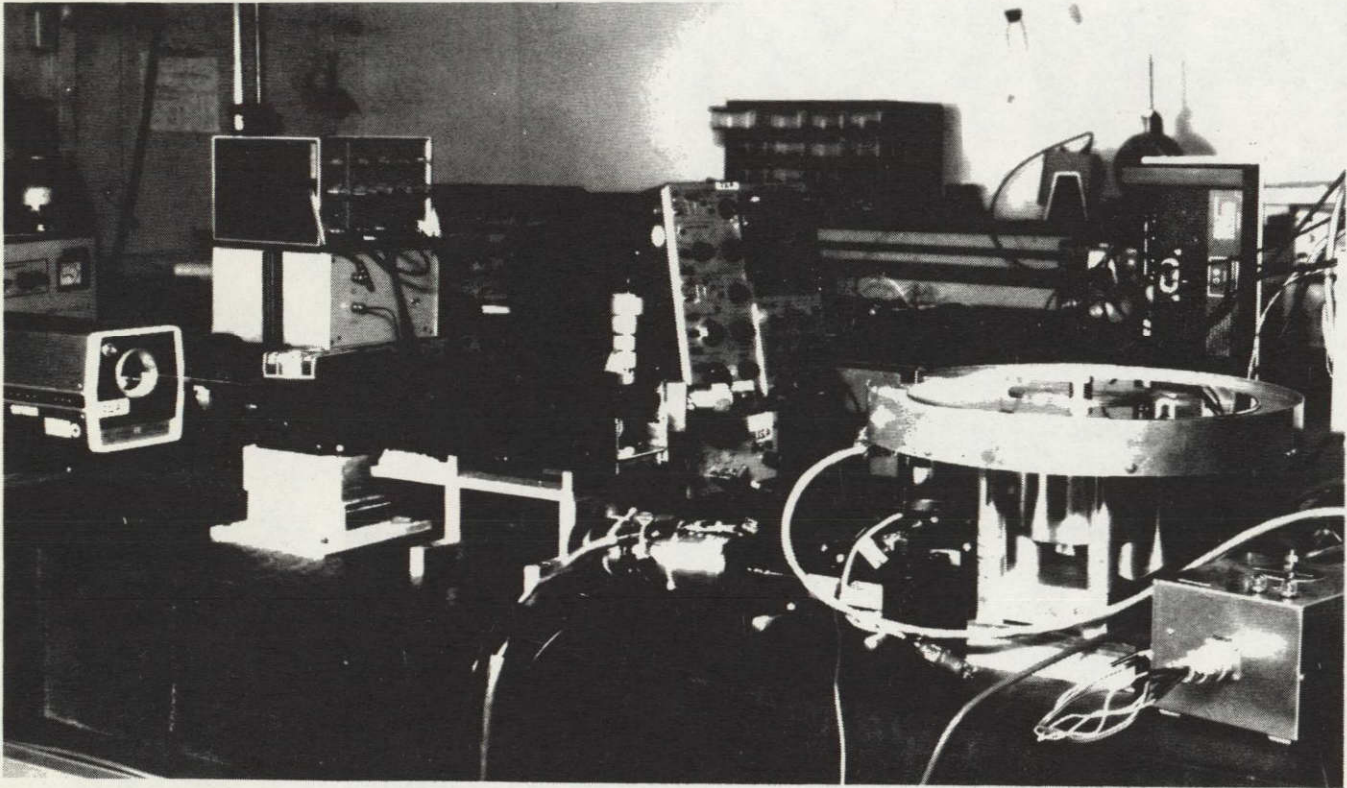
Figure 2. Experimental OVD setup.
