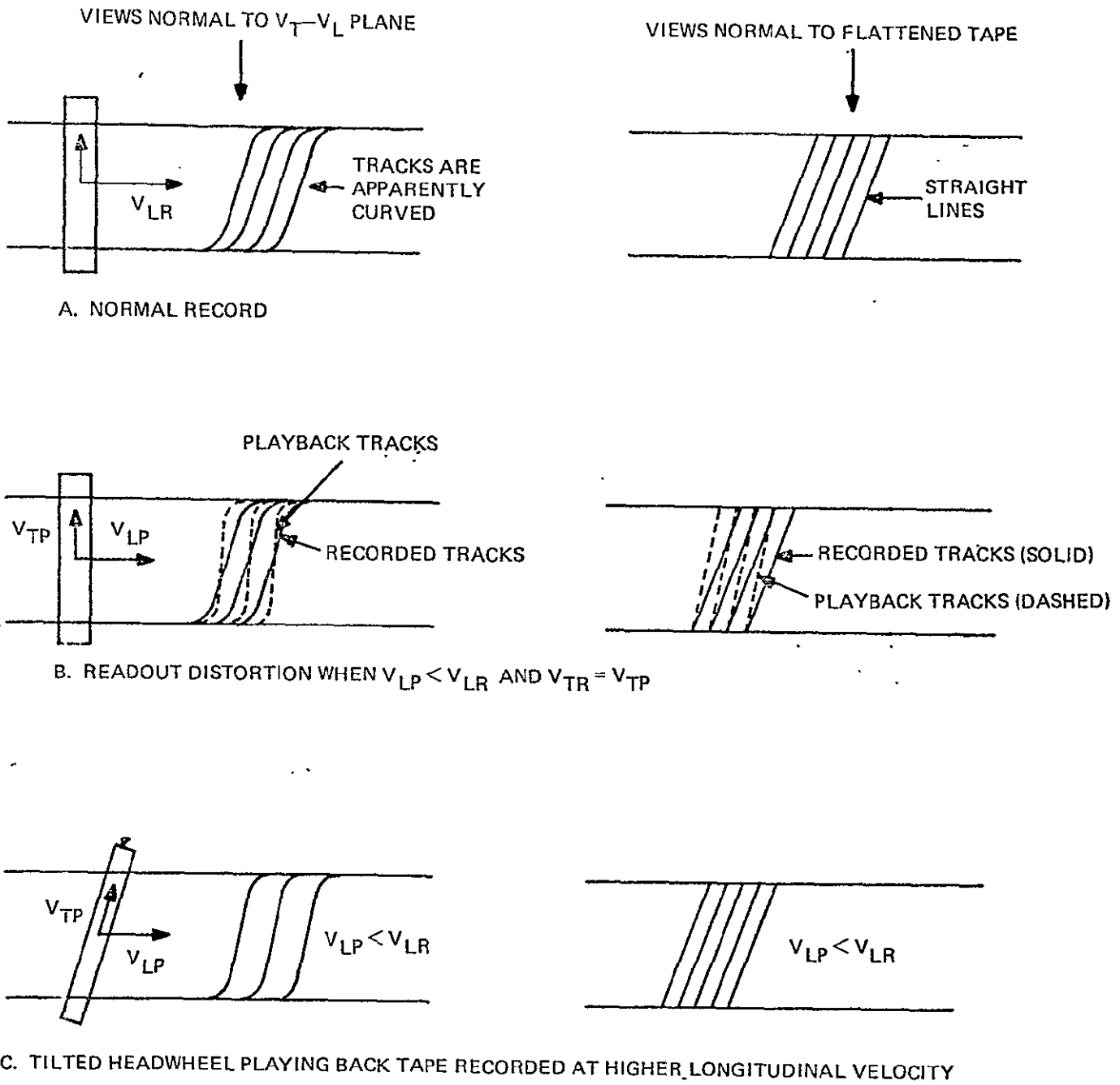
Fig. 3. Tilted Headwheel Reproduction.
