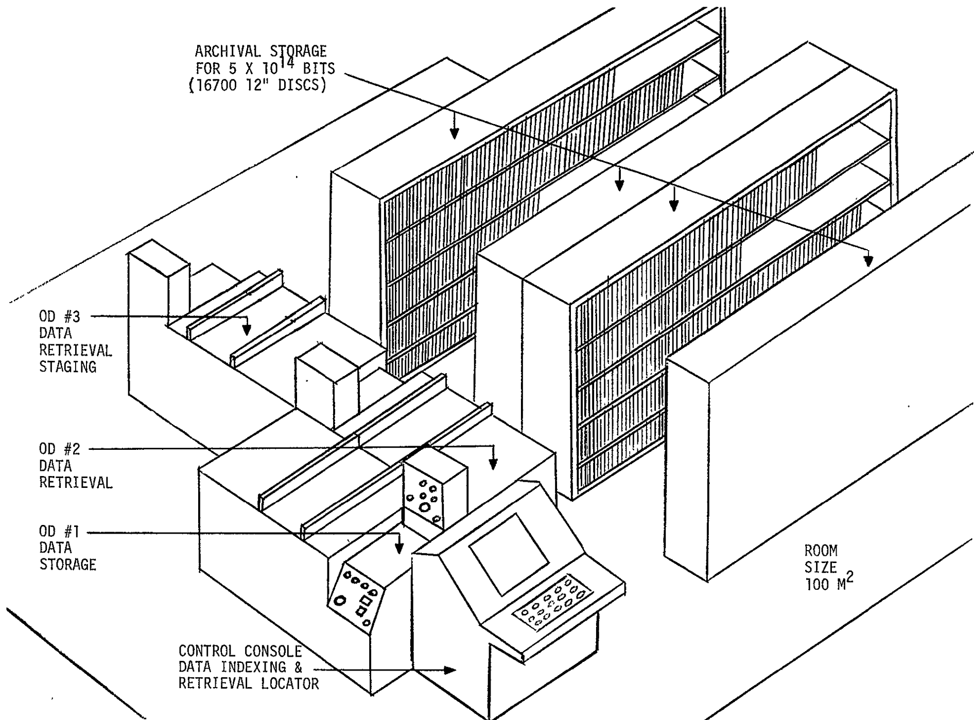
FIGURE 6 - 3 ARCHIVAL DATA STORAGE SYSTEM - OD
