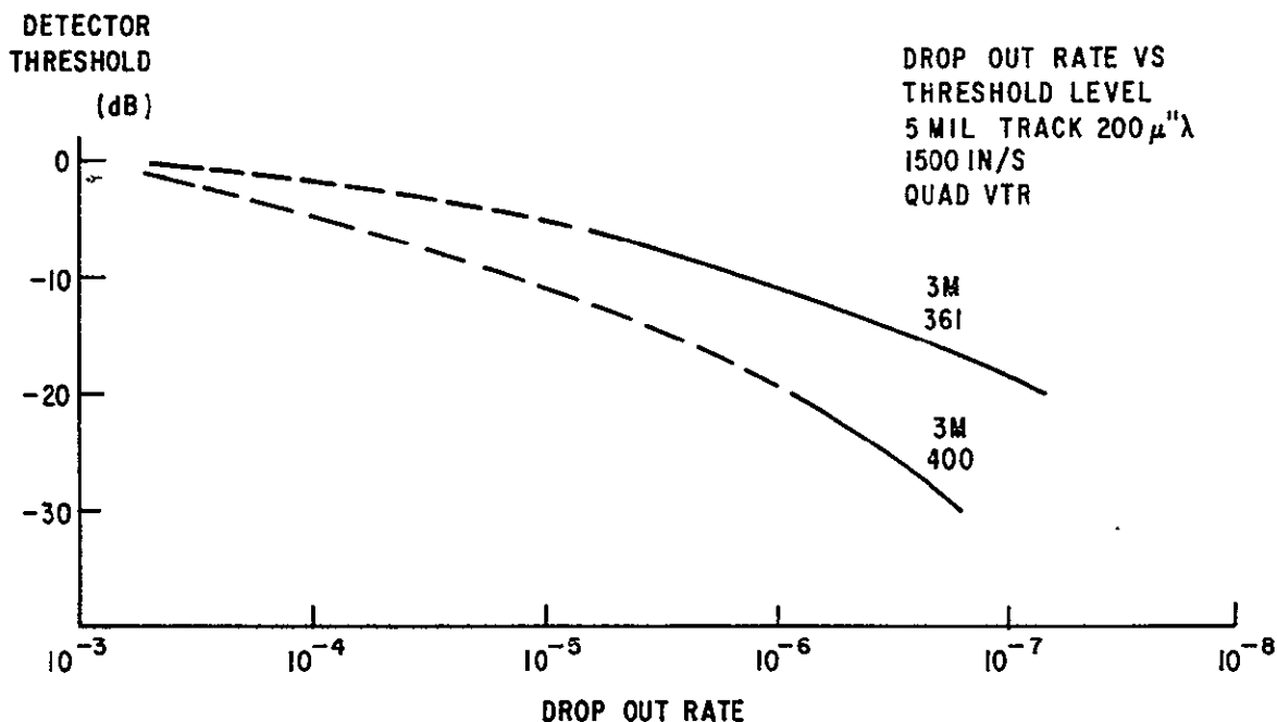
Figure 19. Dropout Rate vs Threshold Level
