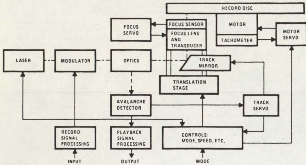
Figure 1. RCA optical video disc system.
