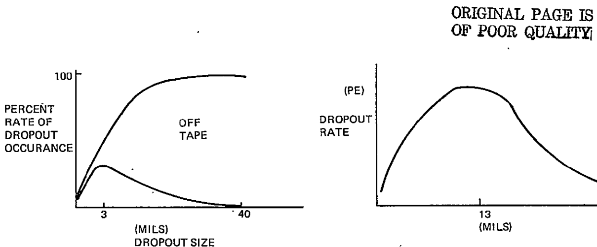
Figure 17A. A Rate of Occurrence Versus Size of Dropouts
