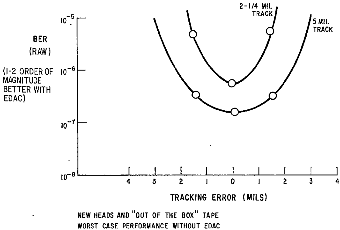
Figure 14. BER Vs. Tracking
