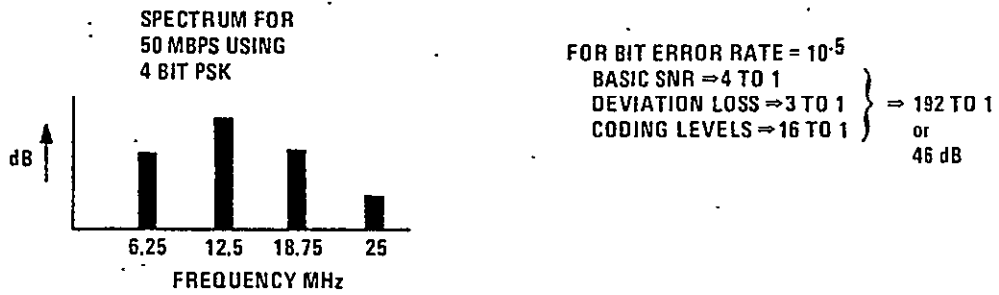
Figure 6. Multilevel coding considerations.
