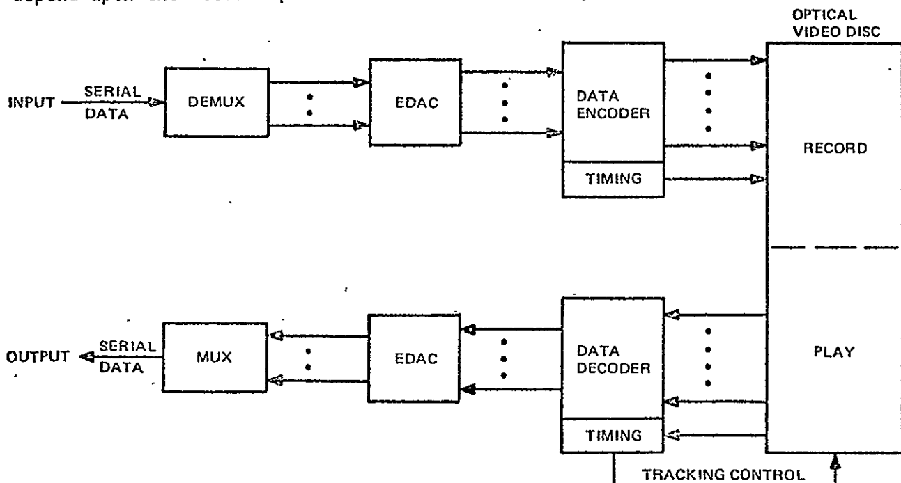
Figure 5-5. OD Record/Reproduce Signal Processing
