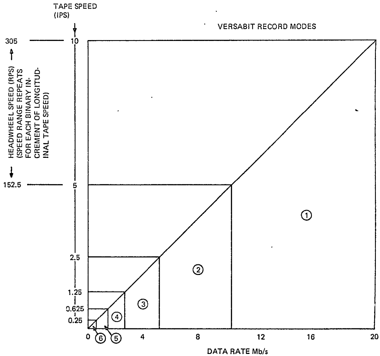
Fig. 6. Recording parameters V_{LR} and W_R/2\pi as functions of data rate.
