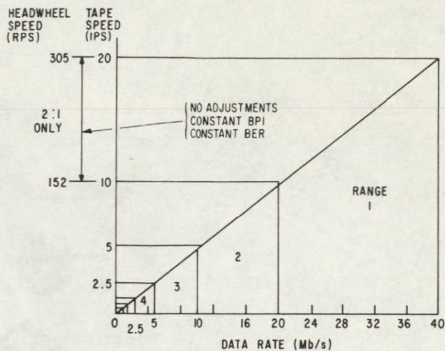
Figure 11. 40:1 Data Rate Range
