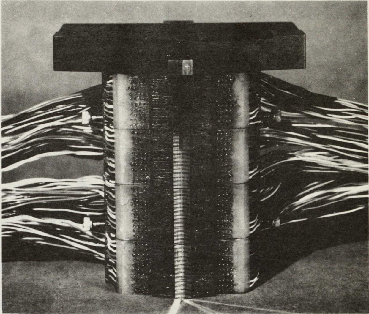
Figure 5. 164-Track High Density Multichannel Recording Head
