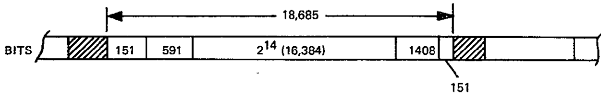
Figure 8. VERSABIT Tape Format Recorded Data Track (ASA C98.6)
