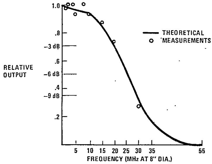
Figure 5. Frequency response of RCA OVD.
