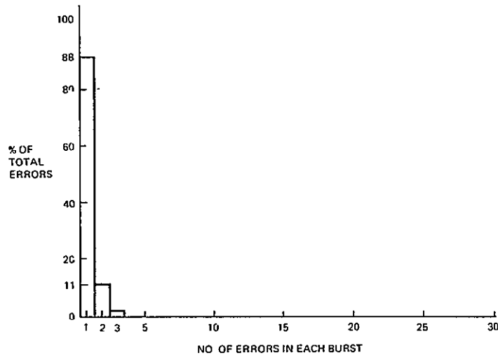
Figure 18. Rate of Occurrence Versus Size of Dropouts After Interleaver
