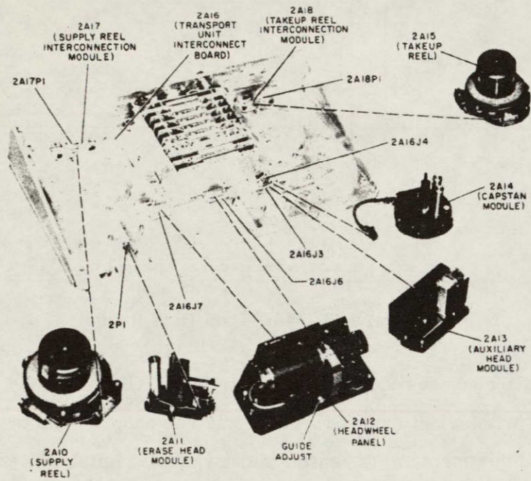
Figure 12. MIL-E-5400 Transport Sub-Assemblies
