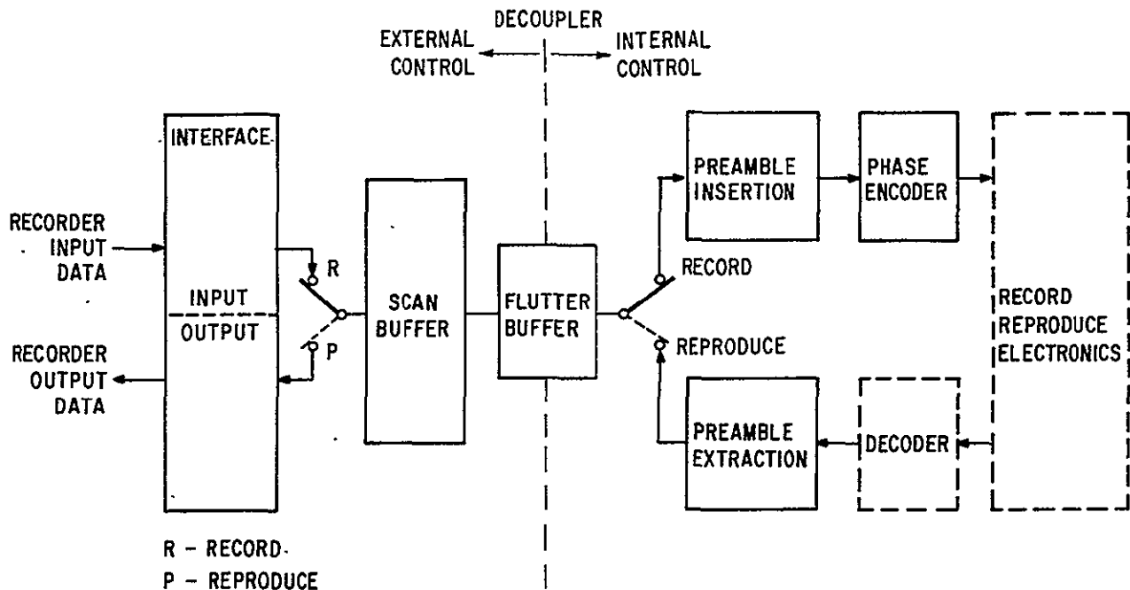
Figure 10. Data Processing Block Diagram
