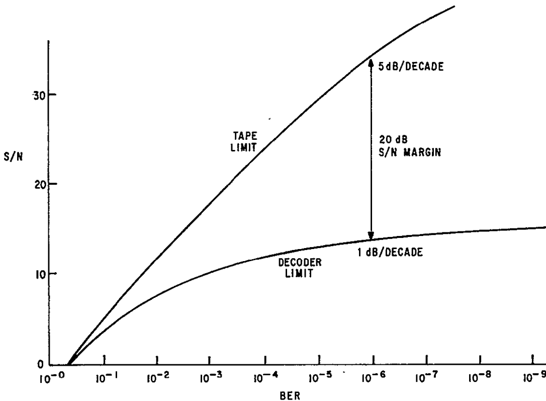
Figure 15. S/N Margin
