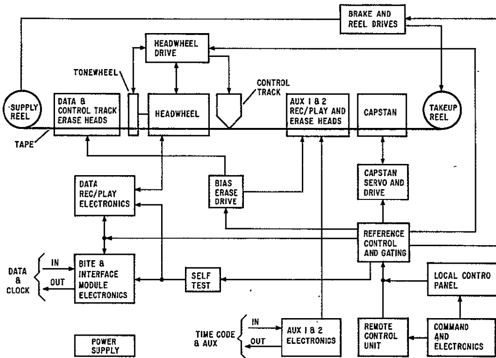
Figure 9. VERSABIT Simplified Block Diagram
