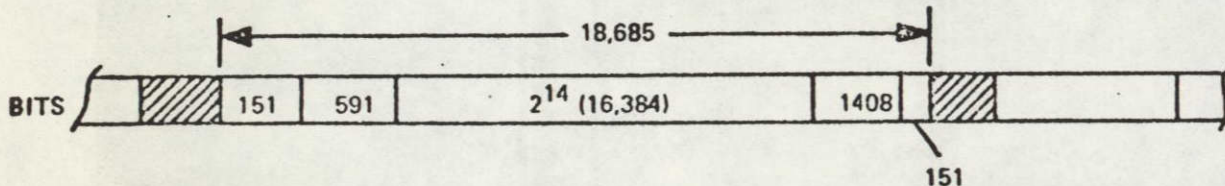
Figure 5-2. VERSABIT Tape Format Recorded Data Track (ASA C98.6)
