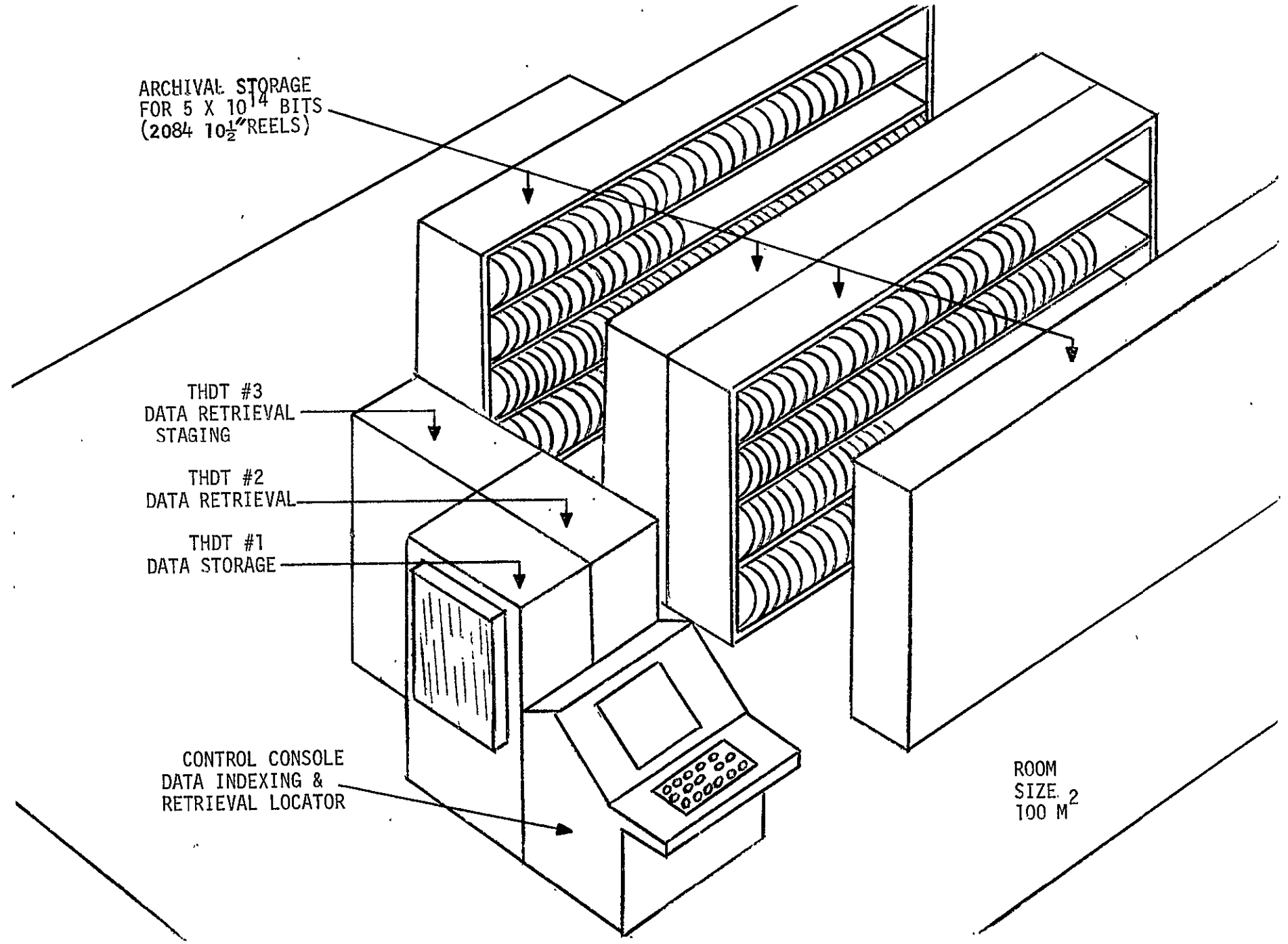
FIGURE 6 - 2 ARCHIVAL DATA STORAGE SYSTEM - THDT
