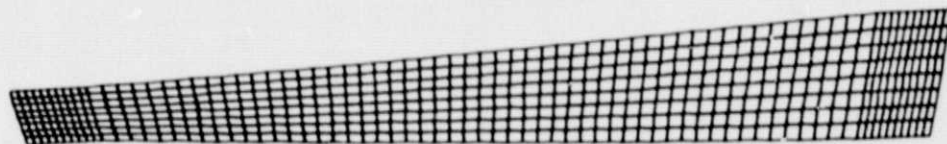
(c) Out-of-plane twisting moment (11,30 N·m (100 in·lb)); maximum deflection, 9.29 cm (3.658 in.).
