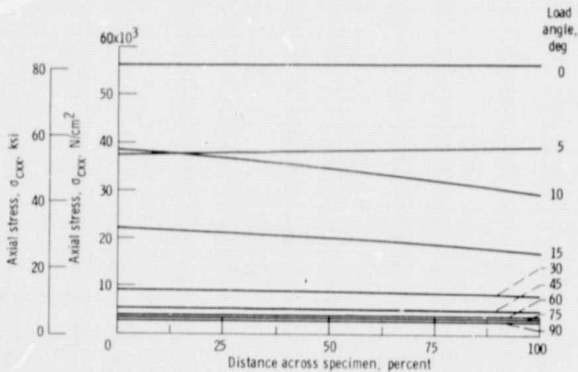
Figure 4. - Axial stress variation at midlengths for Mod I/E specimens for several load angles (finite-element analysis using the experimental fracture load for each specimen).
