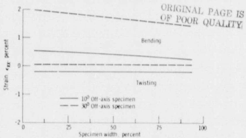
Figure 12. - Out-of-plane bending and twisting effects on axial strain at midlength of 10^\circ and 30^\circ off-axis specimens from Mod I/E composite (11.3-N·m (100-in·lb) moments).
