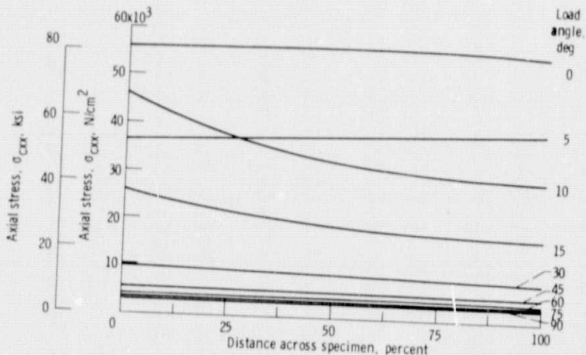
Figure 2. - Axial stress variation at tab ends for Mod I/E specimens for several load angles (finite-element analysis using the experimental fracture load for each specimen).
