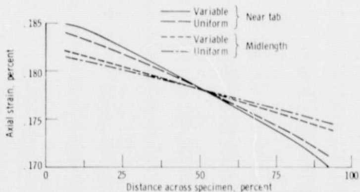
Figure 14. - Comparison of finite-element analysis results for 50^\circ off-axis specimen (Mod I/E) showing effects of specimen thickness variation.
