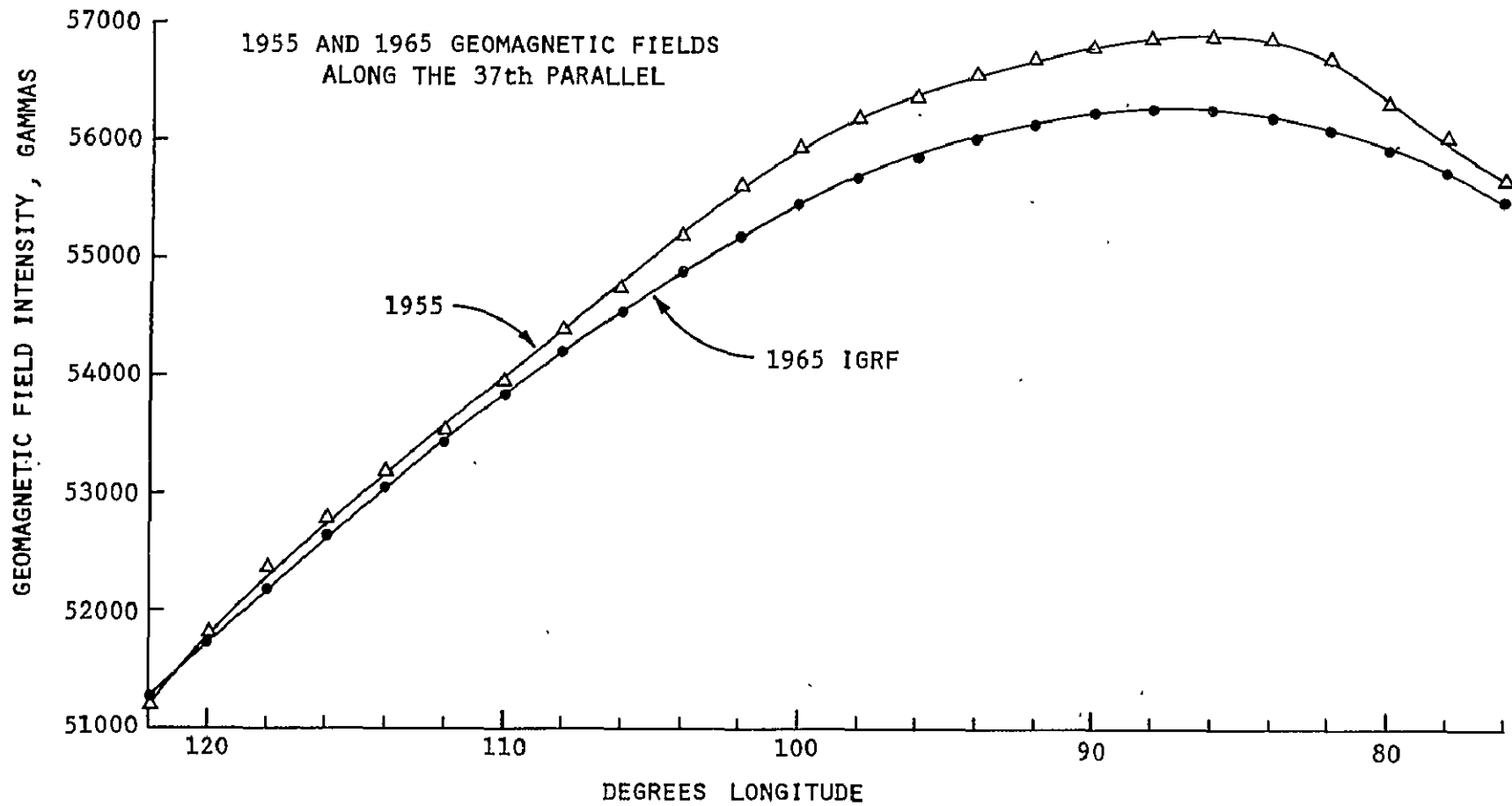
Figure 31. The U.S. Coast and Geodetic Survey's 1955 geomagnetic field and the 1965 International Geomagnetic Reference Field along the 37th parallel of latitude across the continental United States.
