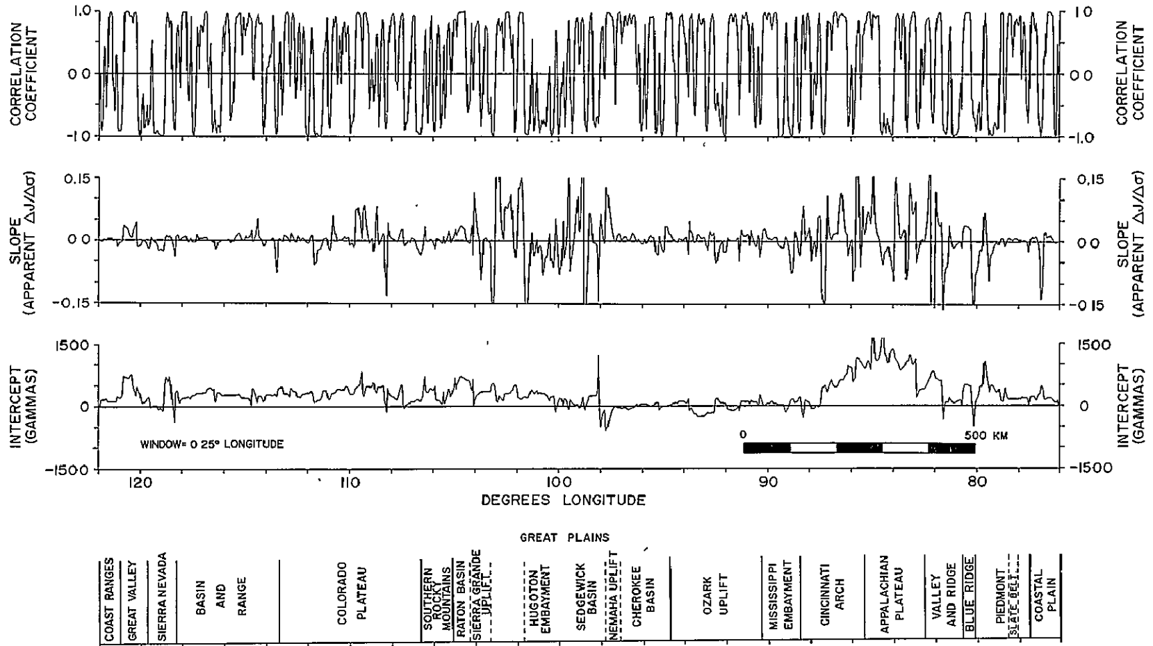
Figure 37. Internal correspondence results of 37th parallel anomaly data upward continued to 6 km.
