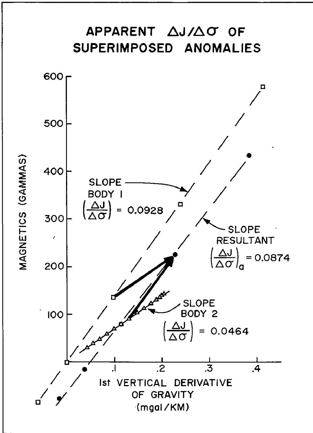
Figure 10. The vector sum of magnetics versus first vertical derivative of gravity relations resulting in an apparent \Delta J/\Delta\sigma .
