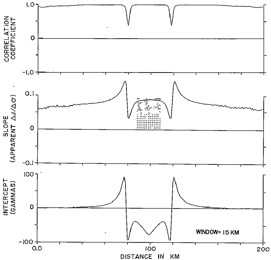
Figure 9. Superimposed anomaly sources: internal correspondence results. The level of the fine stippled bar equals the \Delta J/\Delta \sigma of the upper source, 0.0928, the bold of the lower source, 0.0464.
