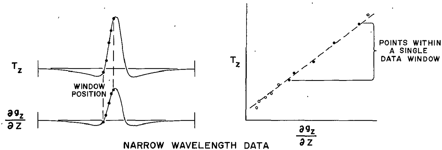
Figure 11. The effect of window size on the range of magnetic versus first vertical derivative of gravity values used in each regression.
