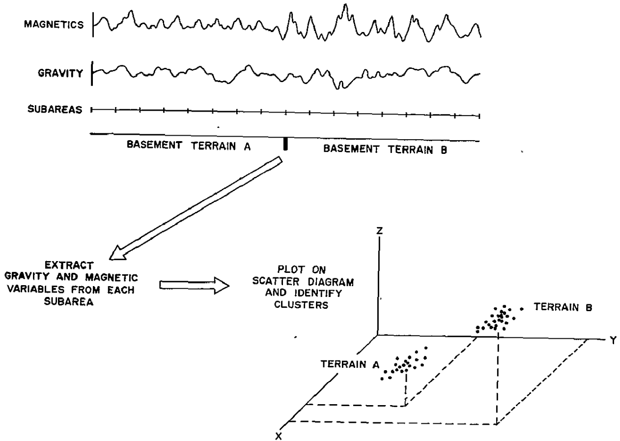
Figure 26. Schematic diagram illustrating the application of cluster analysis to gravity and magnetic data.
