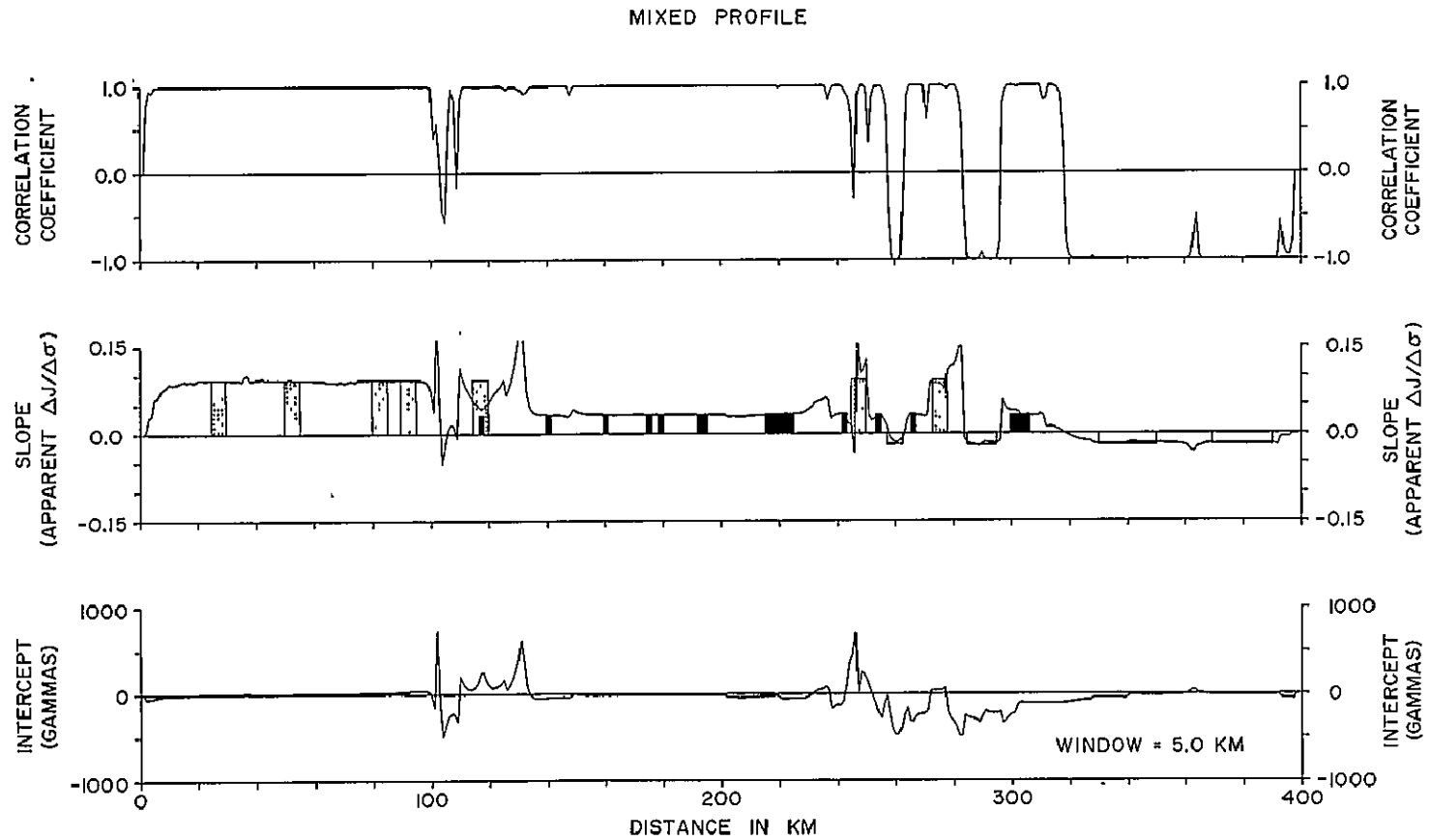
Figure 23. Mixed profile: internal correspondence results using a 5 km window. Position of shaded bars represent source positions and their levels represent actual source \Delta J/\Delta\sigma values.
