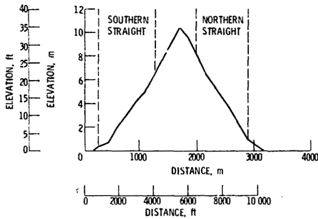
(c) Elevation.
