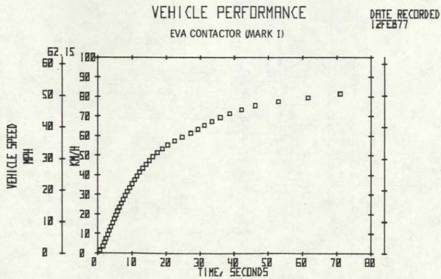
Figure 5. - Vehicle acceleration.
