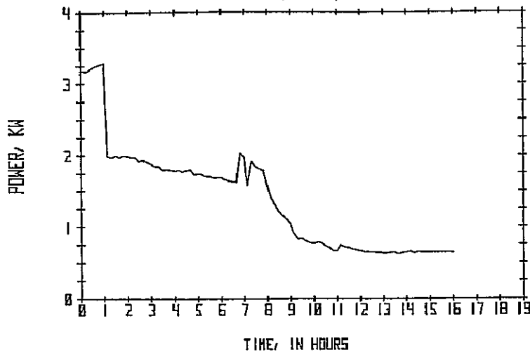
Figure 18 - Battery charger output power
