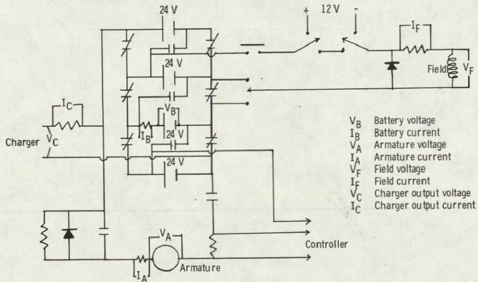
Figure 3. - Schematic diagram of EVA Contactor power circuit and instrumentation.
