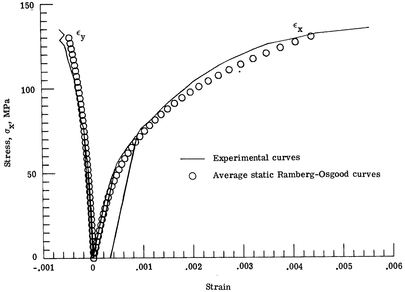
(b) Transverse test.
