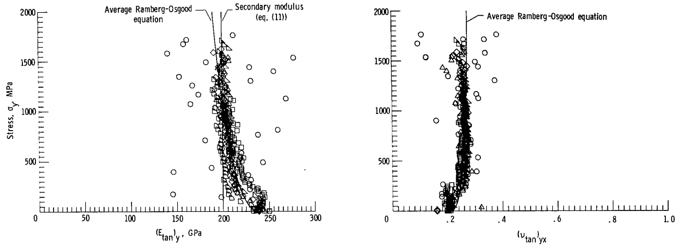
(a) Longitudinal tests.
