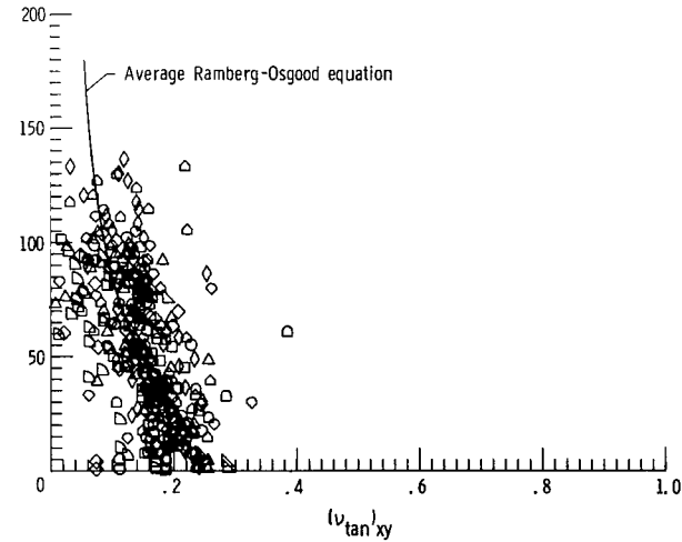
Figure 11.- Tangent moduli and Poisson's ratios for [0_2/+45]_S laminates.
