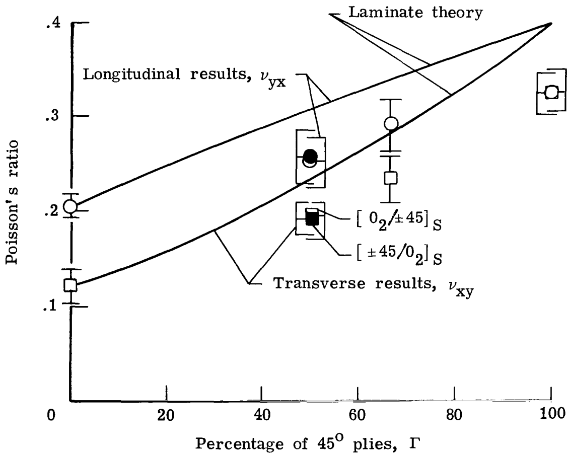
(b) Poisson's ratio.
