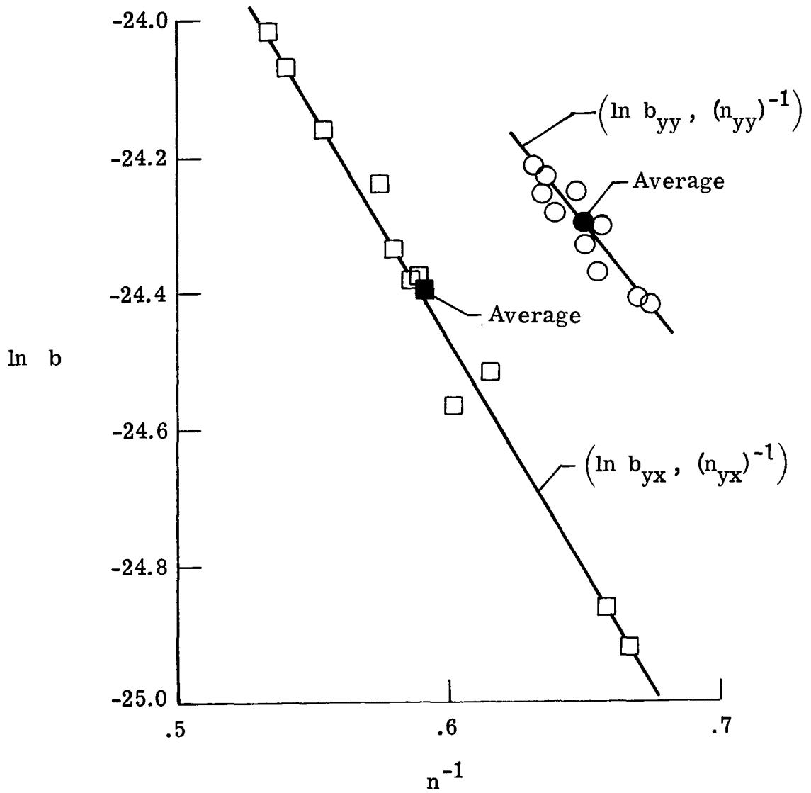
Figure 24.- Ramberg-Osgood constants for longitudinal tests of [0_2/+45]_S laminates.
