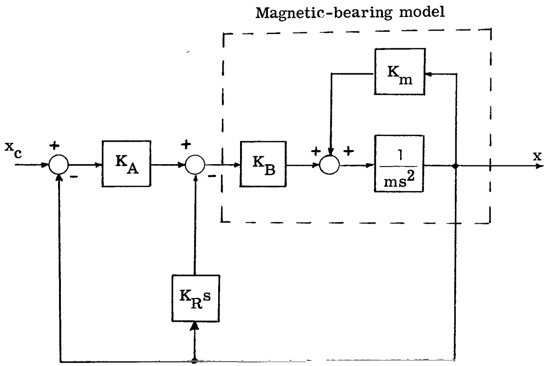
Figure 5.- Block diagram of simplified magnetic-bearing suspension servo.
