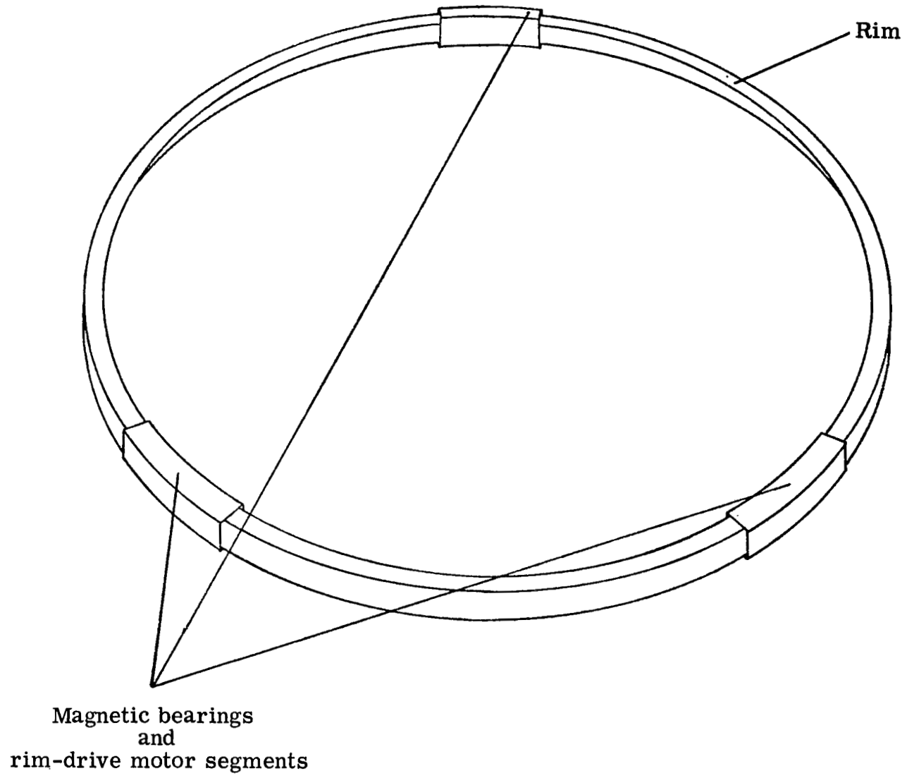
Figure 1.- Annular momentum control device concept.
