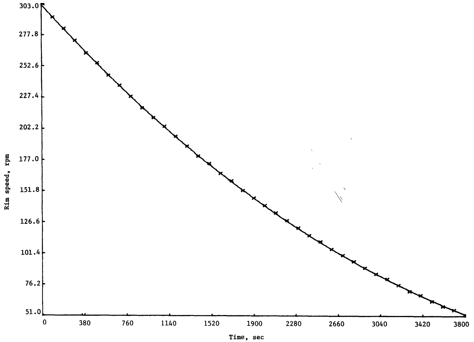
Figure 7.- Rim speed plotted against time during spin-down.
