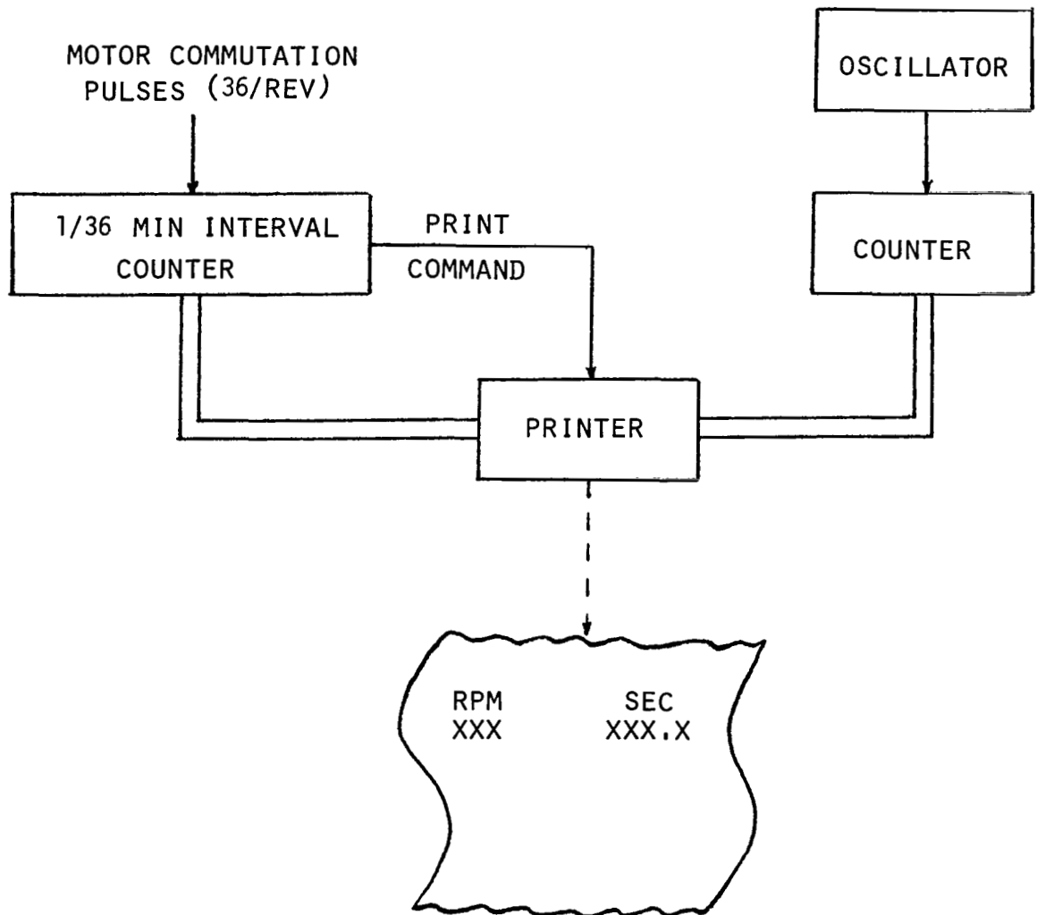
Figure 11.- Data acquisition system used in spin-up and spin-down tests.
