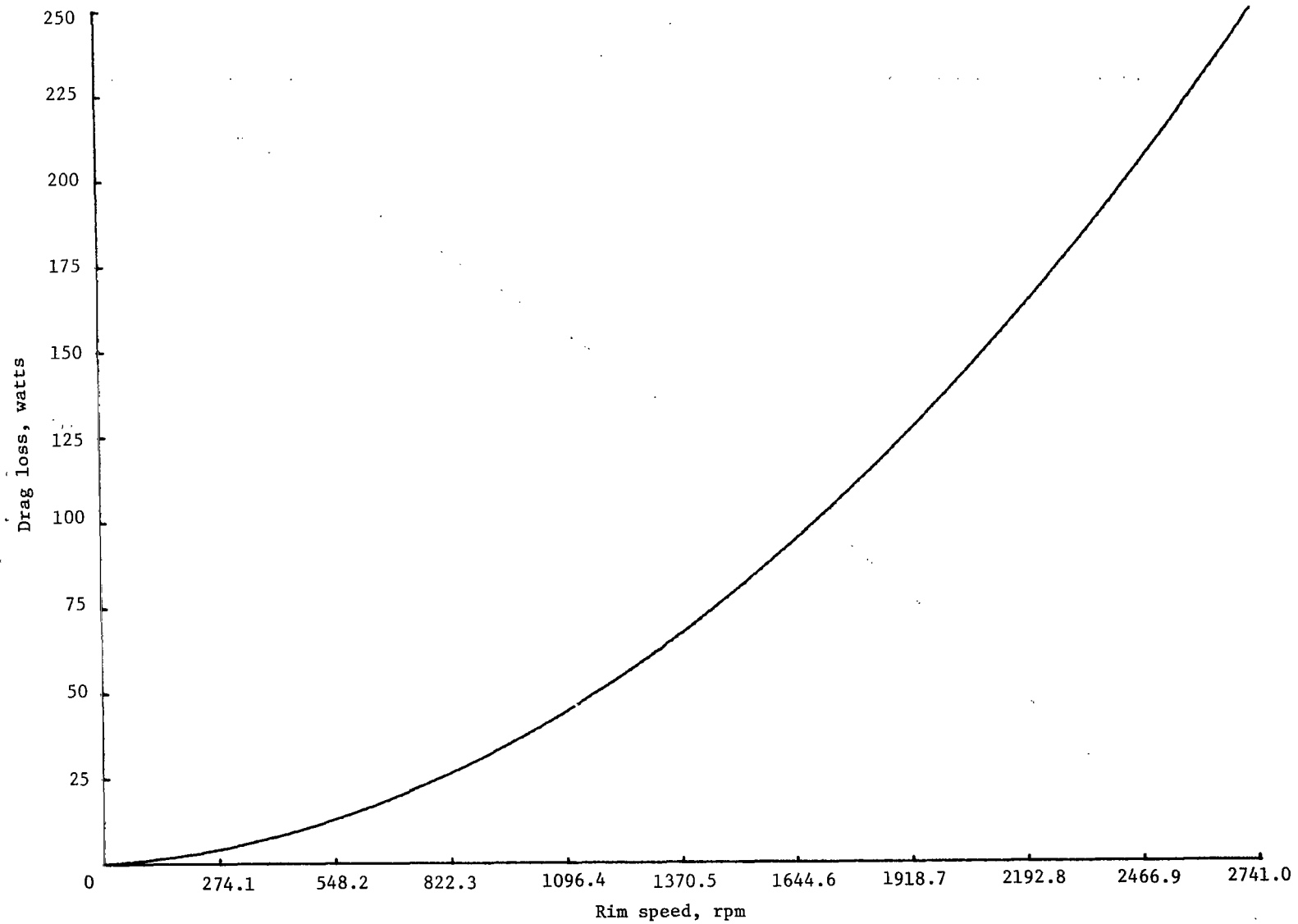
Figure 9.- Total drag loss projected to full speed.
