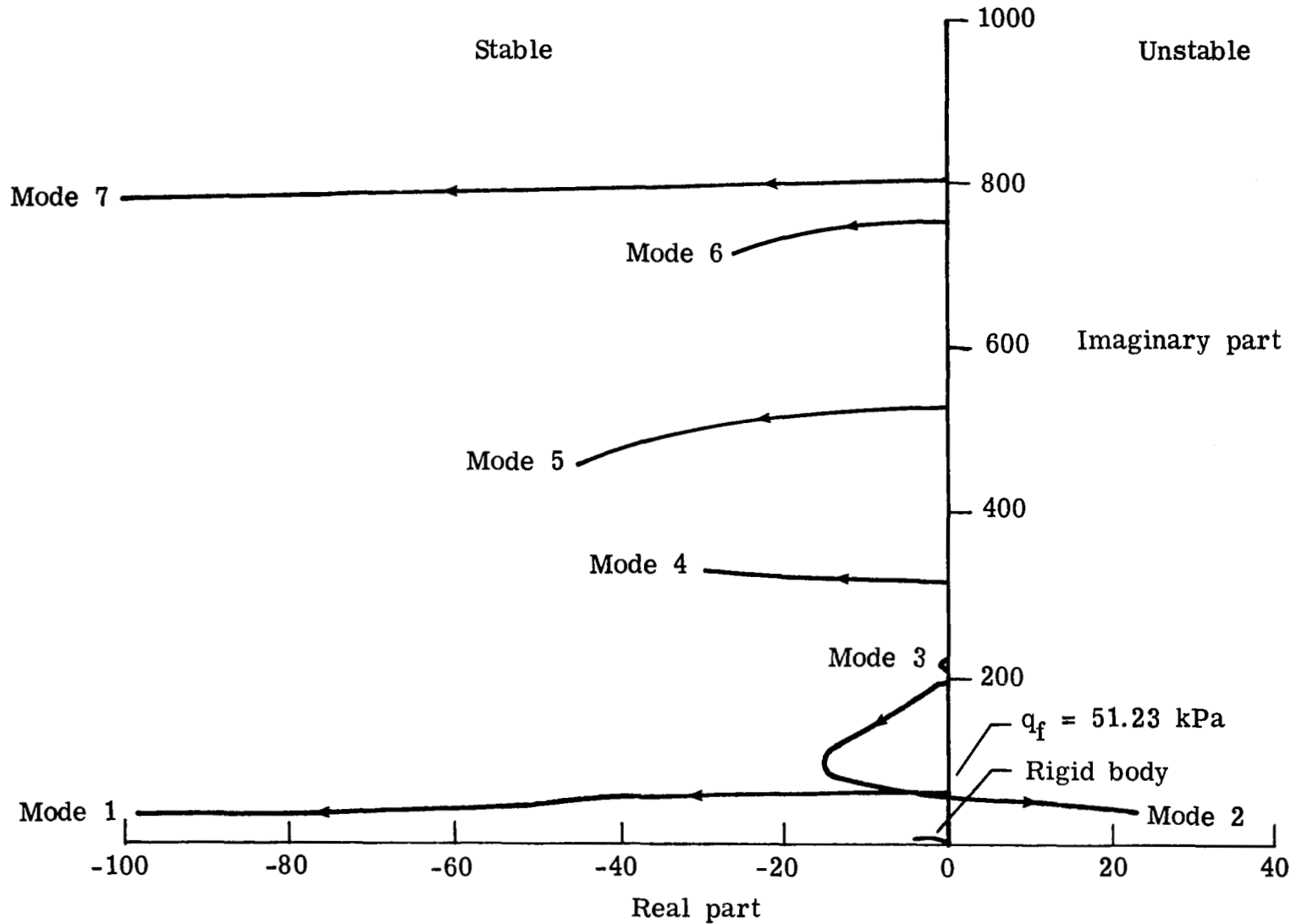
Figure 15.- Root locus plot of optimized trailing-edge control system at M = 0.7 by using DTF. Arrows indicate increasing dynamic pressure.
