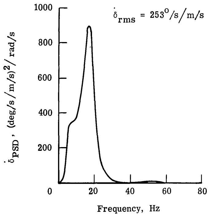
Figure 8.- Power spectral density (PSD) of control surface response at M = 0.90 using LDTF. ( 60 \leq \omega_{n,T} \leq 150 rad/s.)
