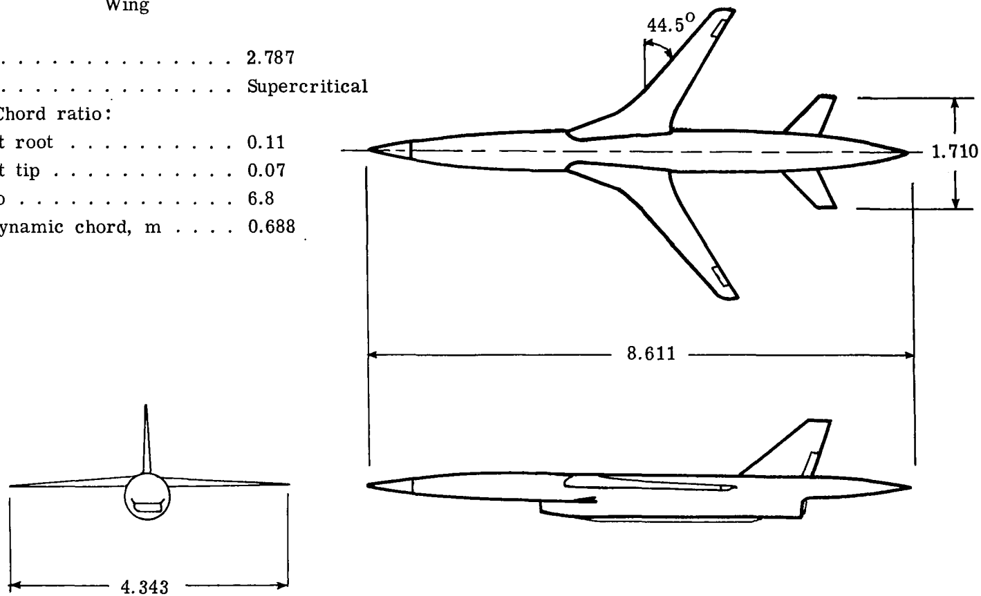
Figure 1.- Three-view drawing of drone research vehicle. All linear dimensions are in meters.
