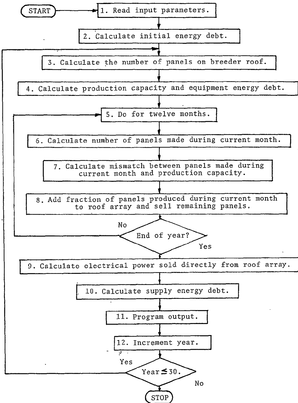
FIG. 14. PROGRAM STRUCTURE
