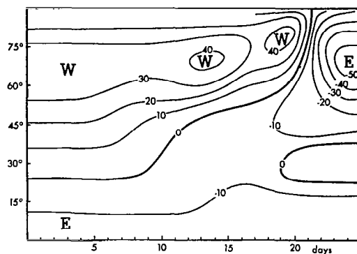
Figure 6.26. - Time-latitude section of mean zonal winds at z = 30 \text{ km} for case C2. Source: Ref. 42.
