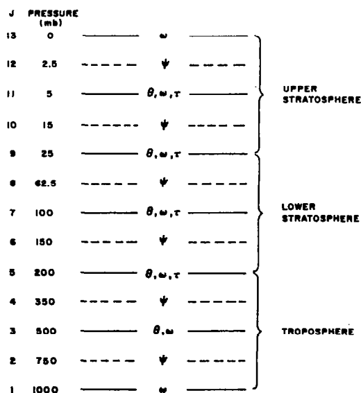
Figure 6.16. - Vertical resolution of Clark's model. Source: Ref. 89.
