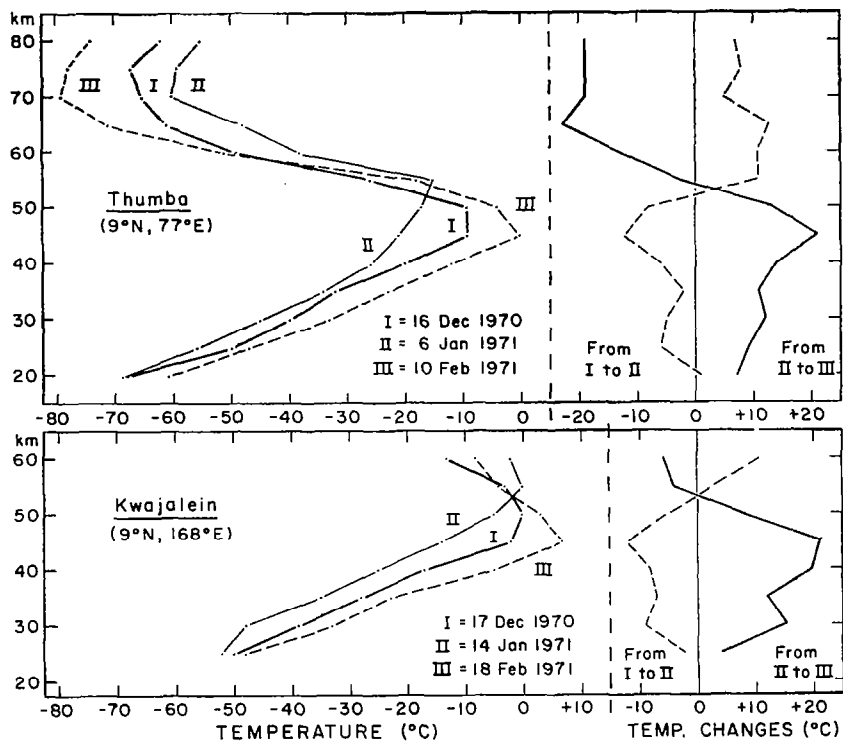
Figure 8.3. - Typical vertical temperature profiles at two typical stations, Thumba, India (Russian instrument) and Kwajalein, Marshall Islands (American instrument), for the winter 1970-71; I, early winter before the beginning of a warming; II, approximately at peak of warming; III, late winter minimum. Also changes between I and II, and between II and III. Source: Ref. 84.
