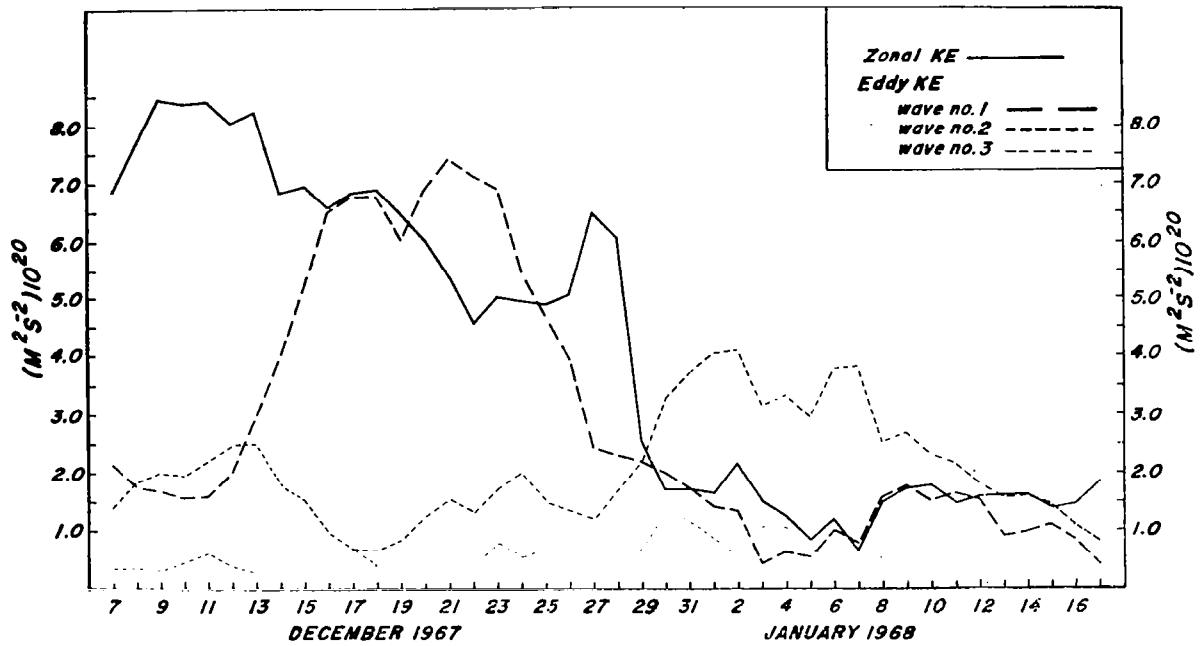
Figure 4.9. - 10-mb zonal and eddy kinetic energies for wave-numbers 1-3 during December 1967 and January 1968. All energies integrated over the region 17.5 - 82.5 degrees north. Units: 10^{20} m^2 s^{-2} . Source: Ref. 70.
