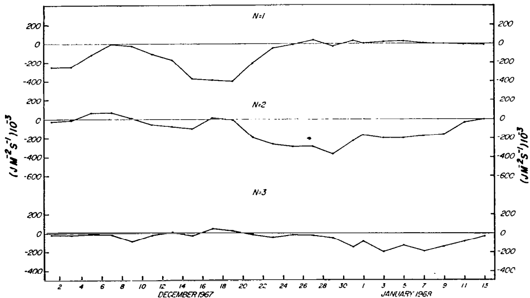
Figure 4.10. - Pressure-interaction term for wavenumbers 1-3 at 100 mb during December 1967 and January 1968. Units: 10^{-3} J m^{-2} s^{-1} . Source: Ref. 70.
