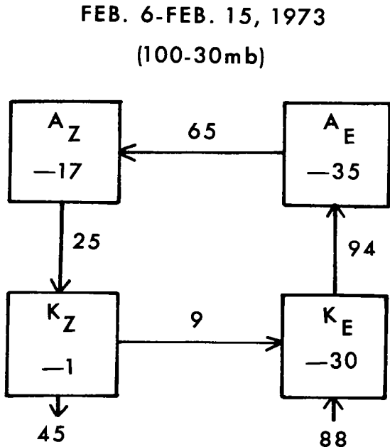
Figure 4.13. - Energy flow diagrams for periods leading up to the 1973 warming, and following the warming. Energy values are integrated for the periods indicated, between 22.5°N and 87.5°N for the layer 100-30 mb. Source: Ref. 41.
