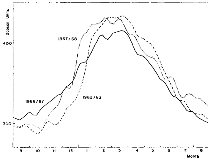
Figure 7.1. - Time cross-sections of the smoothed mean total ozone north of 40^{\circ} latitude for the winters 1962-63, 1966-67 and 1967-68. (Source: Ref. 99.)
