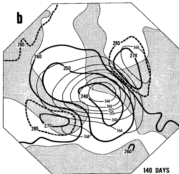
Figure 6.7. - The hemispheric variation of temperature (thick isolines), meridional velocity, and geopotential height (thin isolines) for the top level of the model at two different times illustrating the changes produced by the forcing from below. Shaded areas are regions of northwards velocity. Units: temperature, °K; geopotential height, 100 m). Source: Ref. 87.
