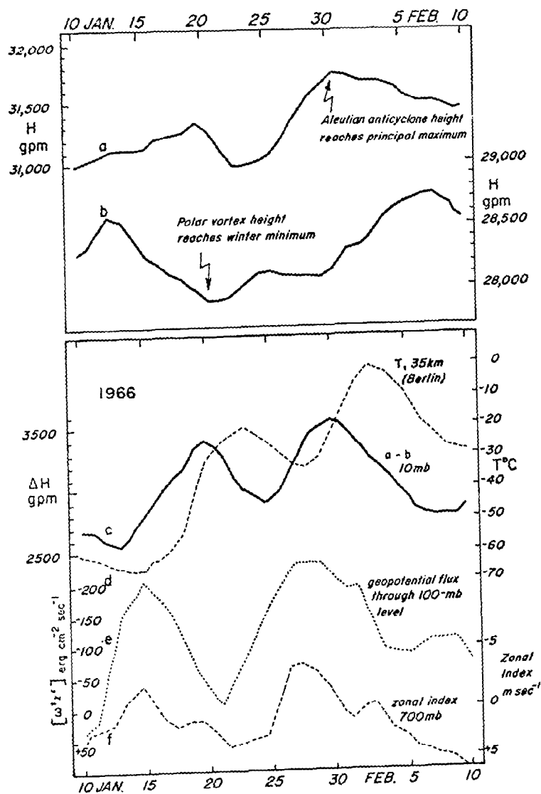
Figure 3.11. - Tropospheric and stratospheric parameters during early 1966. (a) maximum height of 10-mb surface north of 45^{\circ}N ; during period depicted, this was the height of the Aleutian-Siberian anticyclone. (b) central height of 10-mb polar vortex. (c) difference, (a) minus (b). (d) Berlin, Germany, temperature, 35 km. (e) vertical flux of geopotential, integrated over latitudes 17.5^{\circ}-82.5^{\circ}N , through the 100-mb level, wave number 1. Negative values refer to upward flux. (f) polar zonal index ( 55^{\circ}-70^{\circ}N ), 700 mb, Western Hemisphere. Note parallelism of (e) and (f), both leading (c) by 3-5 days. Berlin temperatures, 35 km, lag (c) by about 3 days. Low zonal index values in mid- and late January were associated with blocking of westerlies. (Source: Ref. 40.)
