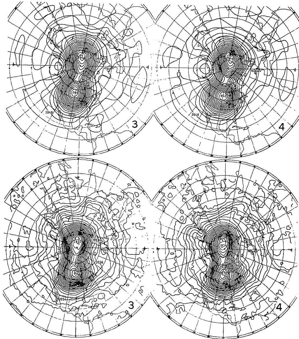
Figure 6.2. - Same as Figure 6.1, except for the following two days. Source: Ref. 86.
