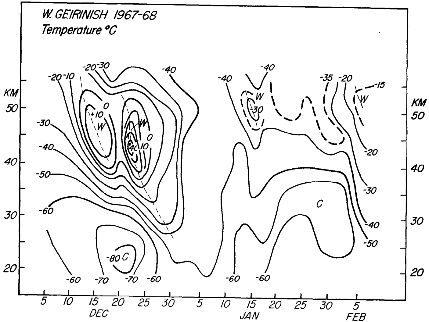
Figure 3.17c. - Temperature data from rocket soundings at West Geirinish, Scotland, suggesting downward propagation of warming. Source: Ref. 27.
