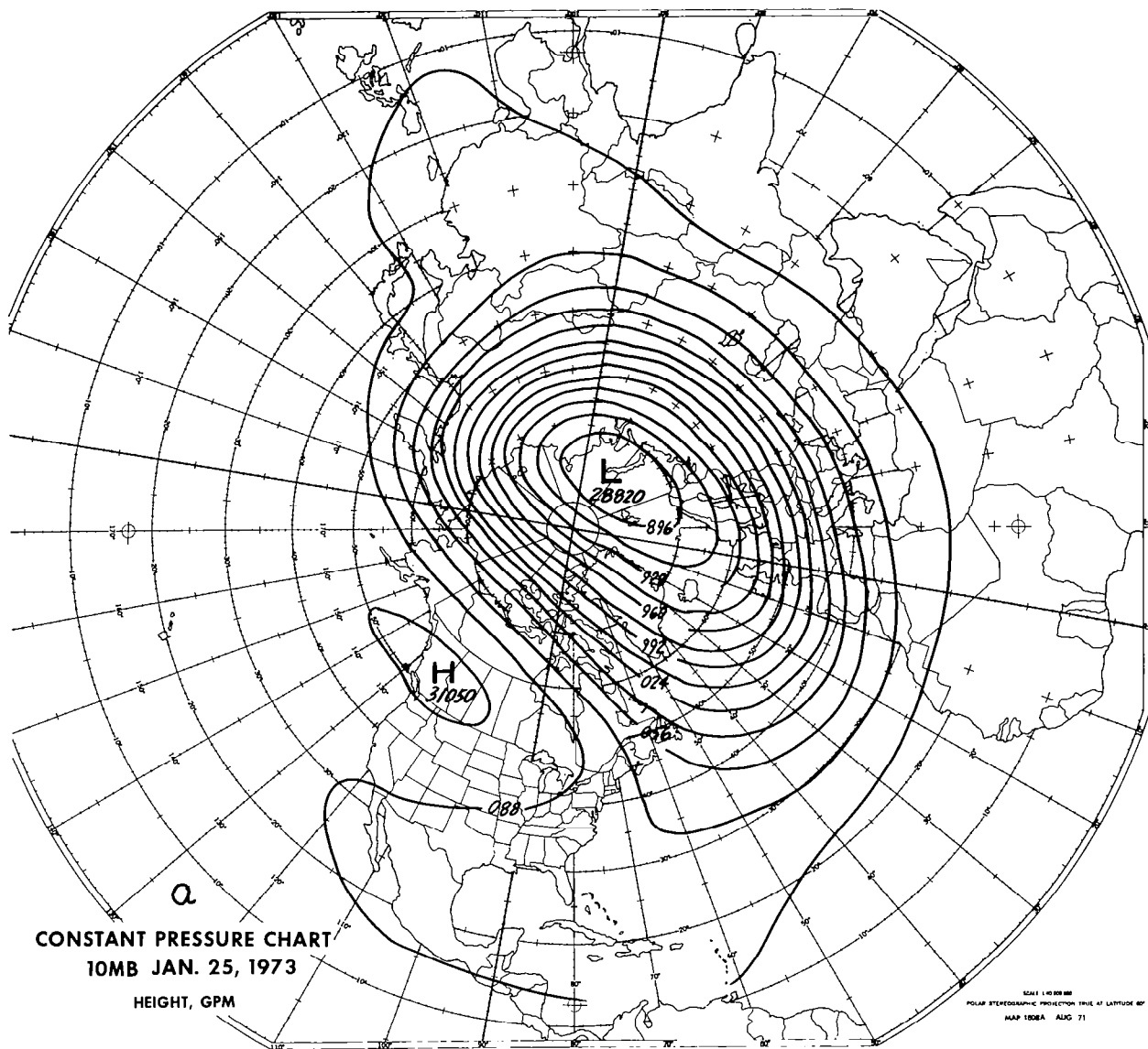
Figure 3.14a. - 10-mb map for 25 January 1973.
