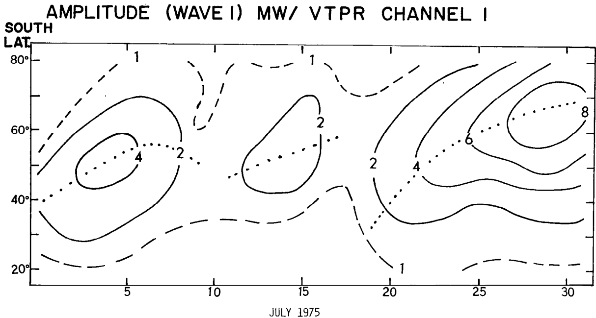
Figure 3.19. - Amplitude of wavenumber 1 in radiance (VTPR Channel 1), 20-80°S, July 1975.
