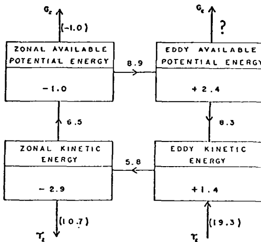
Energy flow diagram, 25 January-4 February 1957. Rates of energy change (ergs cm -2 mb -1 sec -1 ) appear in boxes. Arrows indicate direction of energy flow. Figures by arrows give rates of energy conversion, transfer, or generation (ergs cm -2 mb -1 sec -1 ). Figures in parentheses represent only crude estimates.
