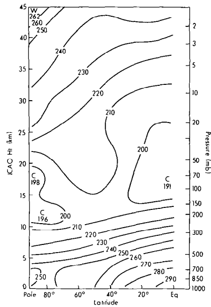
Figure 6.12. - Zonally mean cross-section of temperature in ^{\circ}K for day 90. Source: Ref. 43.
