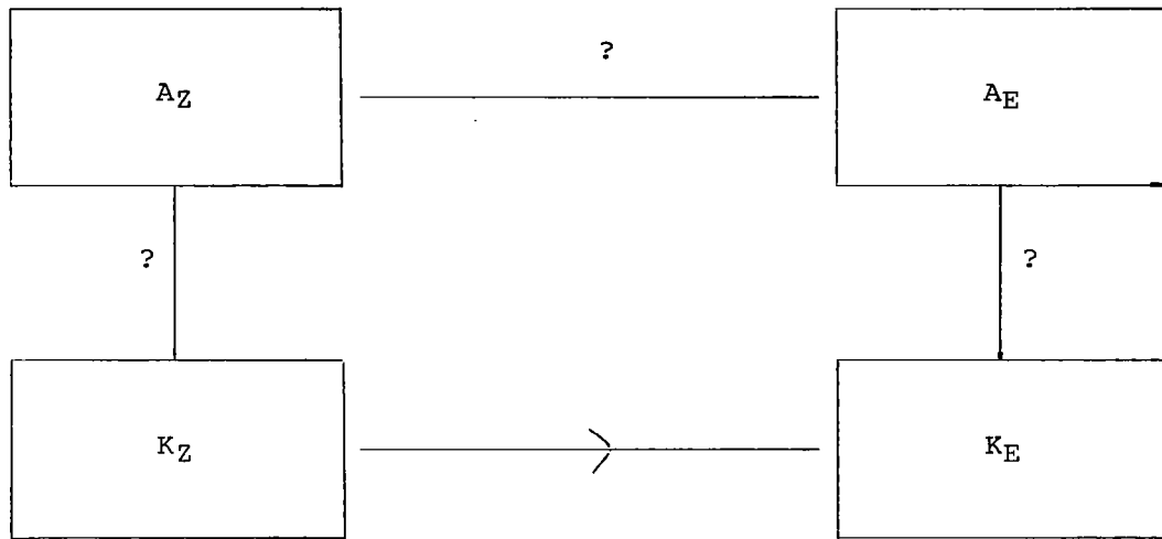
BAROTROPIC
