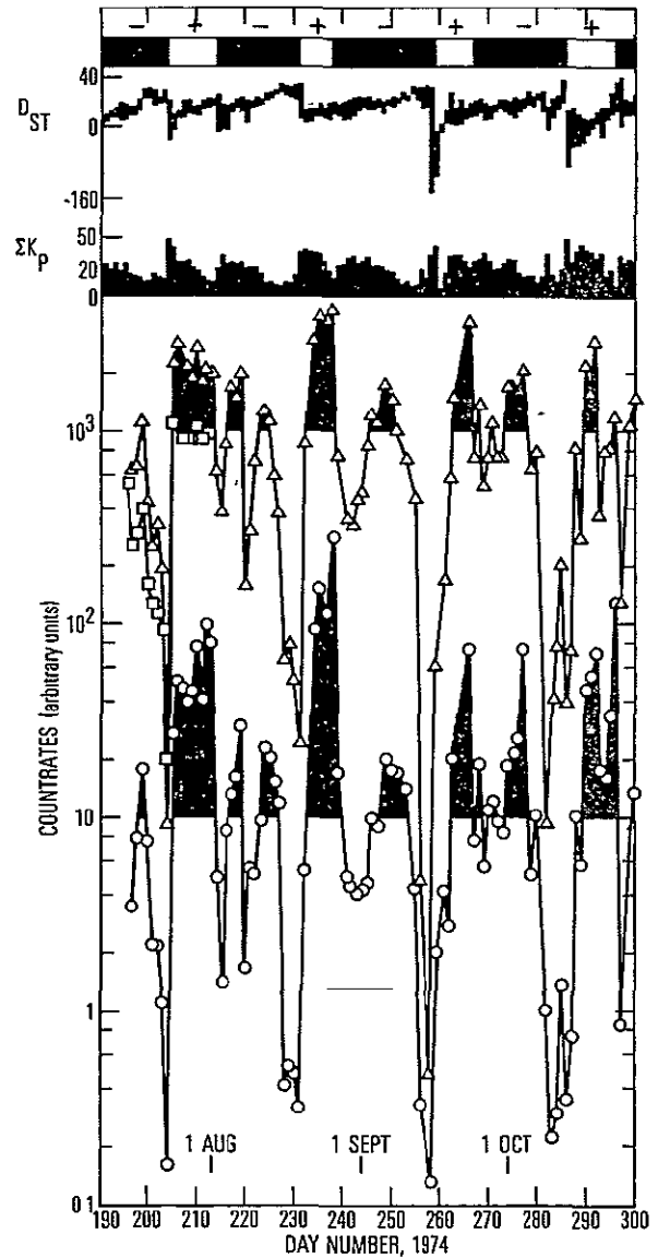
Figure 1. Hourly averages of energetic electron count rates observed in the late summer and fall of 1974 by ATS-6 and ATS-1 are plotted as a function of Day Number, 1974. Also plotted (at the top of the figure) are the polarity of the interplanetary magnetic field as inferred by Svalgaard (1975), the daily sum of K_p and the range of D_{st} for each day. Local time for all particle data is local noon, the sector boundary transitions are assumed to occur at 0000 UT for the days indicated. Circles and triangles are ATS-6 observations of > 3.9 and > 1.6 MeV electrons respectively, squares are ATS-1 observations of > 1.9 MeV electrons. For emphasis we have shaded those portions of the curves where E > 1.6 MeV count rates exceed 10^2/\text{sec} and E > 3.9 MeV count rates exceed 10/\text{sec} .
