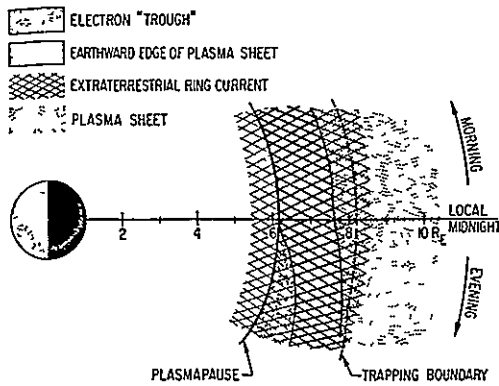
Fig 1 Spatial relationships near the synchronous orbit at local midnight between the ring current, the plasmopause, the energetic particle trapping boundary, and the Earthward terminus of the plasma sheet. This figure is qualitative and representative of magnetic quiet (from Frank [1])
