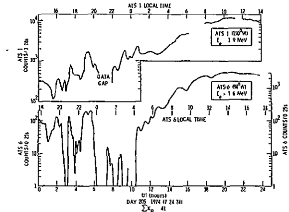
Fig 8 Comparison of energetic electron count rates observed by ATS-6 and ATS-1 during a magnetically disturbed day (day 205).
