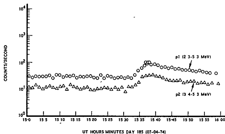
Fig 10 Increase in solar proton flux associated with a sudden commencement (a compression of the geomagnetic field) near 15 35 on July 4, 1974
