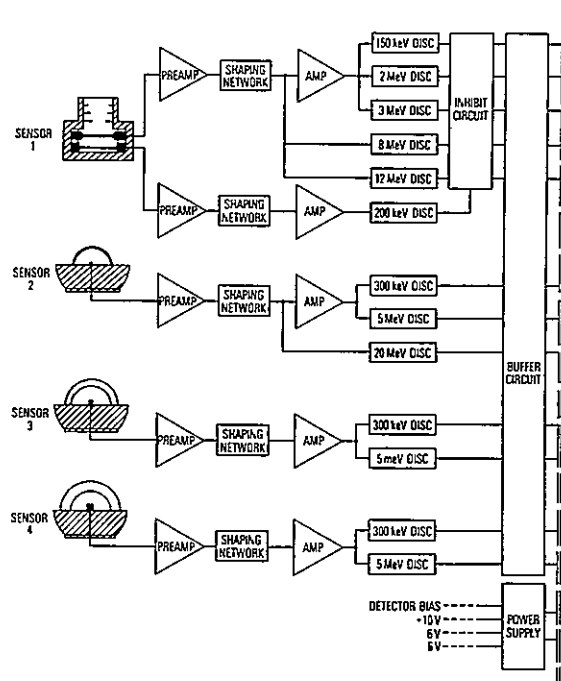
Fig 3 Schematic block diagram of detector/electronic system
