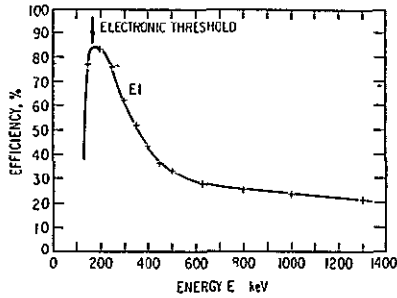
Fig 4 Efficiency of detection of electrons in the E1 channel This channel has a nominal energy sensitivity of 140-600 keV Sensitivity of this channel below the nominal electronic threshold is associated with the finite noise of the detector
