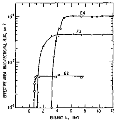
Fig 5 Effective area of the E2, E3, and E4 electron channels as a function of electron energy This effective area, when integrated over the angular response of the detector, yields the omnidirectional geometric factor
