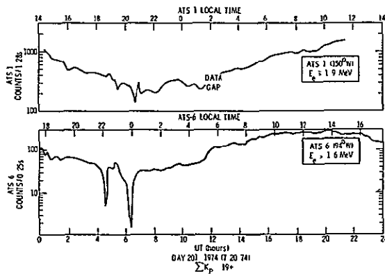
Fig 7 Comparison of energetic electron count rates observed by ATS-6 and ATS-1 during a magnetically quiet day (day 201). The three days preceding day 201 were also quiet.
