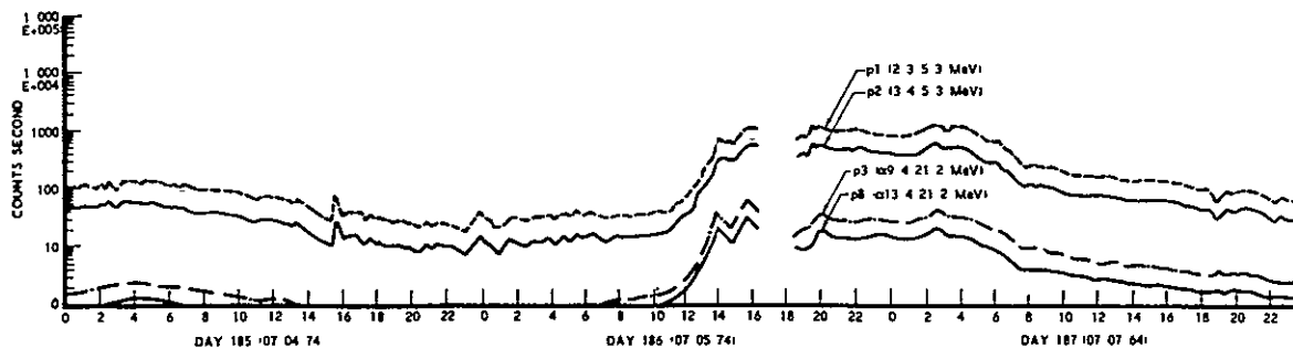
Fig 9 Count rates of proton and alpha channels during the solar proton event of July 1974 Data for two proton channels and two alpha channels for 4, 5, and 6 July 1974 are presented here
