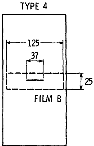
Figure 3.- Fracture specimen configurations. (All dimensions are in millimeters.)
