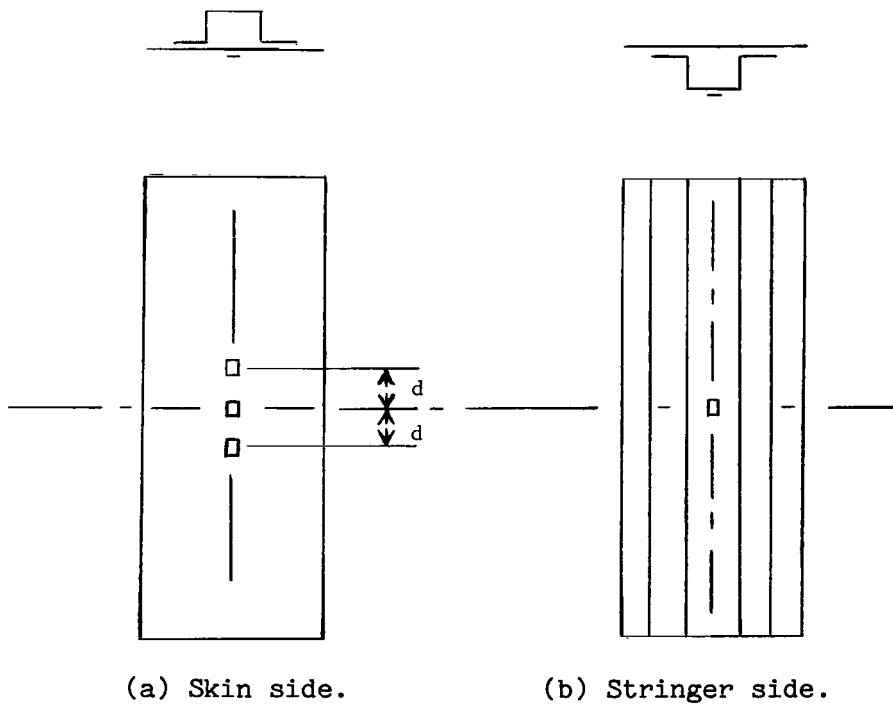
Figure 4.- Location of strain gages used in test of skin-stringer panels. d = 50.8 \text{ mm (2 in.)} .
