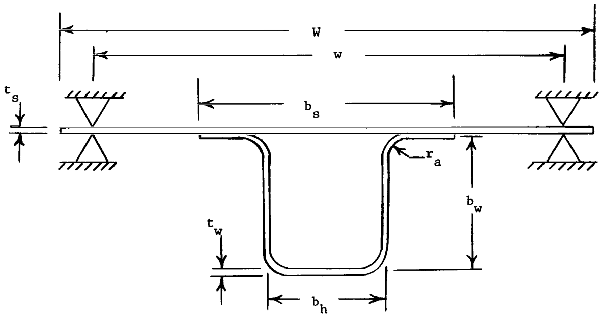
Figure 3.- Cross section of skin-stringer panel.
