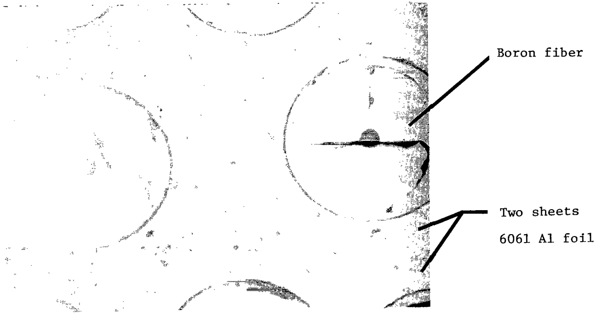
(a) Skin.
