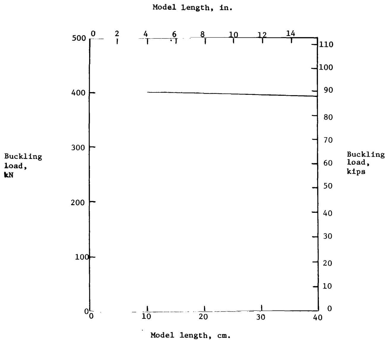
Figure 18.- Variation of analytical buckling load with model length.
