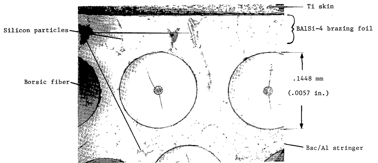
Figure 15.- Photomicrograph of typical BA1Si-4 brazed joint.
