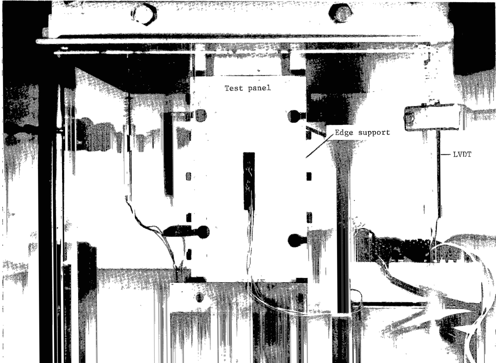
Figure 5.- Test setup for skin-stringer panels.
