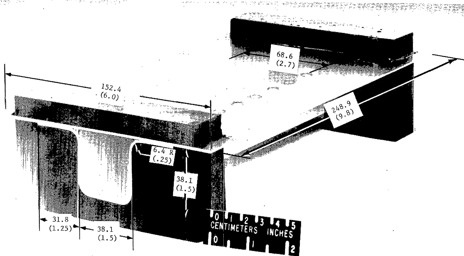
Figure 2.- Skin-stringer panel. Dimensions are given in millimeters (inches). L-74-4367.1
