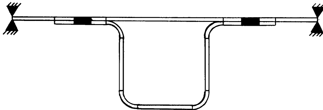
(b) Model 2 - simulates attachment by spotwelding.
