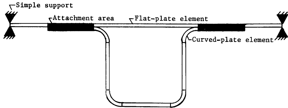
(a) Model 1 - simulates attachment by diffusion bonding, adhesive bonding, or brazing.
