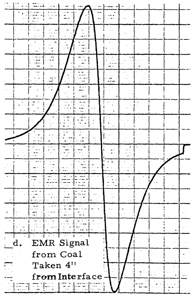
FIGURE 3. EMR SIGNALS FROM COAL AROUND THE FIRST (top) INTER- FACE AT DISTANCES FROM THE INTERFACE OF (a) 0 to 1/2", (b) 2", (c) 3" AND (d) 4".
