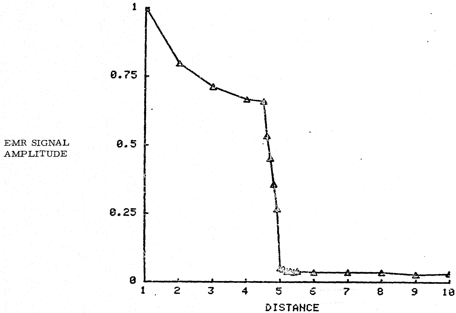
FIGURE 31. GRAPH OF THE EMR SIGNAL AMPLITUDE FROM THE MATHEMATICAL MODEL AS A FUNCTION OF DISTANCE WITH A COAL-ROCK INTERFACE AT 5 INCHES. Additional points are taken every 0.1 inch from 4.5 to 5.5 inches.
