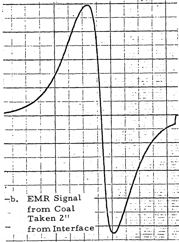
FIGURE 3. EMR SIGNALS FROM COAL AROUND THE FIRST (top) INTER- FACE AT DISTANCES FROM THE INTERFACE OF (a) 0 to 1/2", (b) 2", (c) 3" AND (d) 4".
