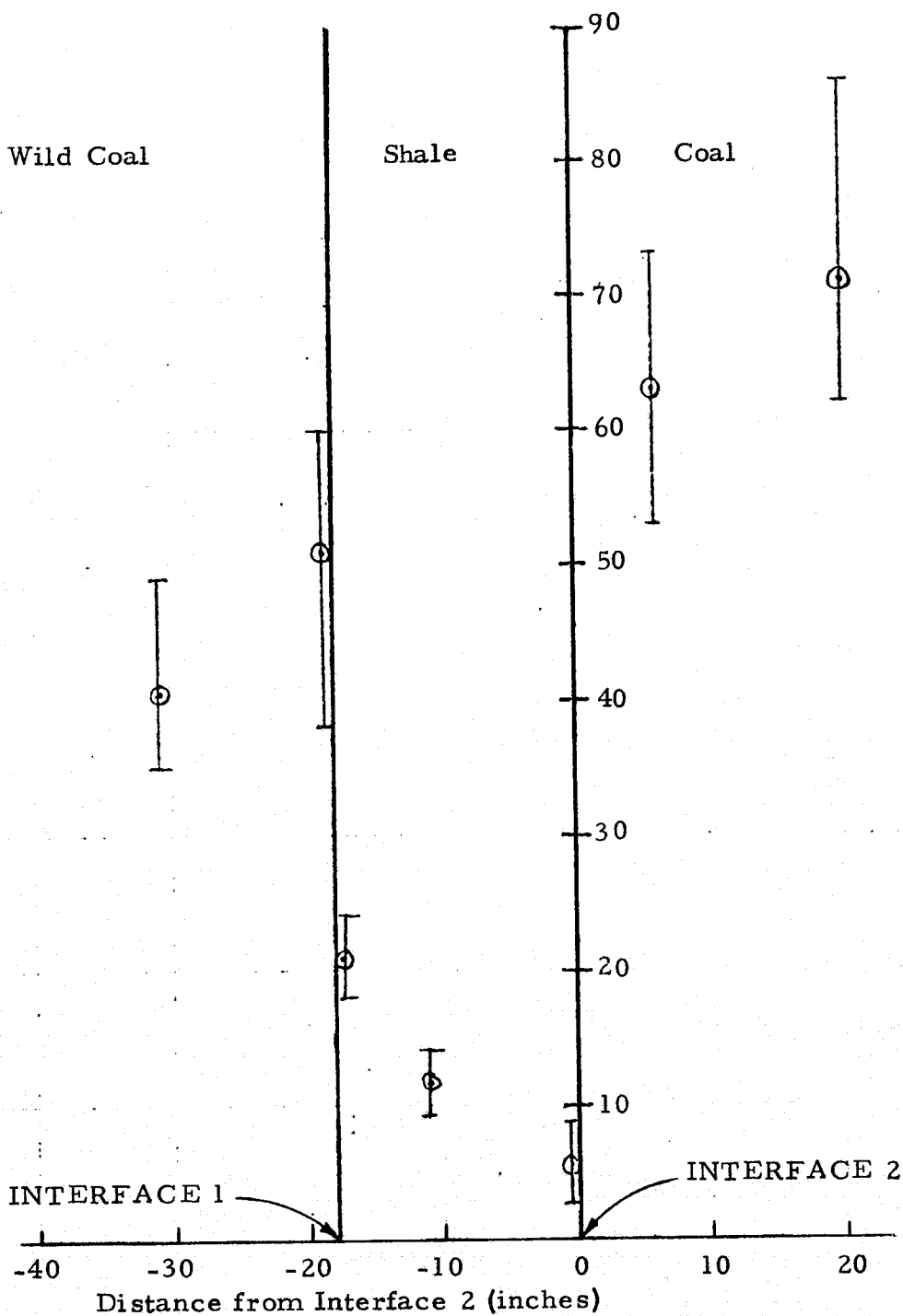
FIGURE 14. GRAPH OF THE MEAN VALUES AND LIMITS OF THE PEAK-TO-PEAK EMR SIGNALS FROM THE FOUR REPLICATES FROM EACH OF THE SEVEN SAMPLES FROM THE BRUCETON MINE
