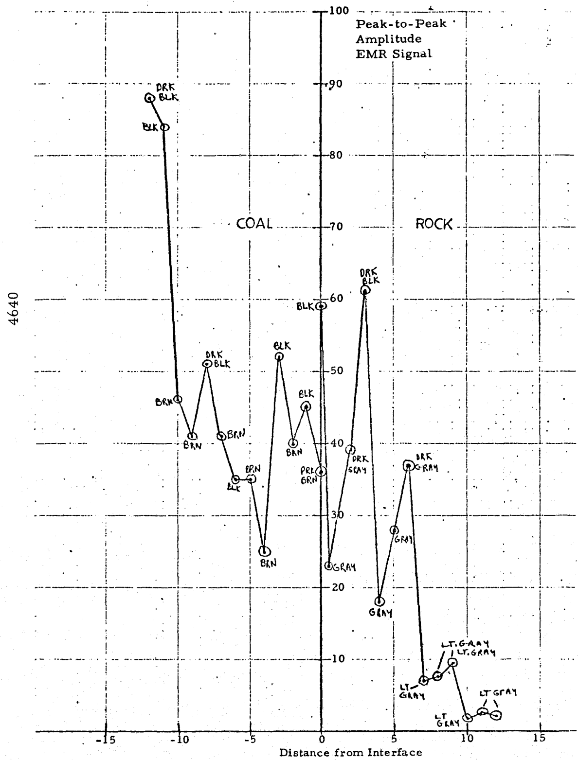
FIGURE 12. GRAPH OF THE PEAK-TO-PEAK VALUES OF THE REPEAT ELECTRON MAGNETIC RESONANCE SIGNALS USING AN IMPROVED ATTENUATION ADJUSTMENT TECHNIQUE, FROM THE SAMPLES TAKEN AT VARIOUS DISTANCES AROUND THE THIRD INTERFACE (Position 3) OF THE DRUMMOND STRIP MINE
