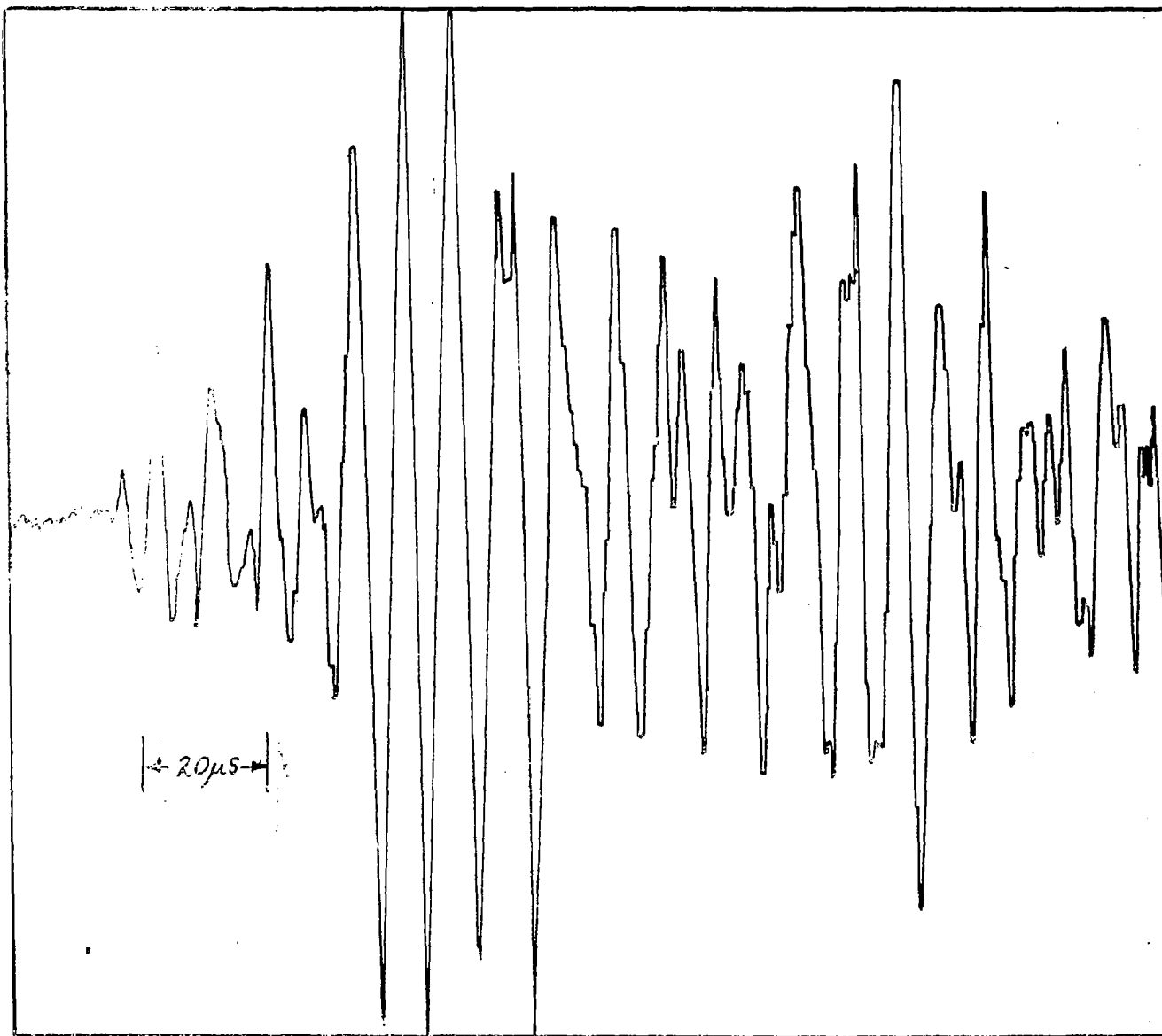
Fig. 2. Acoustic emission pulse from electrical spark.
