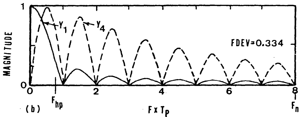
Fig. 26. Square pulse: \zeta = 1.66 ; F_{hp}/F_n = 1.43 ; T_p F_n = 8.0 .
