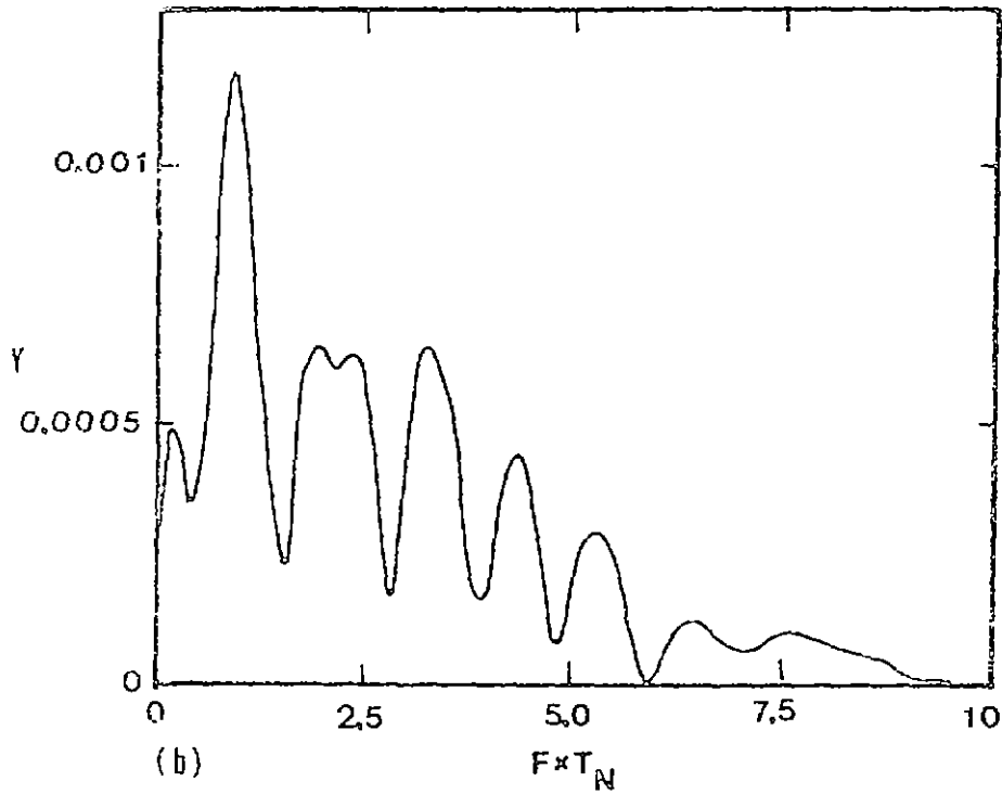
Fig. 4. Fourier spectrum of two pulses: a) square pulse input and b) unknown AE pulse input.
