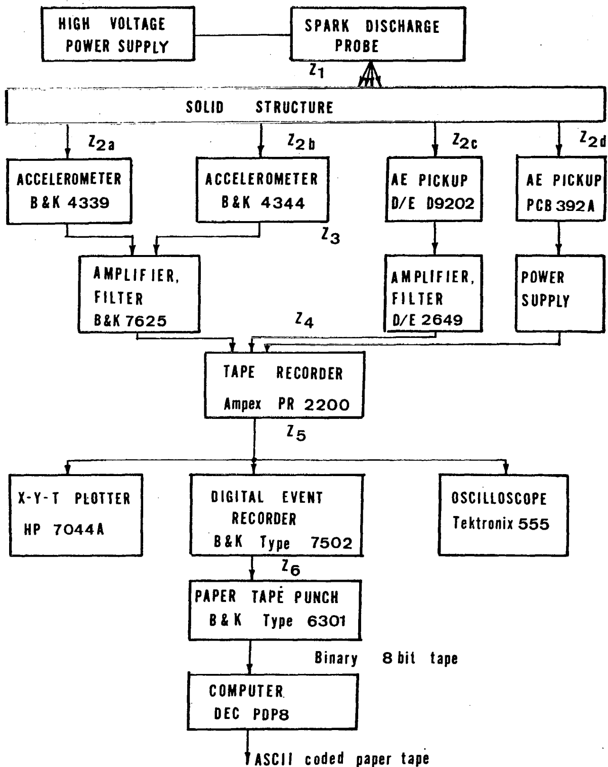
Fig. 33. Flow diagram of the components used for the spark discharge measurements with four different transducers.
