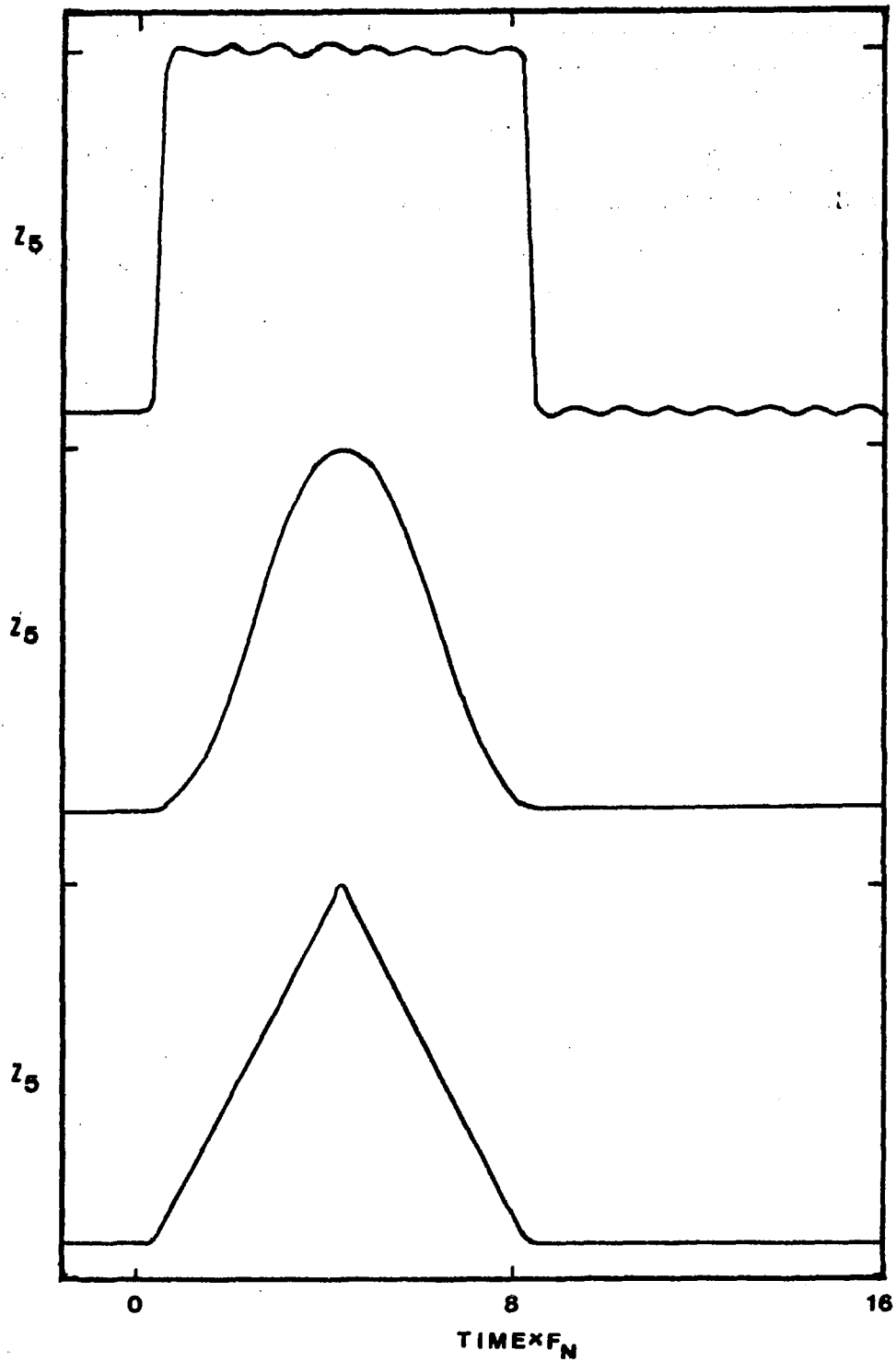
Fig. 15. Deconvolution of three sample pulses, z_5 sequence as in Figure 12.
