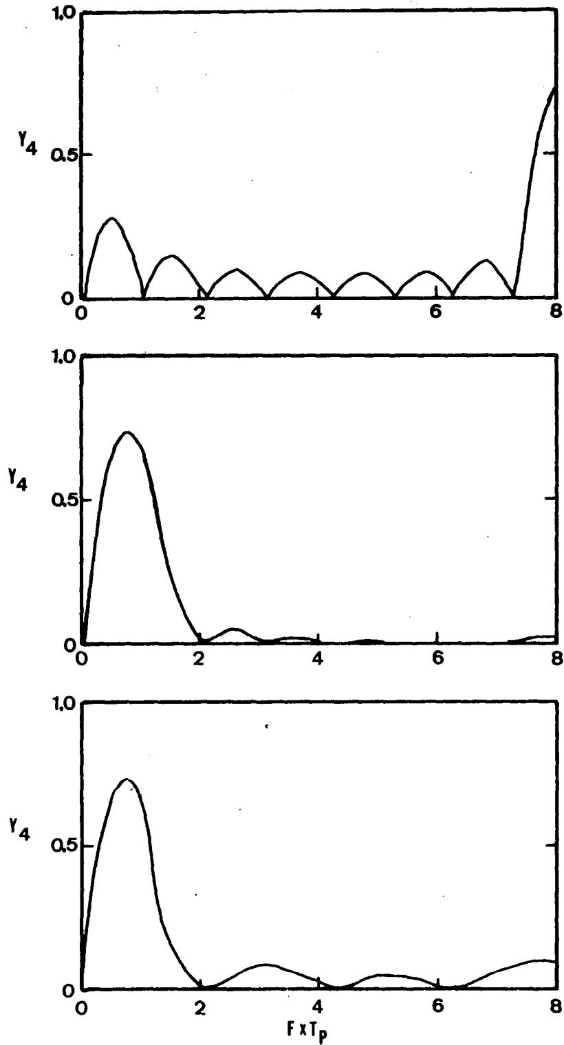
Fig. 14. Fourier spectrum of three sample output pulses, sequence as in Fig. 13.
