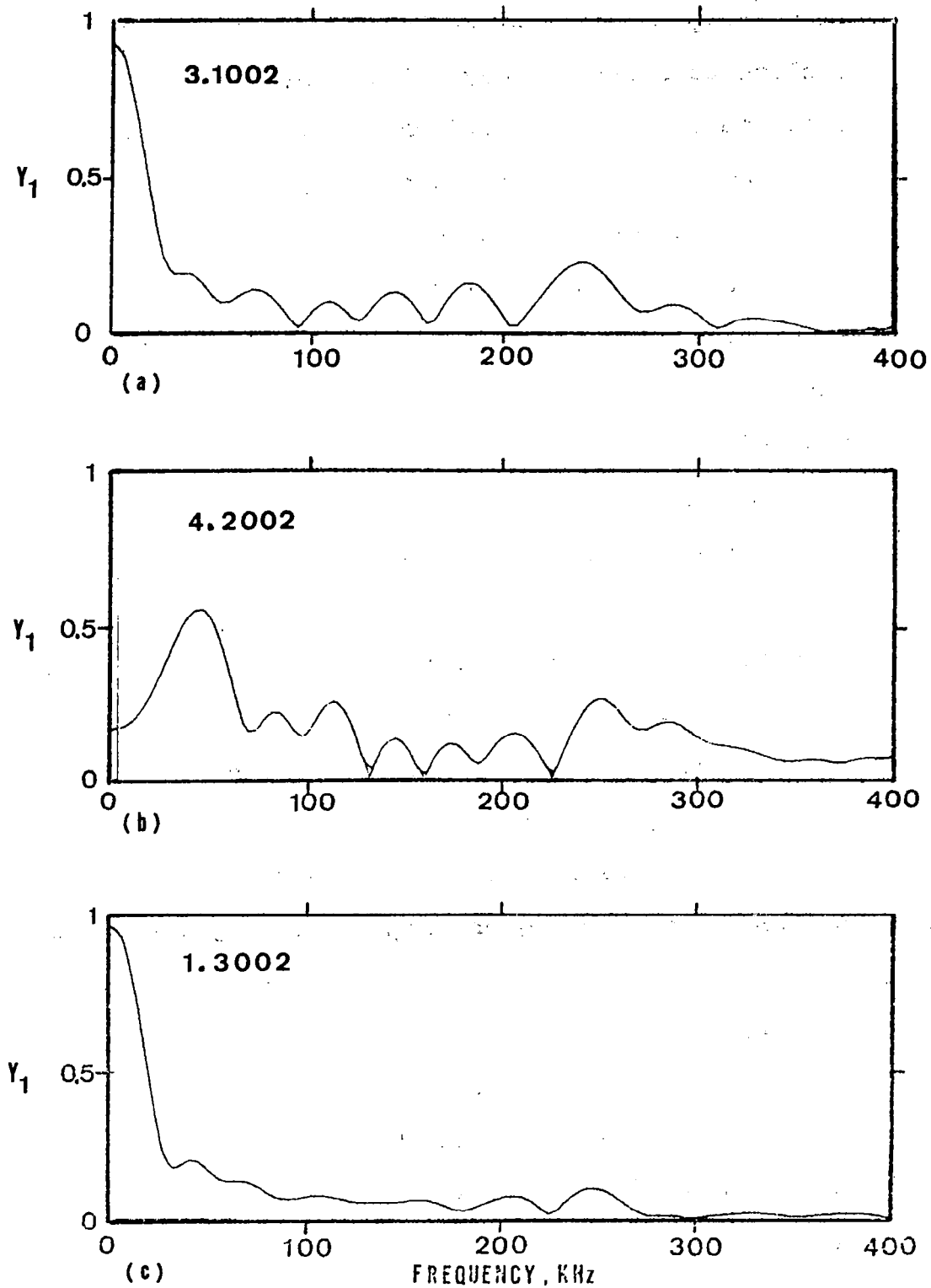
Fig. 58. Frequency spectrum of the pulse deconvolutions shown in Figure 57.
