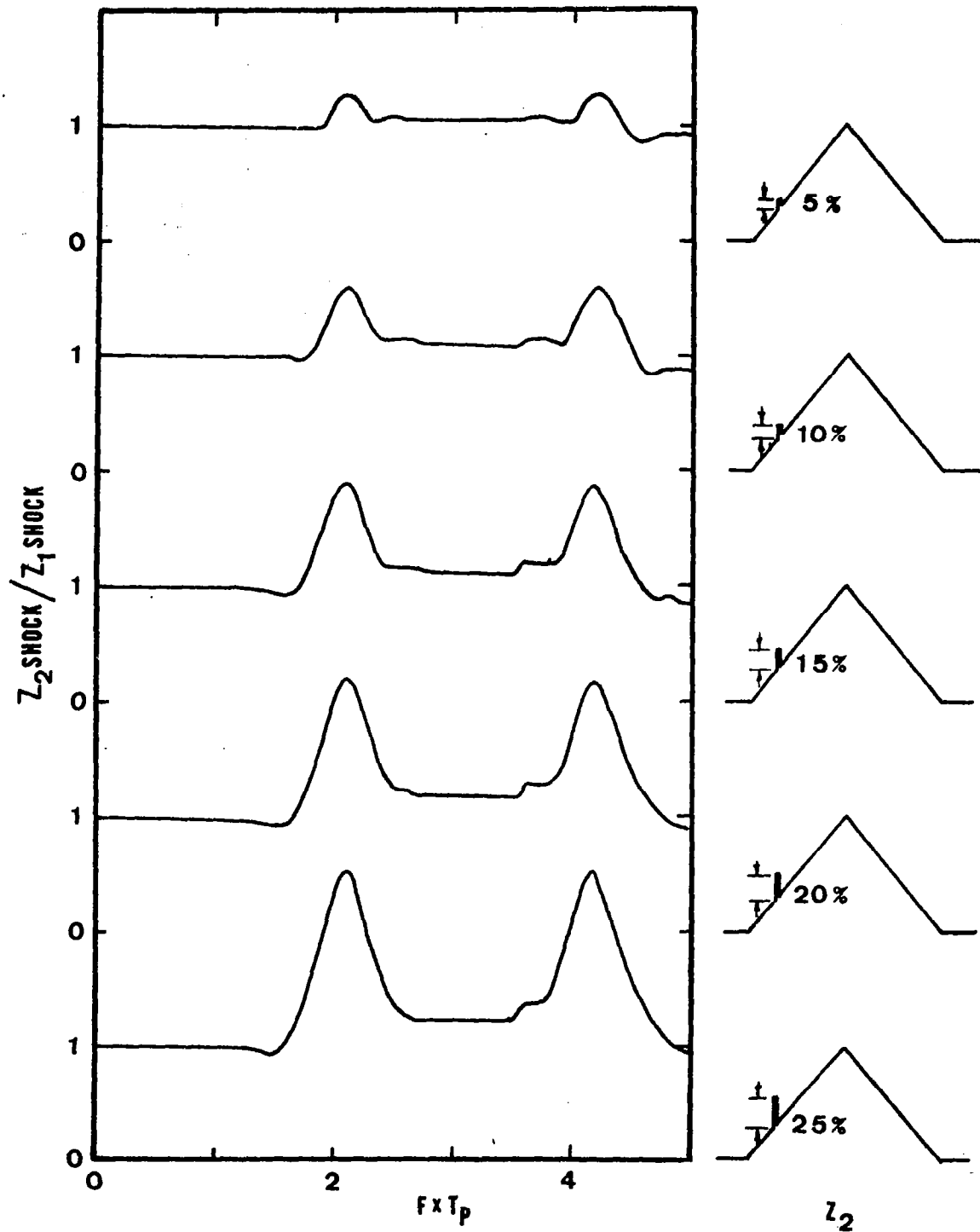
Fig. 10. Shock spectrum ratio plots for perturbation of different height located at 0.125 T_p .
