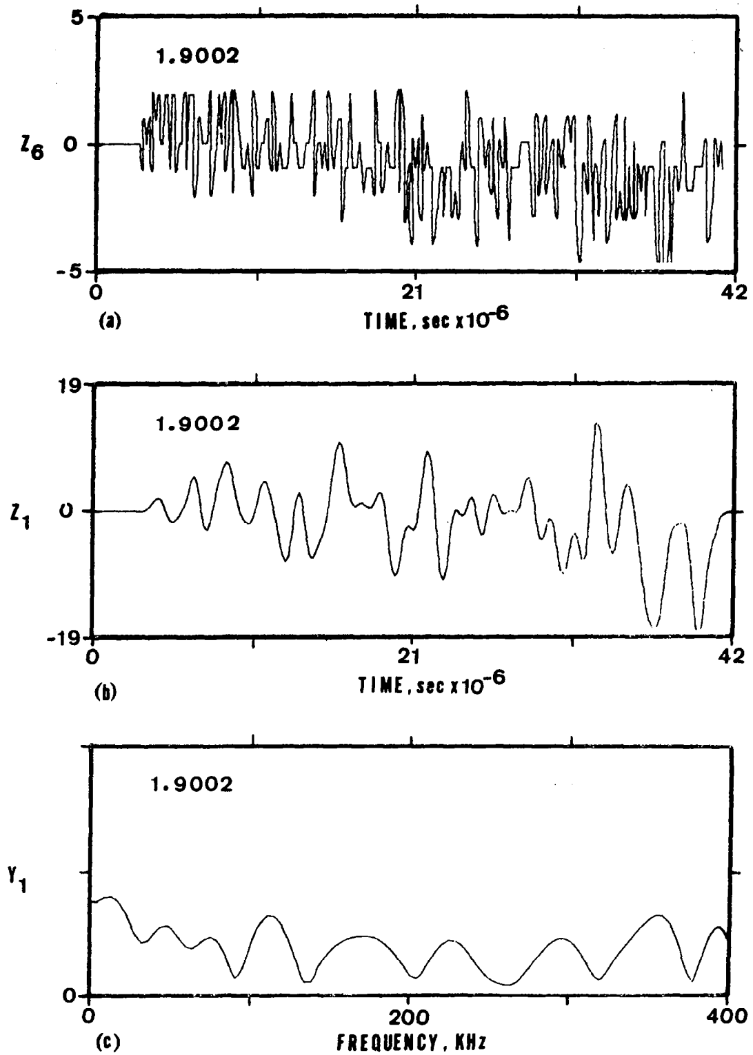
Fig. 60. Background signal with the bearing stationary.
