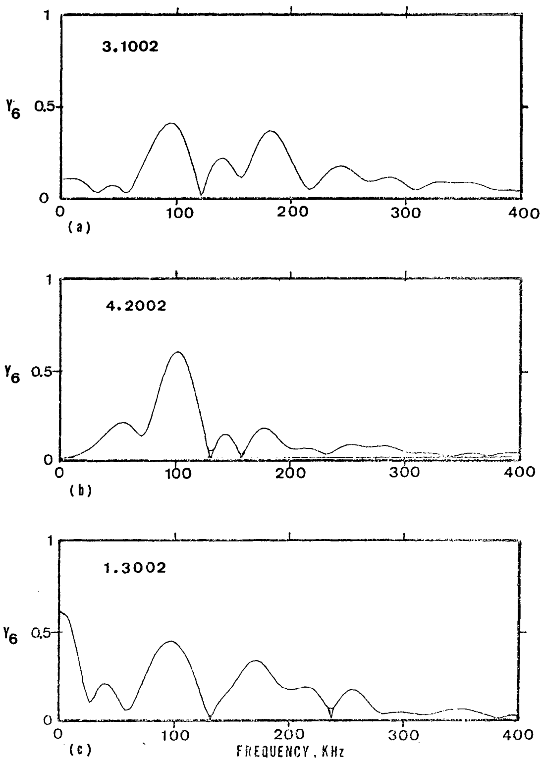
Fig. 56. Frequency spectrum of pulses shown in Figure 55.
