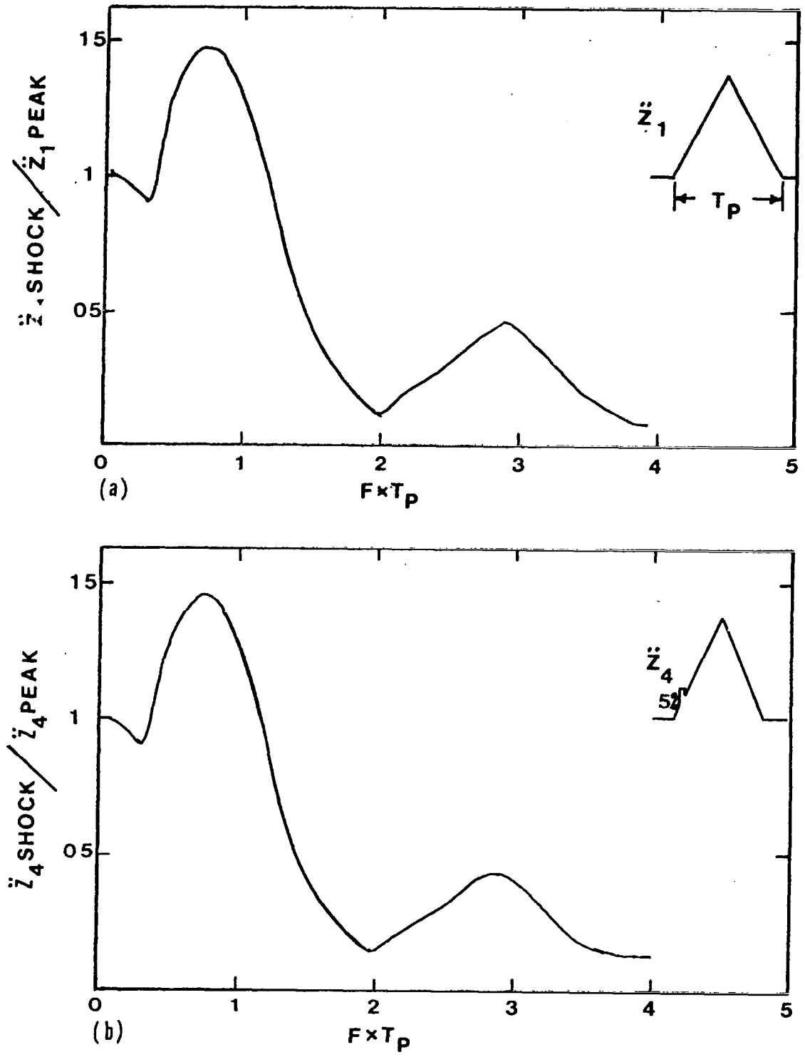
Fig. 7. Shock spectrum of relative motion for triangular pulse and triangular pulse with a 5% perturbation (damping ratio = 0.0001).
