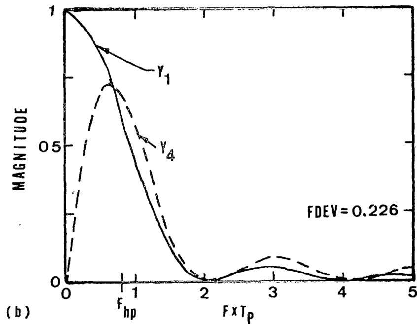
Fig. 21. Triangular pulse: \zeta = 0.01 ; F_{hp}/F_n = 0.1 ; T_p F_n = 8.0 . a) time domain; b) frequency domain.
