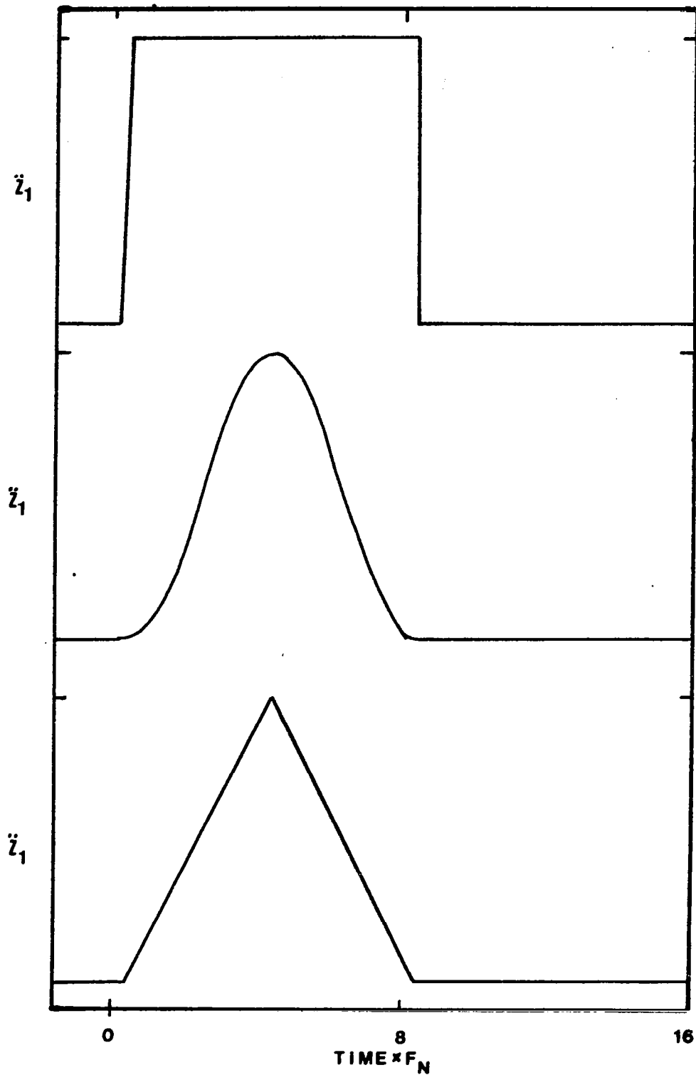
Fig. 12. Three sample acceleration pulses input at the transducer base, \ddot{z}_1 vs Time \times F_N .
