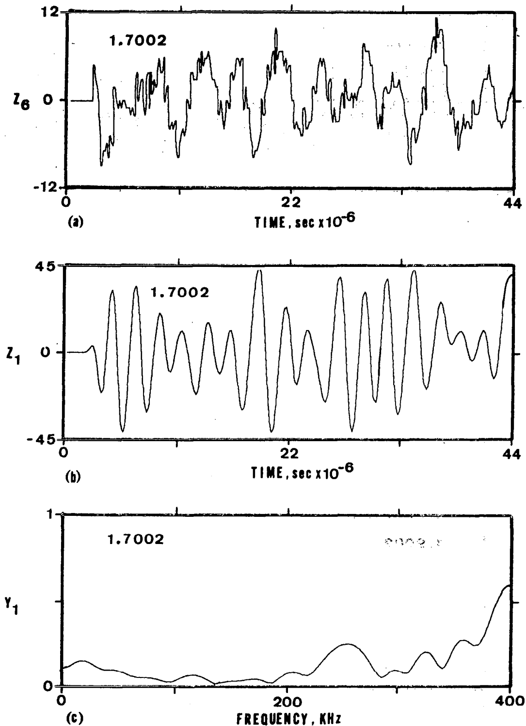
Fig. 61. Acoustic emission from a clean well lubricated bearing running with a 700 lb load.
