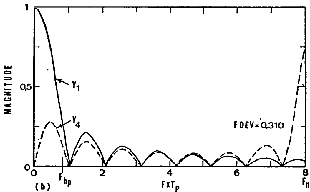
Fig. 20. Square pulse: \zeta = 0.01 ; F_{hp}/F_n = 0.1 ; T_p F_n = 8.0 . a) time domain; b) frequency spectrum.
