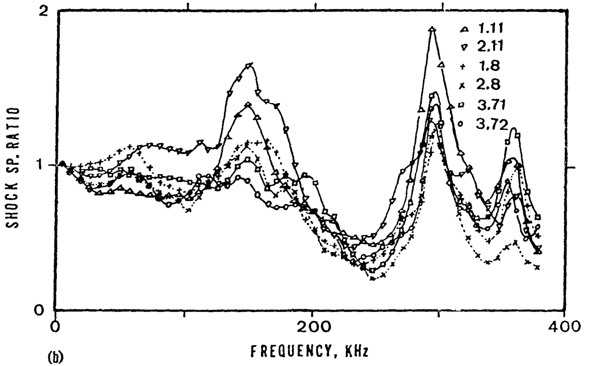
Fig. 73. Bearing tests: superimposed shock spectrum a) as-received traces, b) deconvoluted traces.
