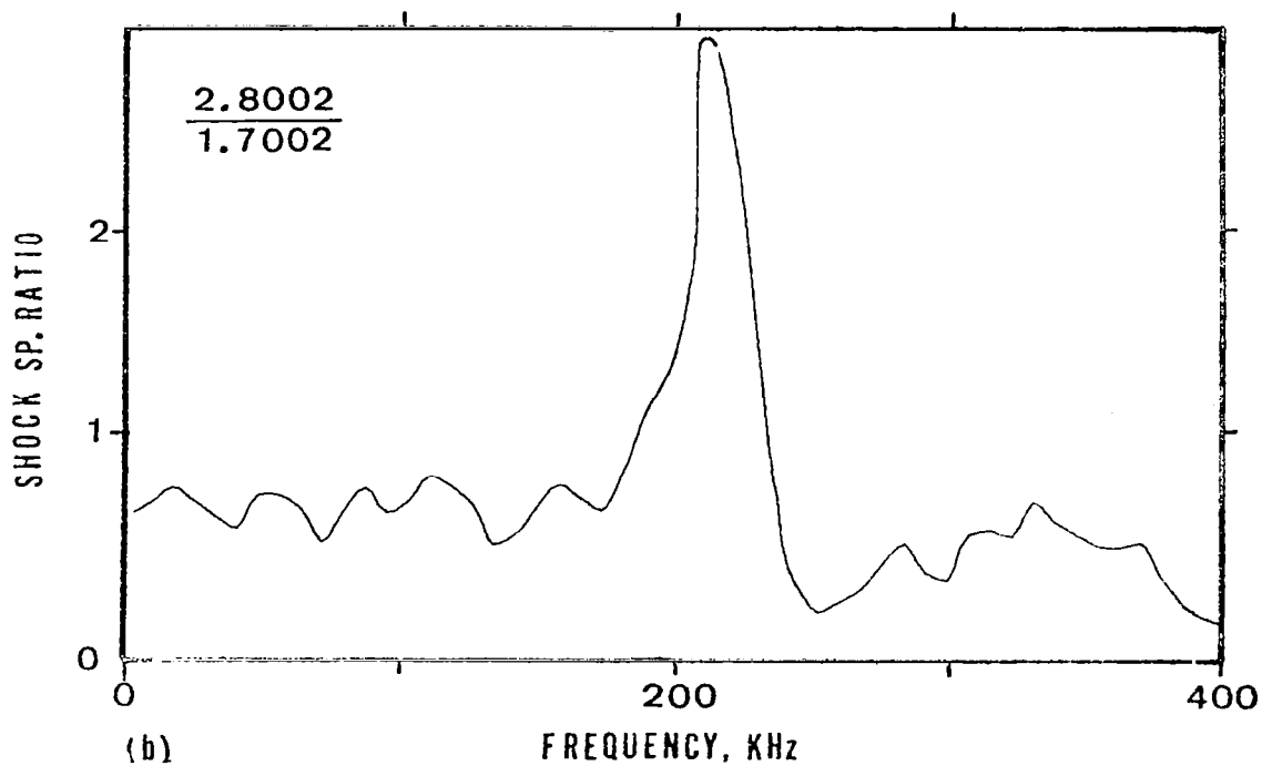
Fig. 71. Shock spectrum ratio of as-received traces of a bearing with a cut in the race relative to the trace in Figure 61(a).
