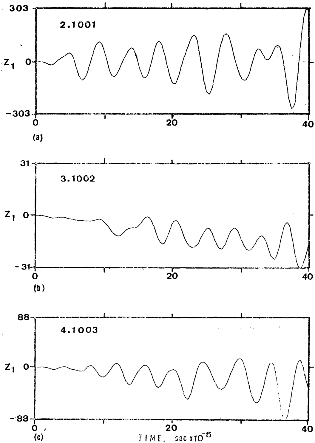
Fig. 53. Deconvolution through the flat plate model for the pulse shown in Figure 51.
