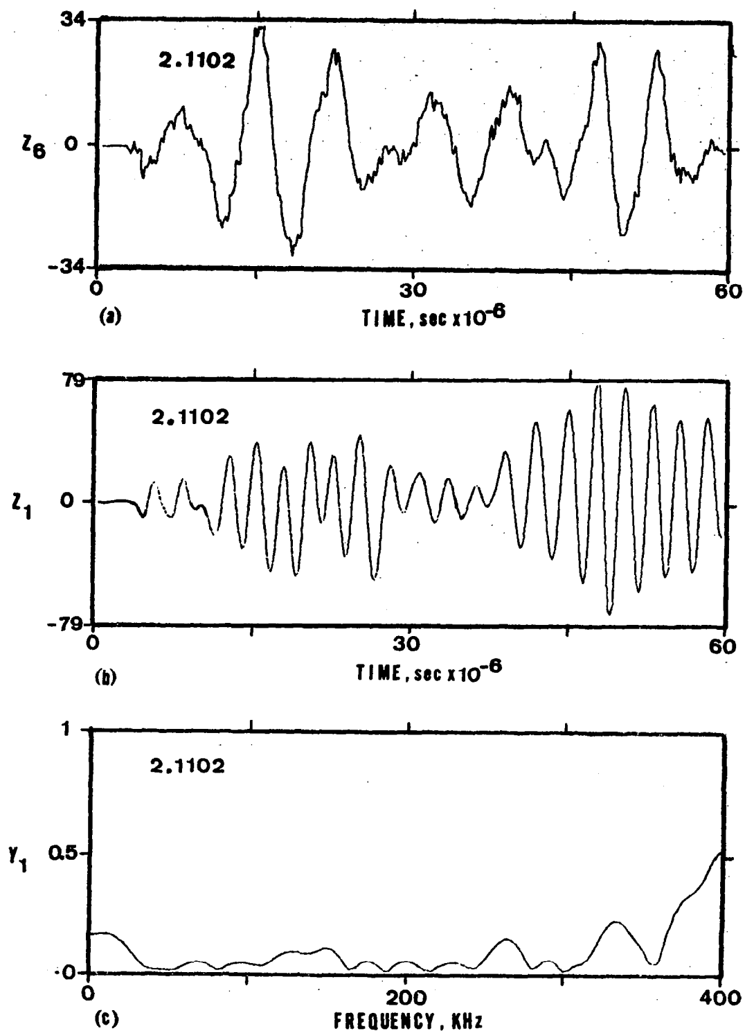
Fig. 67. Acoustic emission from a bearing with a cut in one ball; 700 lb thrust.
