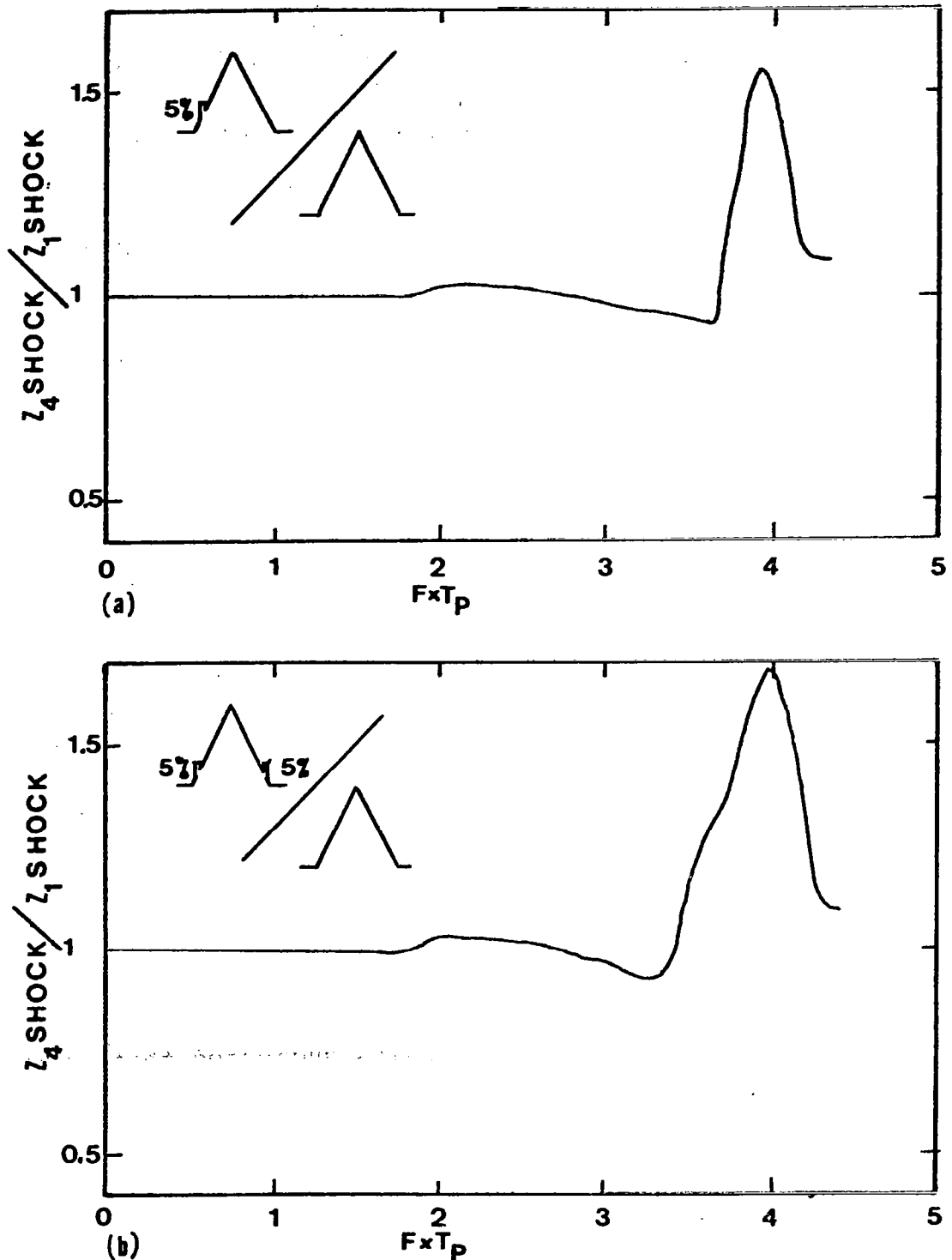
Fig. 8. Ratio of shock spectrums for two pulses relative to a simple pulse: a) 5% perturbation in leading edge of pulse and b) 5% perturbation on both edges of pulse.
