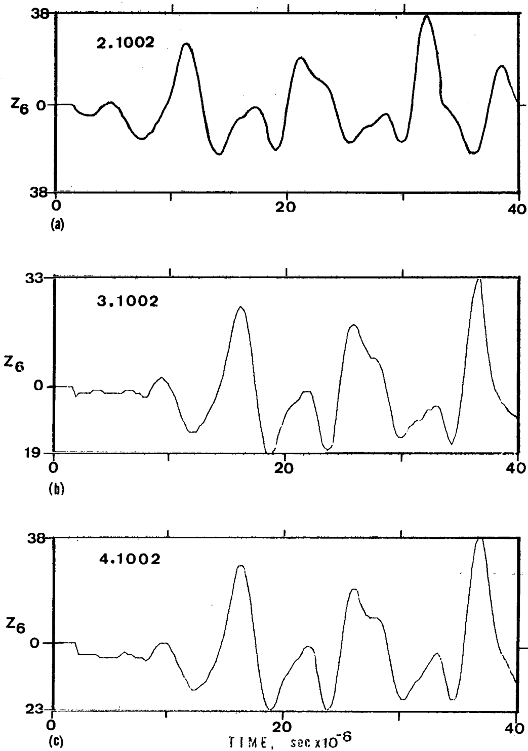
Fig. 45. As-received time domain trace for three spark discharges from the Dunegan/Endevco transducer.
