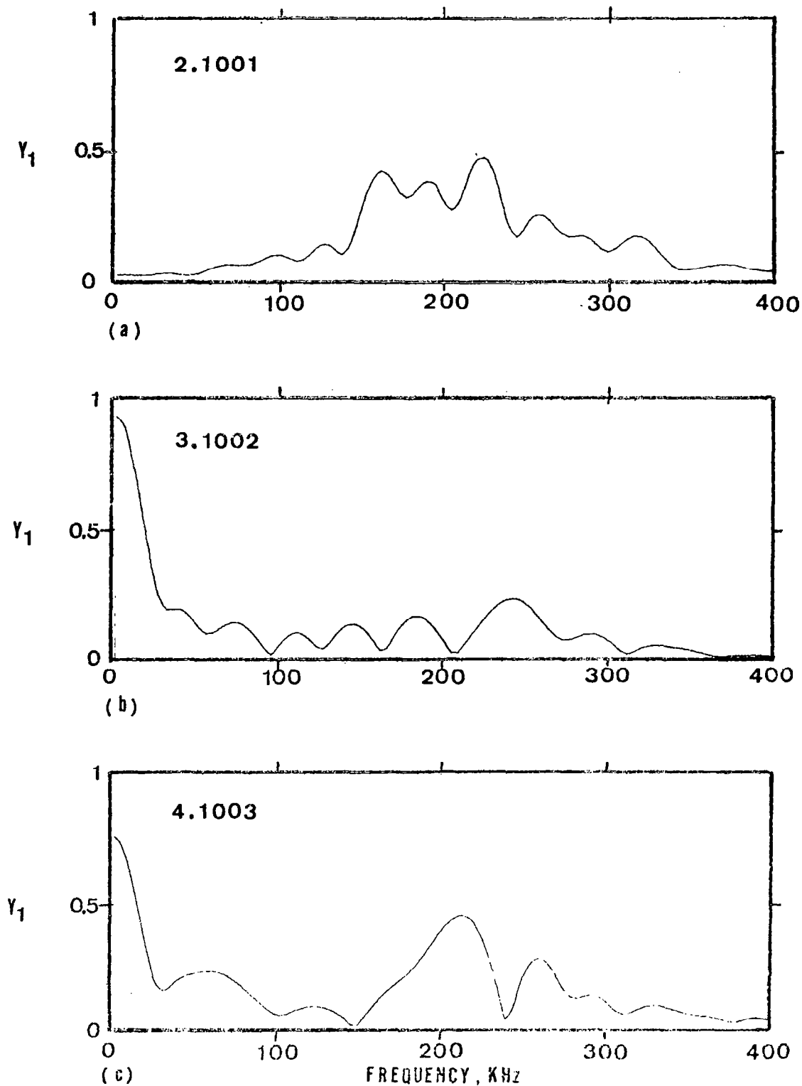
Fig. 54. Frequency spectrum of the pulse deconvolutions shown in Figure 53.
