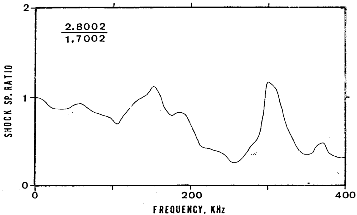
Fig. 69. Shock spectrum ratio of deconvoluted traces of a bearing with a cut in the race relative to the trace in Figure 61(b).
