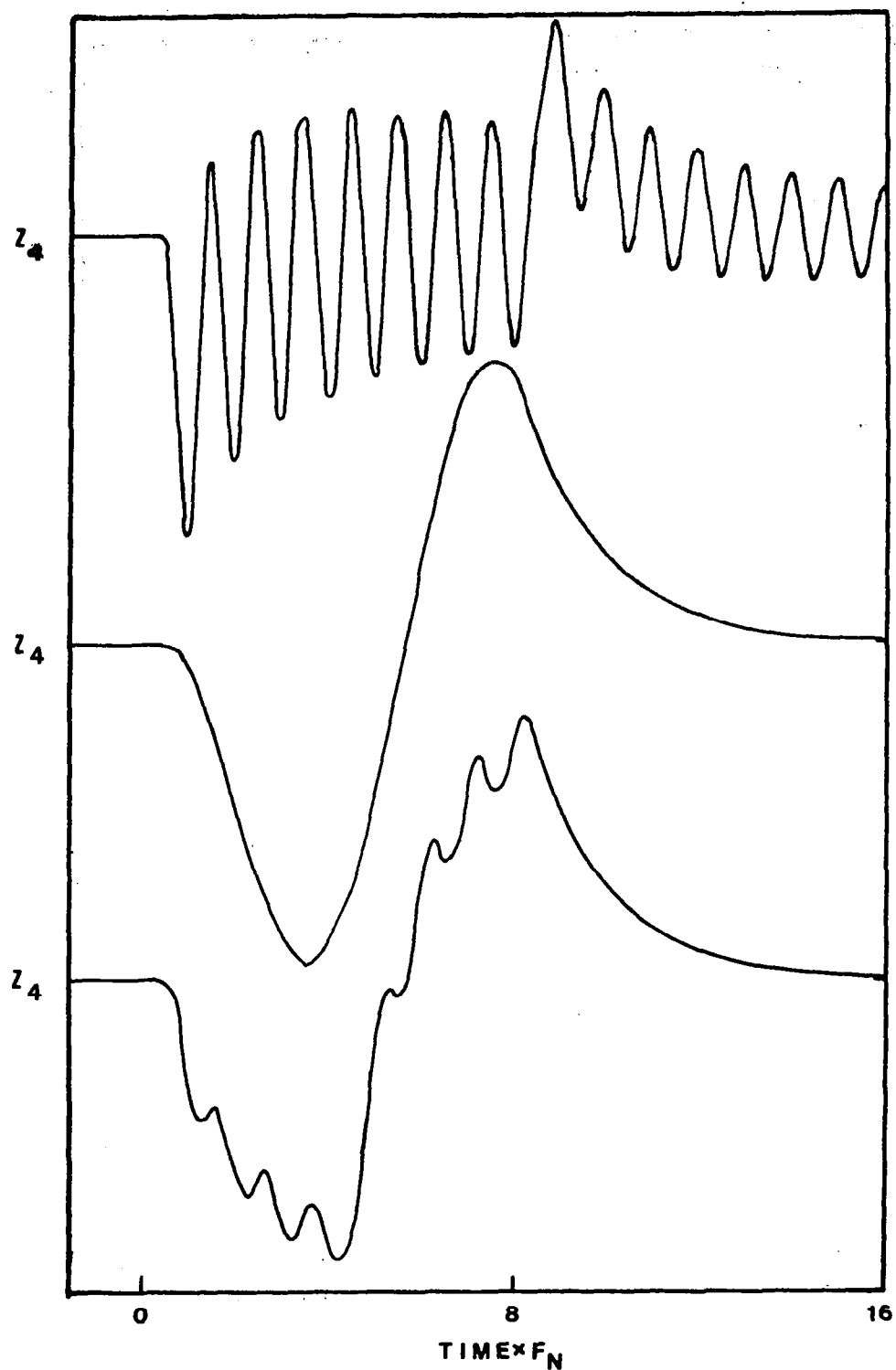
Fig. 13. Recorded output of three sample pulses, sequence as in Fig. 12, Z_4 vs Time \times F_n .
