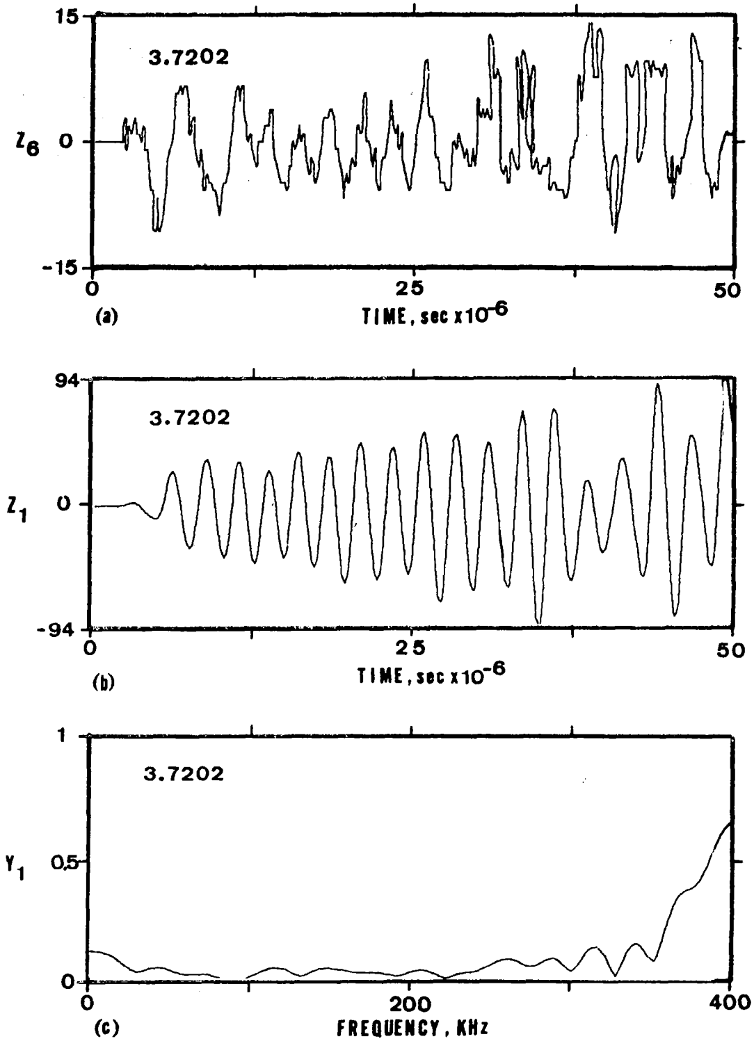
Fig. 63. Acoustic emission from a clean well lubricated bearing with a 700 lb thrust.
