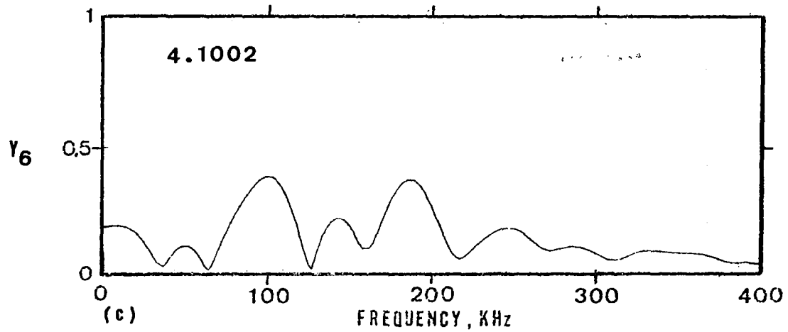
Fig. 46 Frequency spectrum of pulses shown in Figure 45.
