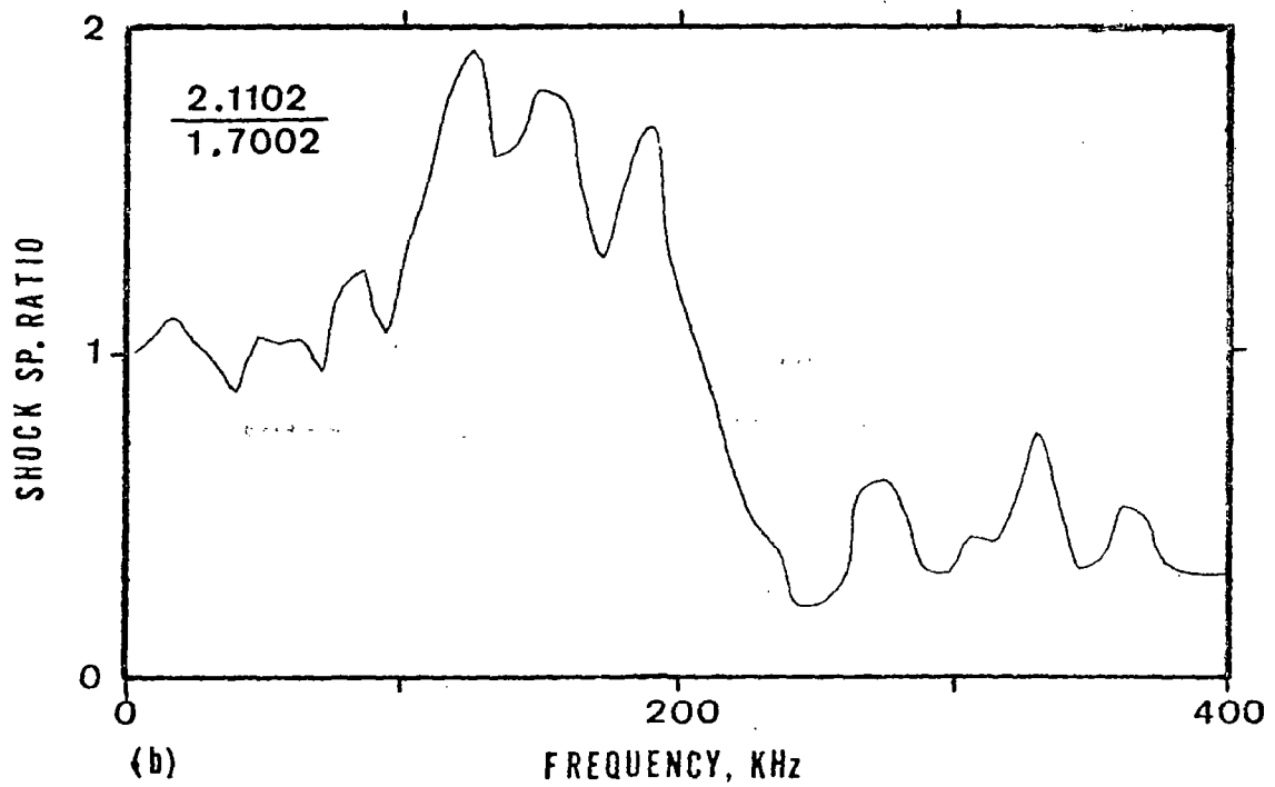
Fig. 72. Shock spectrum ratio of as-received traces of a bearing with a cut in one ball relative to the trace in Figure 61(a).
