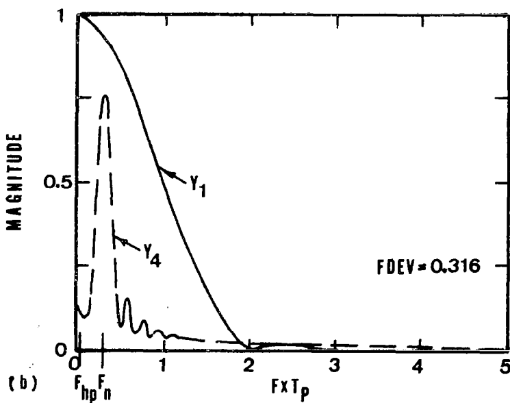
Fig. 19. Cosine pulse: \zeta = 0.01 ; F_{hp}/F_n = 0.1 ; T_p F_n = 0.3 . a) time domain; b) frequency domain.
