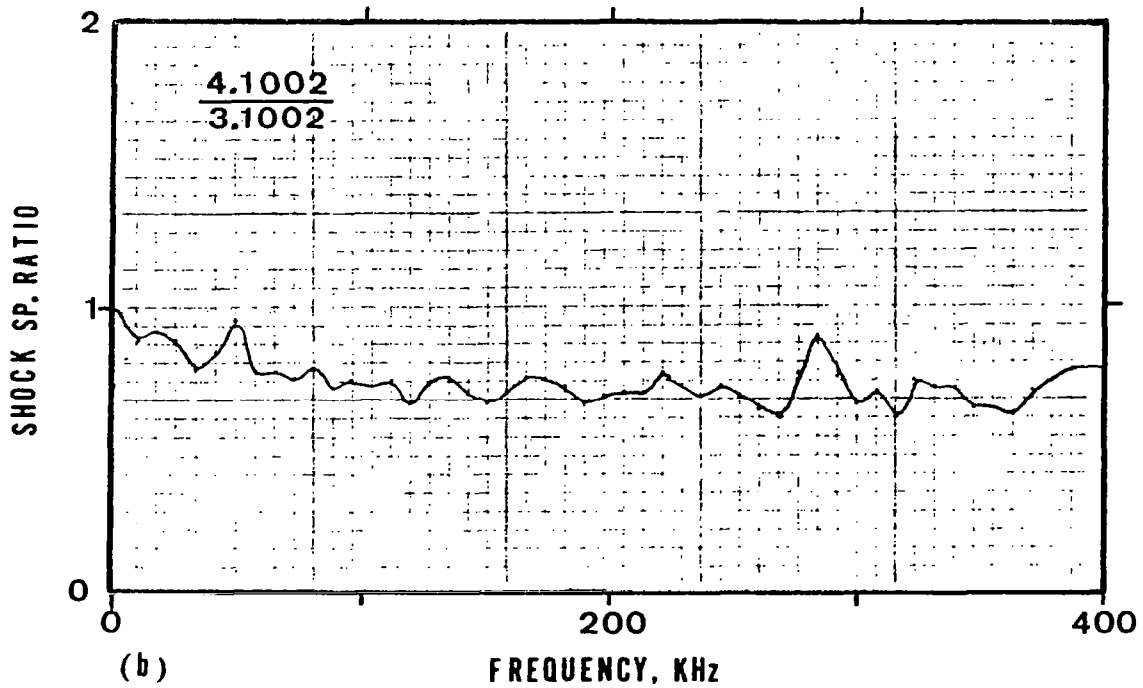
Fig. 49. Shock spectrum ratio of similar deconvolution pulses shown in Fig. 47.
