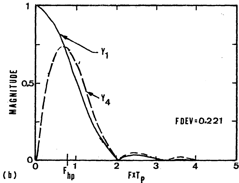
Fig. 22. Cosine pulse: \zeta = 0.01 ; F_{hp}/F_n = 0.1 ; T_p F_n = 8.0 . a) time domain; b) frequency domain.
