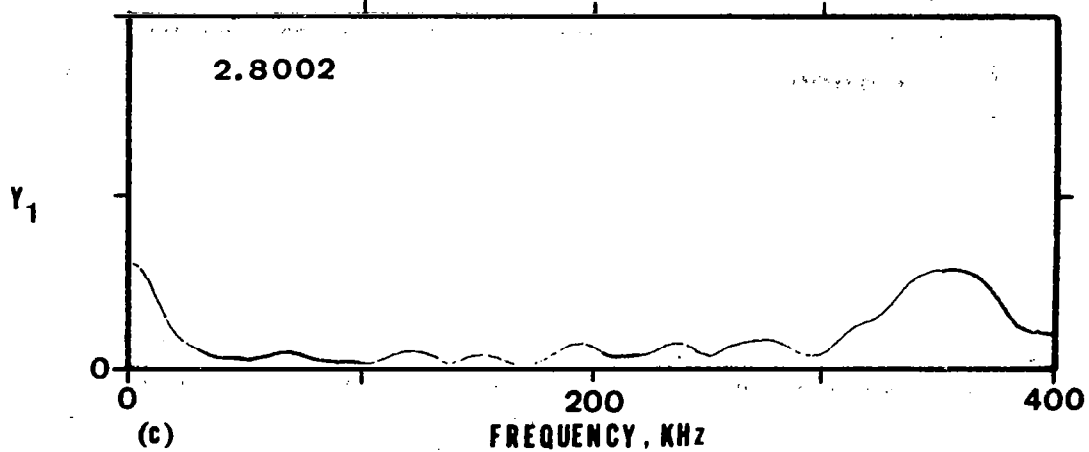
Fig. 65. Acoustic emission from a bearing with a cut in the race; 700 lb thrust.
