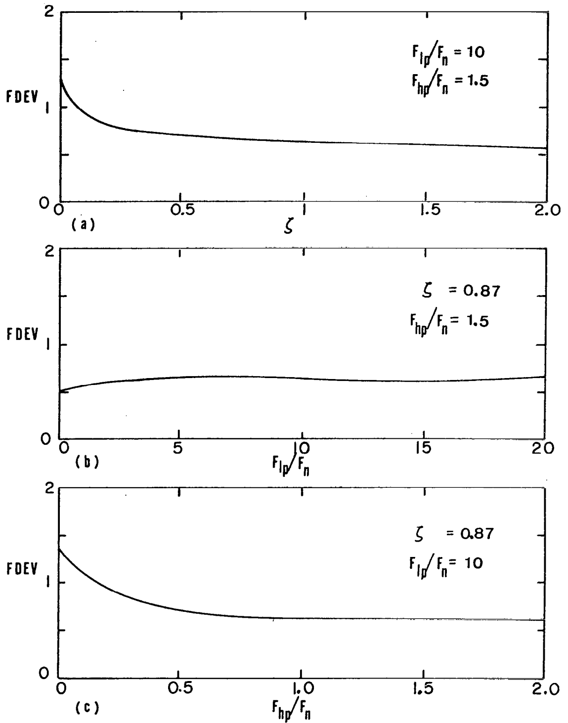
Fig. 23. Frequency domain objective function field for a square pulse: T_p F_n = 0.3 .
