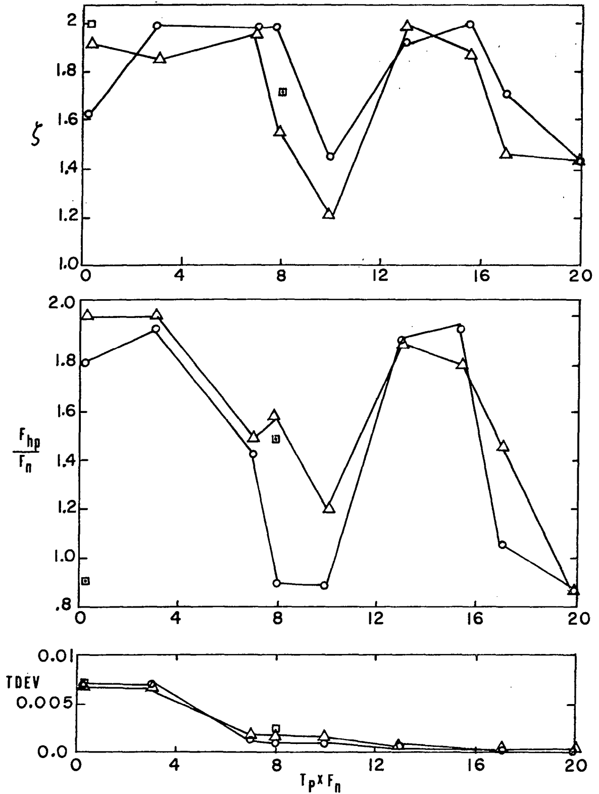
Fig. 25. Summary of optimal designs for triangular ( \Delta ), square ( \square ) and cosine ( o ) pulses of various lengths.
