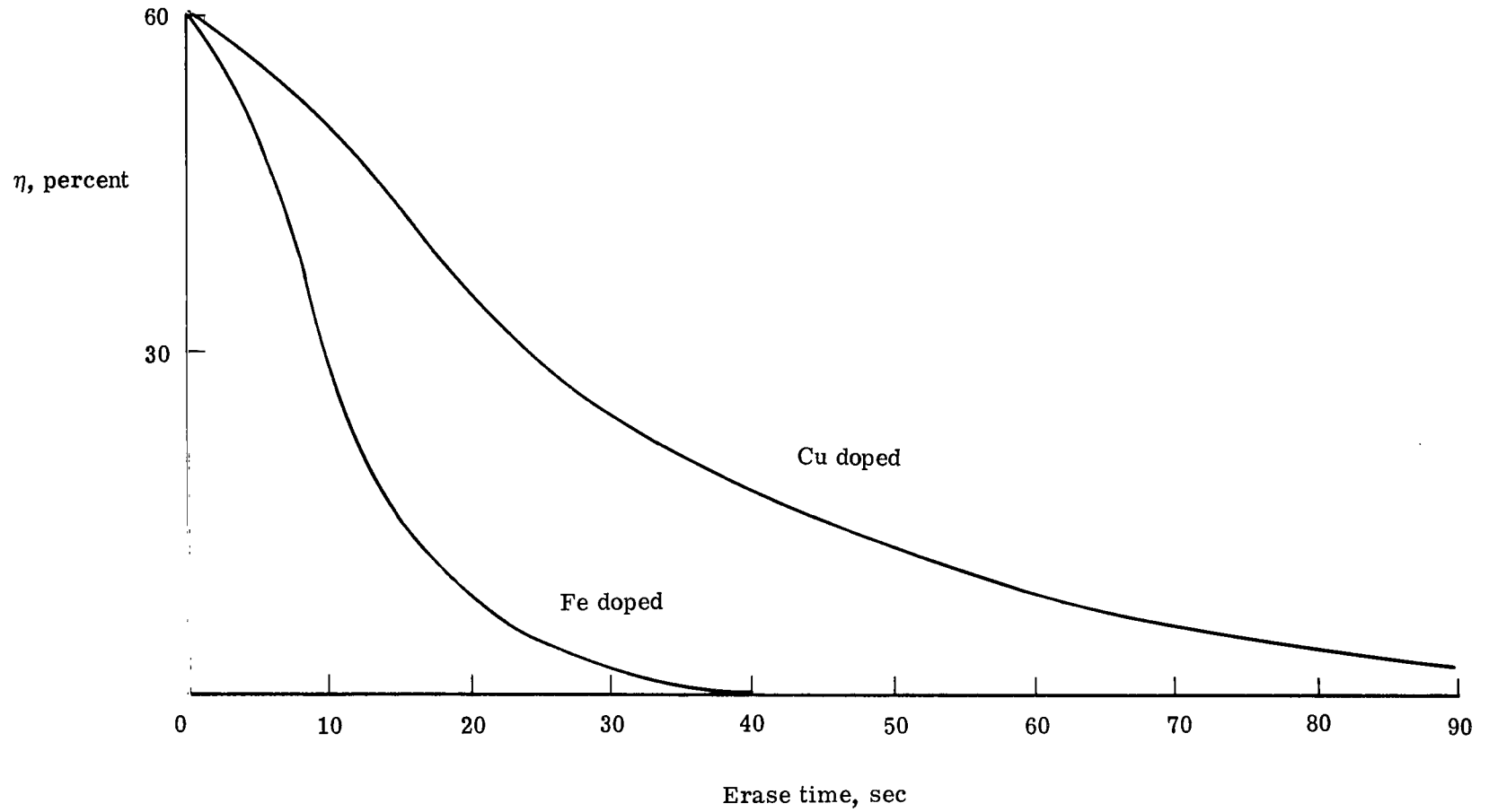
Figure 6.- Erase characteristics of doped LiNbO 3 . Power density = 2.15 W/cm 2 ; \lambda = 514.5 nm.
