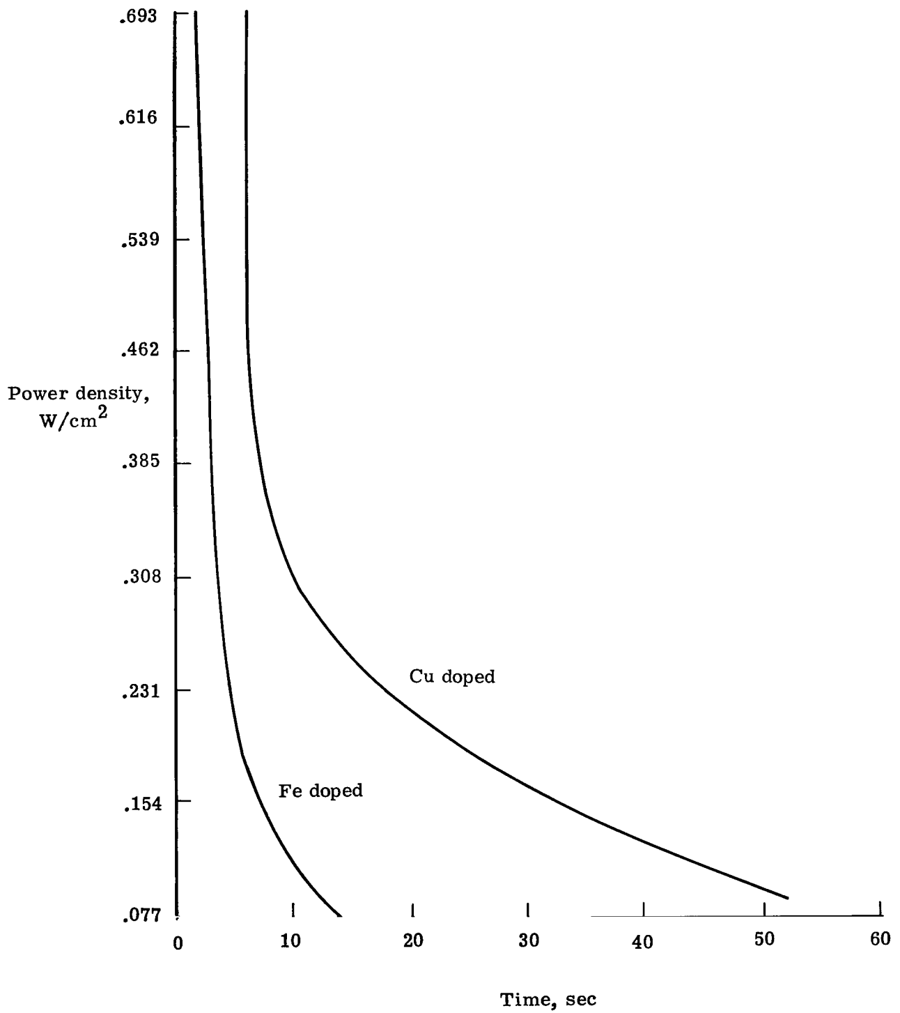
Figure 5.- Write power density plotted against time for 10 percent \eta in doped \text{LiNbO}_3 . Write \lambda = 488 \text{ nm} .
