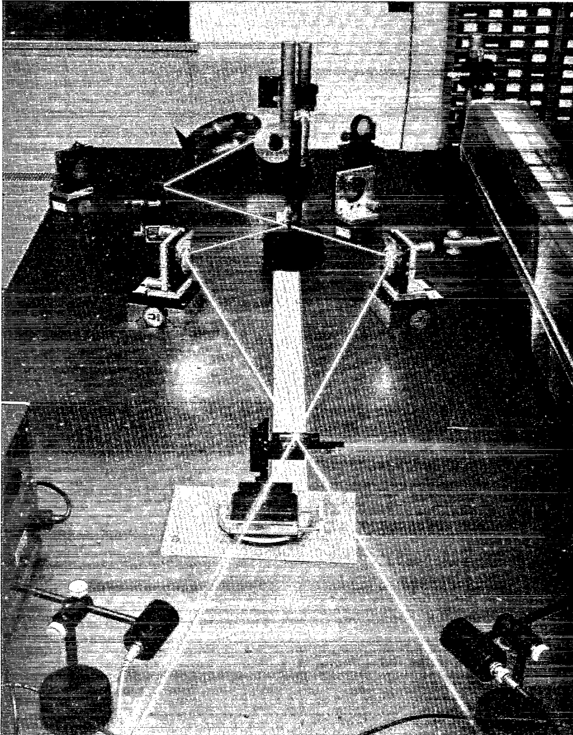
Figure 3.- Experimental setup.
