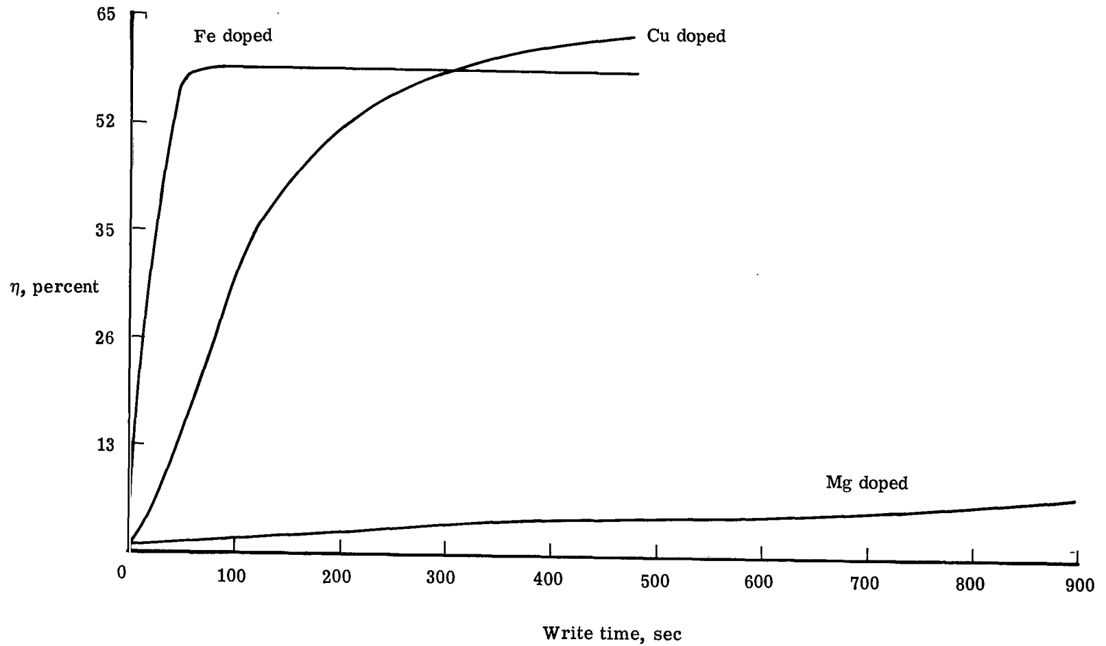
Figure 4.- Write characteristics of doped \text{LiNbO}_3 . Power density = 0.231 \text{ W/cm}^2 ; \lambda = 488 \text{ nm} .
