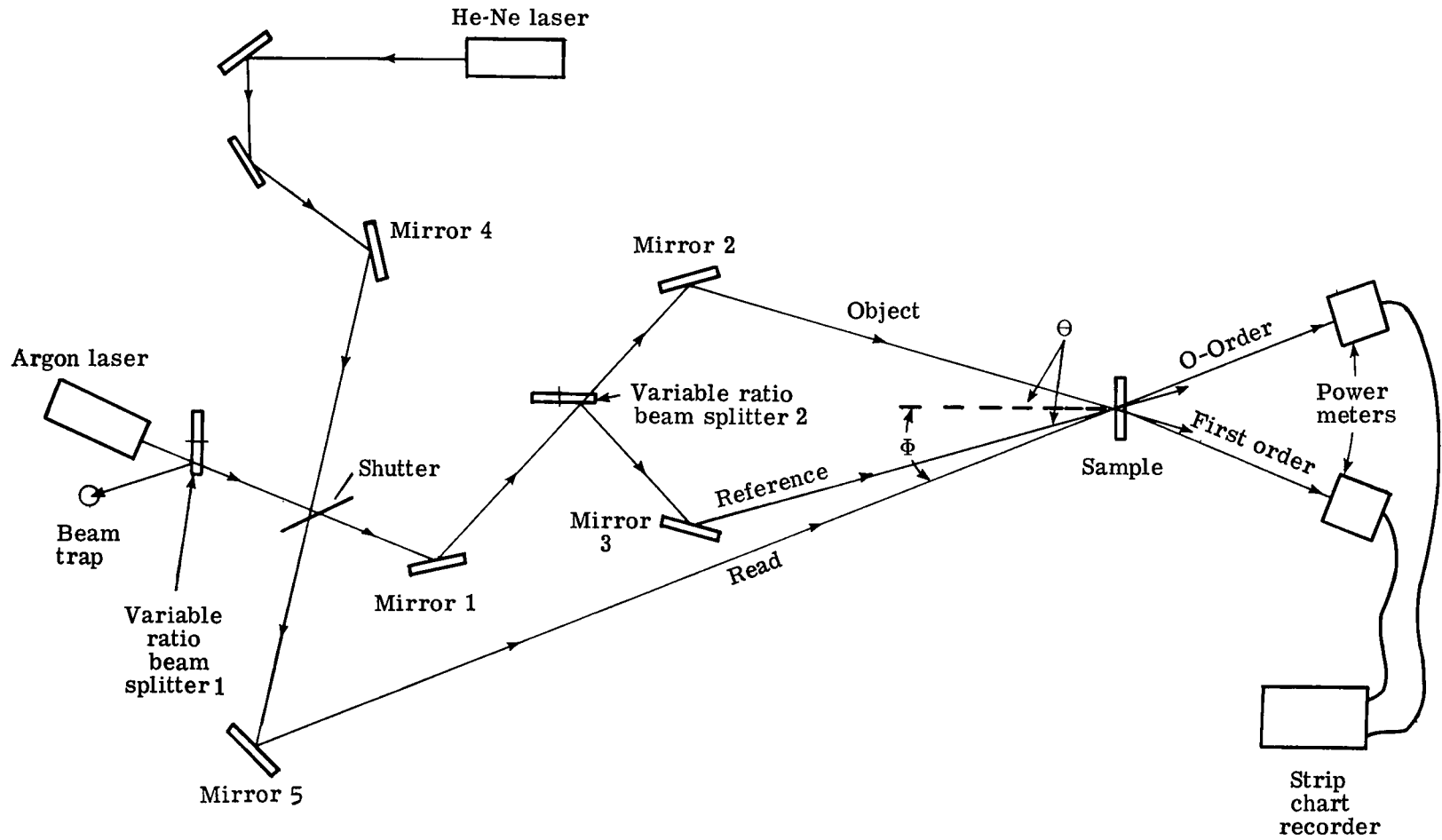
Figure 2.- Optical arrangement.
