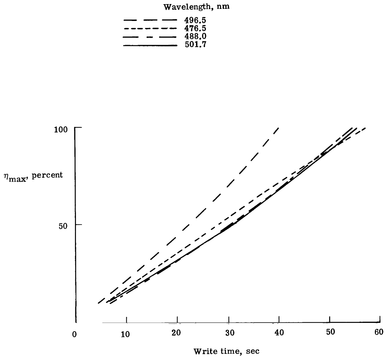
Figure 7.- Results of variable write wavelengths in Fe-doped LiNbO 3 . Power density = 0.231 W/cm 2 .
