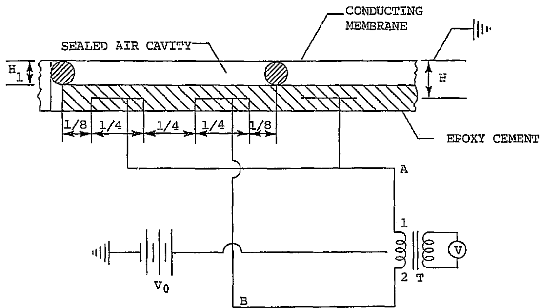
(a) Electrical hookup
